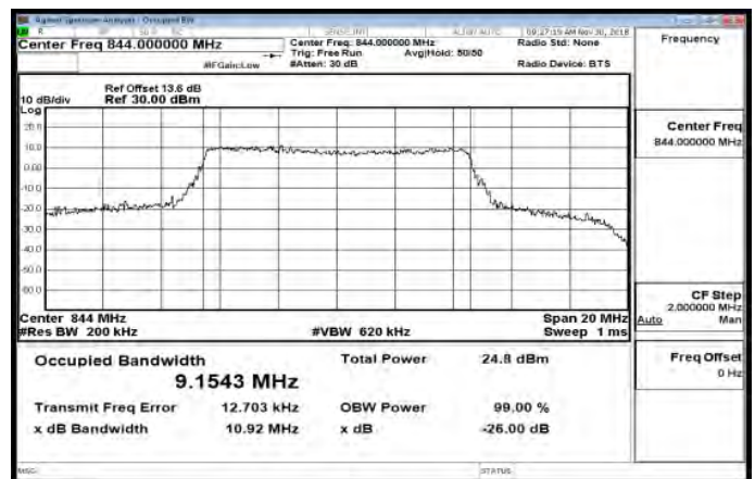
Band5_10MHz_64QAM_50_0_HighCH20600-844
