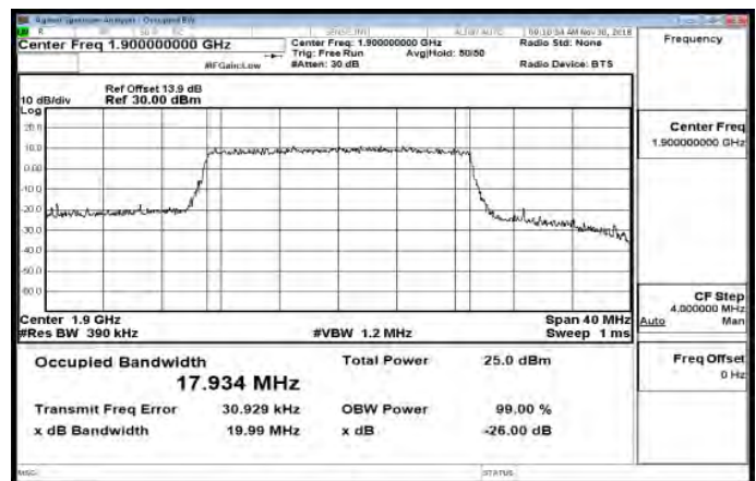
Band2_20MHz_64QAM_100_0_HighCH19100-1900
