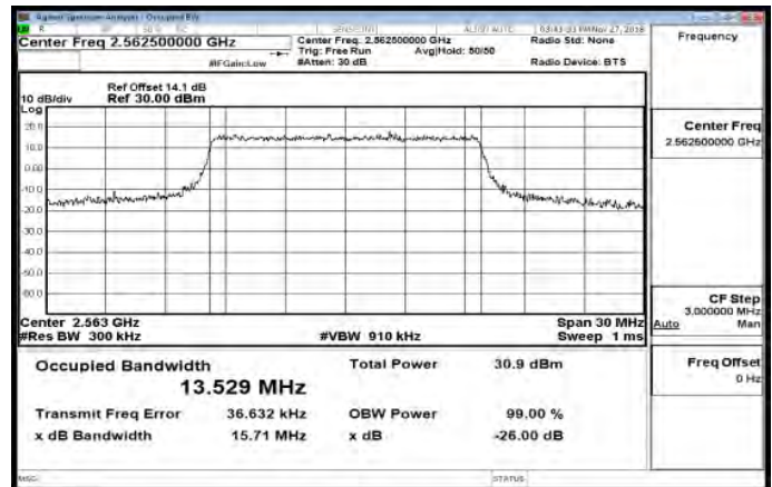
Band7_15MHz_16QAM_75_0_HighCH21375-2562.5
