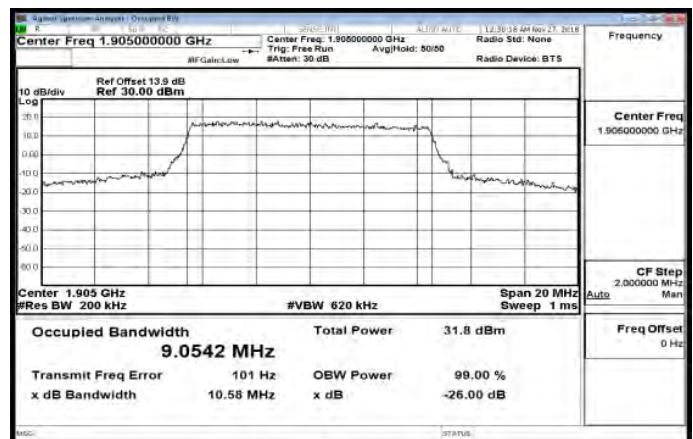
Band2_10MHz_QPSK_50_0_HighCH19150-1905
