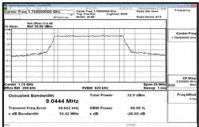
Band4_10MHz_QPSK_50_0_HighCH20350-1750
