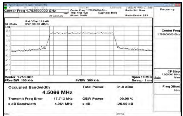
Band4_5MHz_16QAM_25_0_HighCH20375-1752.5
