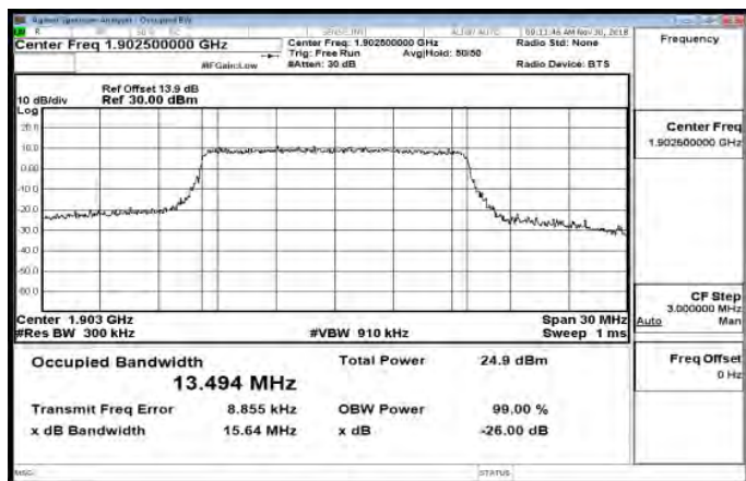
Band2_15MHz_64QAM_75_0_HighCH19125-1902.5
