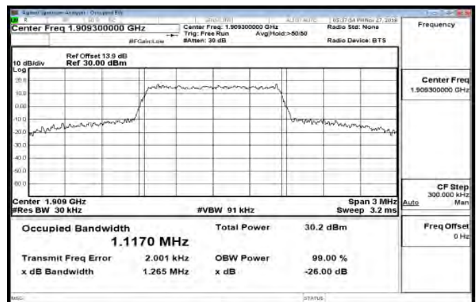
Band2_1_4MHz_16QAM_6_0_HighCH19193-1909.3
