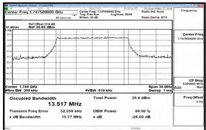
Band4_15MHz_16QAM_75_0_HighCH20325-1747.5
