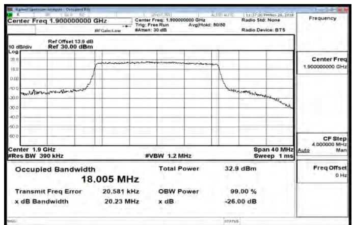
Band2_20MHz_QPSK_100_0_HighCH19100-1900
