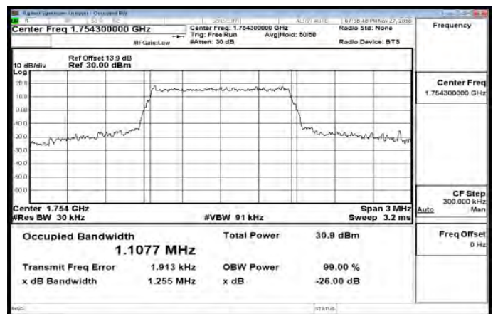
Band4_1_4MHz_16QAM_6_0_HighCH20393-1754.3
