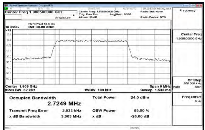
Band2_3MHz_64QAM_15_0_HighCH19185-1908.5
