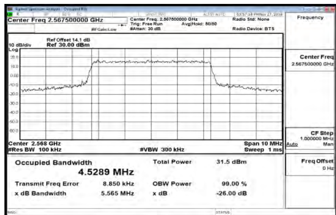
Band7_5MHz_QPSK_25_0_HighCH21425-2567.5
