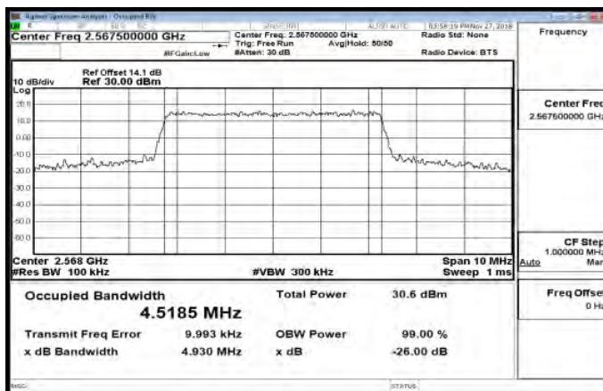
Band7_5MHz_16QAM_25_0_HighCH21425-2567.5
