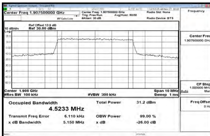
Band2_5MHz_16QAM_25_0_HighCH19175-1907.5
