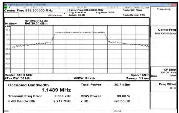
Band5_1_4MHz_16QAM_6_0_HighCH20643-848.3
