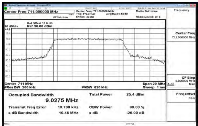
Band17_10MHz_64QAM_50_0_HighCH23800-711
