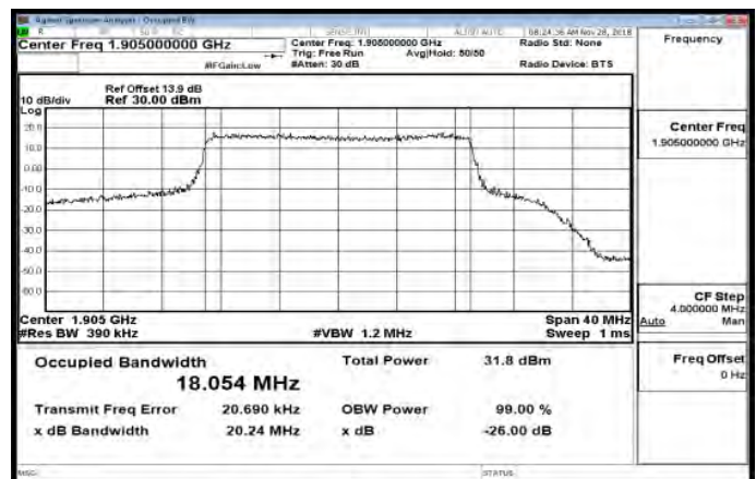
Band25_20MHz_QPSK_100_0_HighCH26590-1905
