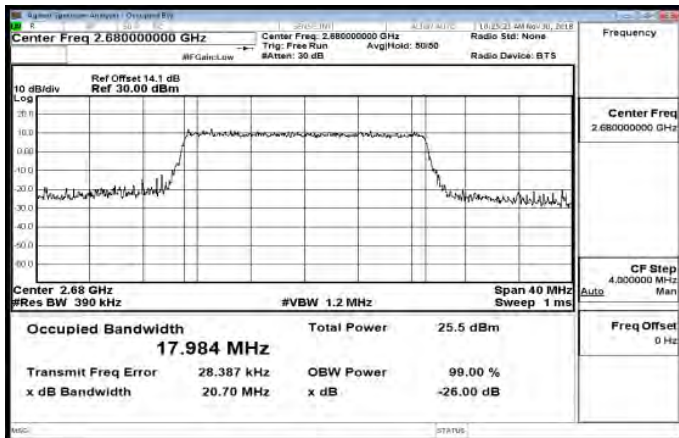
Band41_20MHz_64QAM_100_0_HighCH41490-2680
