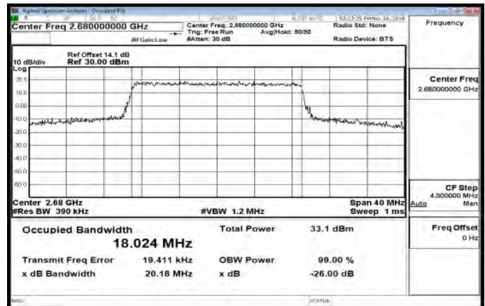
Band41_20MHz_16QAM_100_0_HighCH41490-2680
