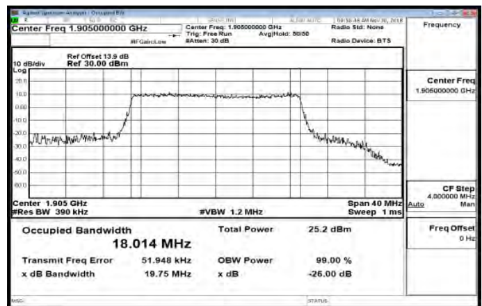
Band25_20MHz_64QAM_100_0_HighCH26590-1905
