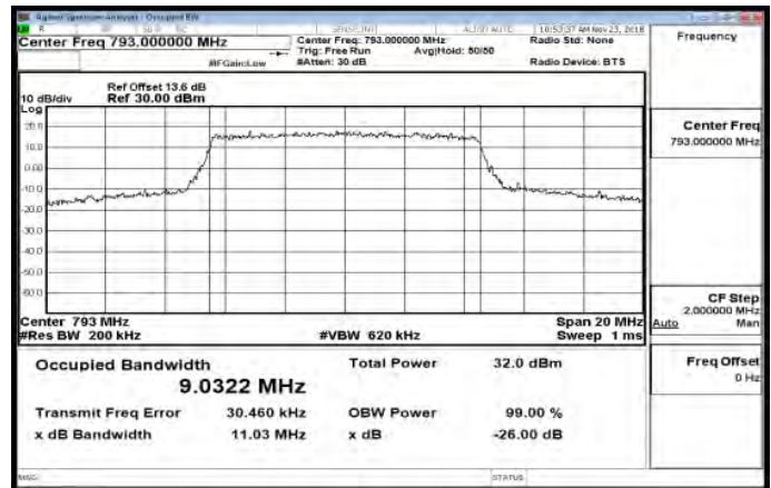
Band14_10MHz_16QAM_50_0_MidCH23330
