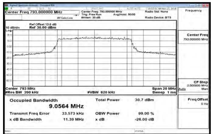
Band14_10MHz_64QAM_50_0_MidCH23330
