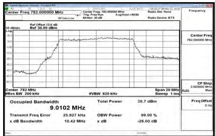
Band13_10MHz_64QAM_50_0_MidCH23230-782
