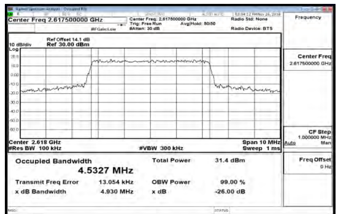
Band38_5MHz_QPSK_25_0_HighCH38225-2617.5
