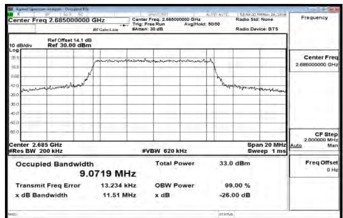
Band41_10MHz_16QAM_50_0_HighCH41540-2685
