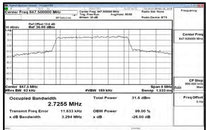
Band26_3MHz_QPSK_15_0_HighCH27025-847.5
