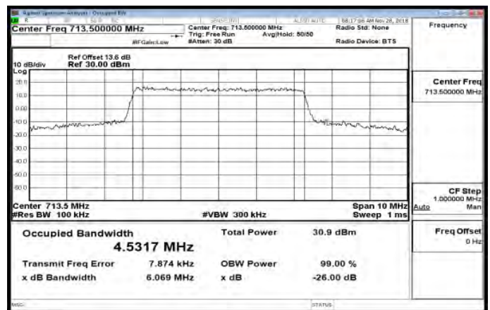
Band17_5MHz_16QAM_25_0_HighCH23825-713.5
