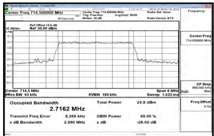
Band12_3MHz_64QAM_15_0_HighCH23165-714.5
