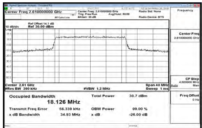
Band38_20MHz_16QAM_100_0_HighCH38150-2610
