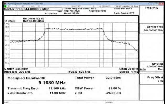
Band26_10MHz_QPSK_50_0_HighCH26990-844
