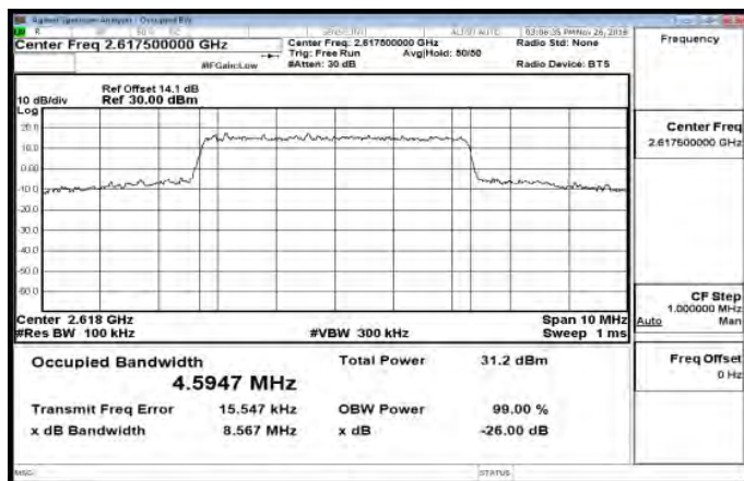
Band38_5MHz_16QAM_25_0_HighCH38225-2617.5
