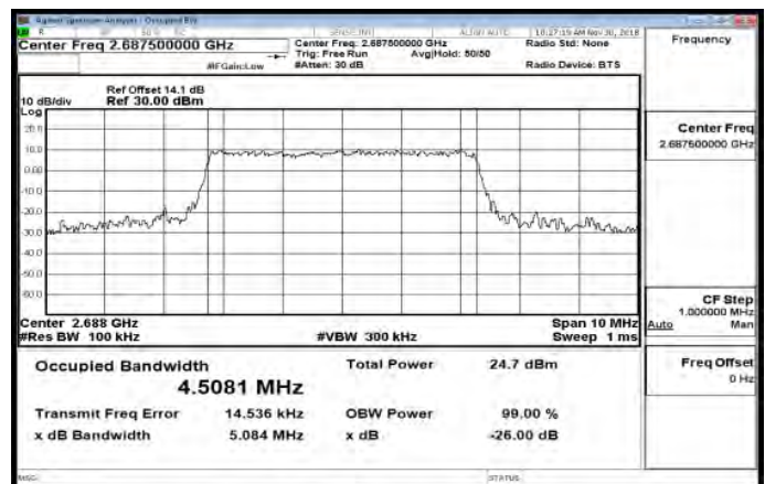
Band41_5MHz_64QAM_25_0_HighCH41565-2687.5
