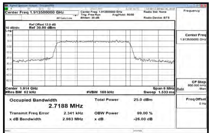
Band25_3MHz_64QAM_15_0_HighCH26675-1913.5
