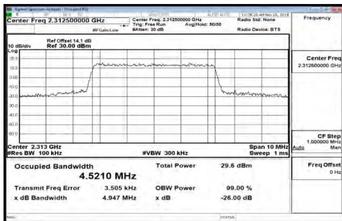
Band30_5MHz_16QAM_25_0_HighCH27735-2312.5
