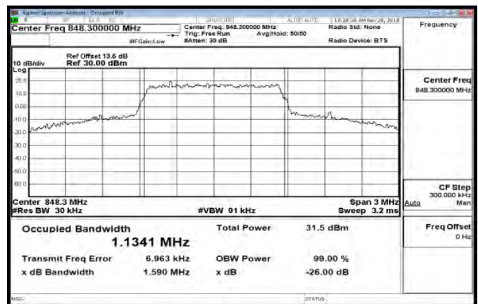
Band26_1_4MHz_16QAM_6_0_HighCH27033-848.3
