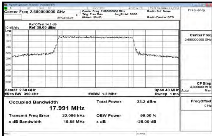
Band41_20MHz_QPSK_100_0_HighCH41490-2680
