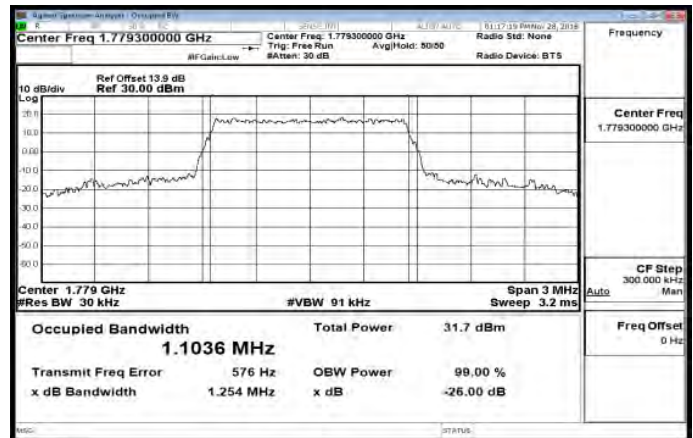
Band66_1_4MHz_QPSK_6_0_HighCH132665-1779.3
