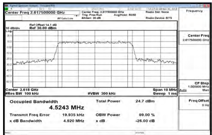
Band38_5MHz_64QAM_25_0_HighCH38225-2617.5
