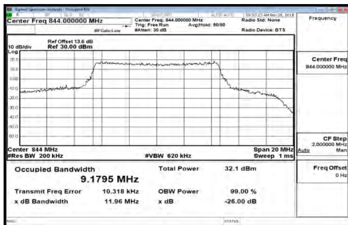
Band26_10MHz_16QAM_50_0_HighCH26990-844
