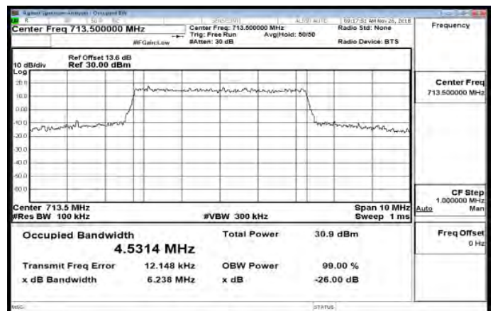
Band12_5MHz_16QAM_25_0_HighCH23155-713.5
