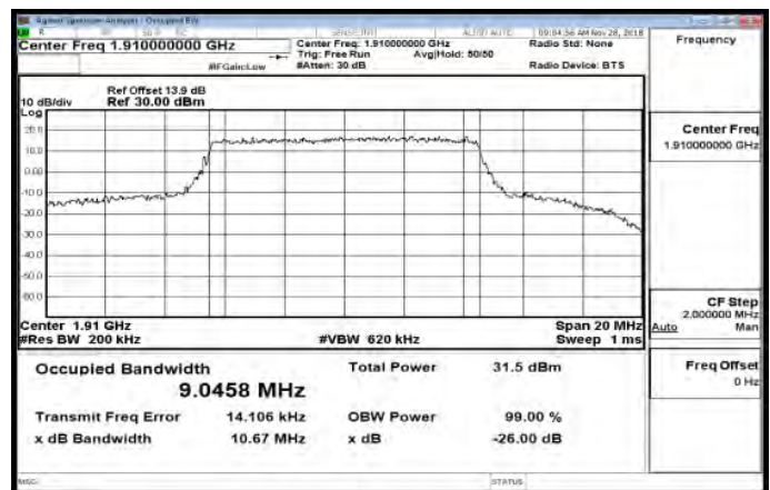
Band25_10MHz_QPSK_50_0_HighCH26640-1910
