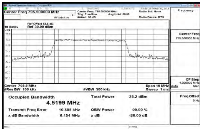
Band14_5MHz_64QAM_25_0_HighCH23355
