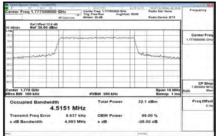
Band66_5MHz_QPSK_25_0_HighCH132647-1777.5
