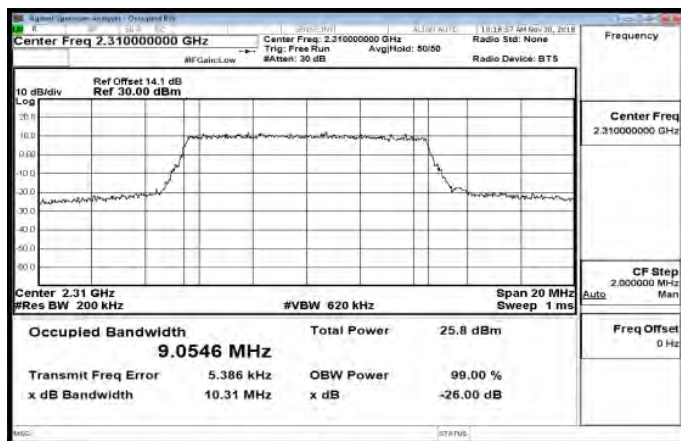
Band30_10MHz_64QAM_50_0_MidCH27710-2310
