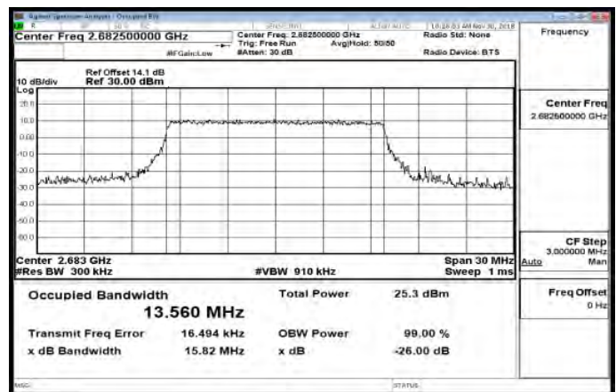
Band41_15MHz_64QAM_75_0_HighCH41515-2682.5
