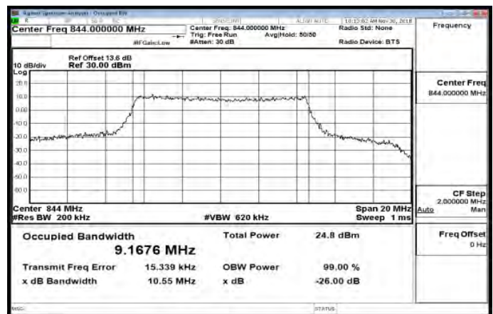
Band26_10MHz_64QAM_50_0_HighCH26990-844
