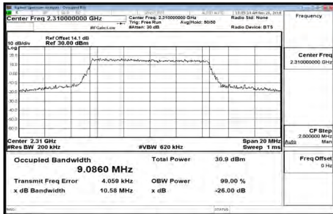
Band30_10MHz_16QAM_50_0_MidCH27710-2310
