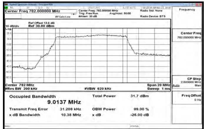
Band13_10MHz_16QAM_50_0_MidCH23230-782
