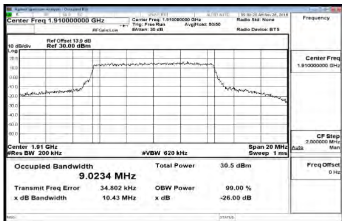
Band25_10MHz_16QAM_50_0_HighCH26640-1910
