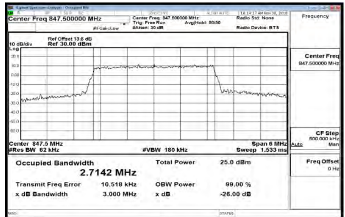
Band26_3MHz_64QAM_15_0_HighCH27025-847.5
