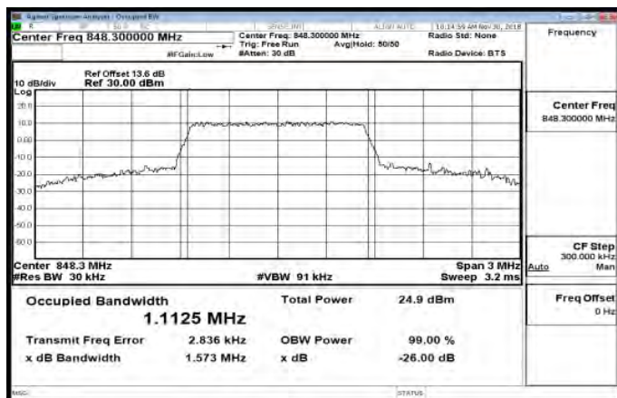
Band26_1_4MHz_64QAM_6_0_HighCH27033-848.3
