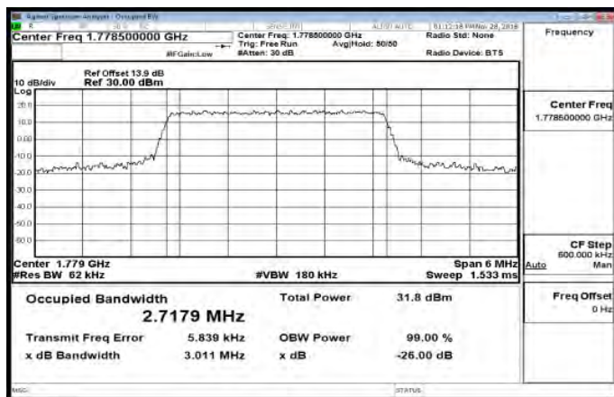
Band66_3MHz_QPSK_15_0_HighCH132657-1778.5
