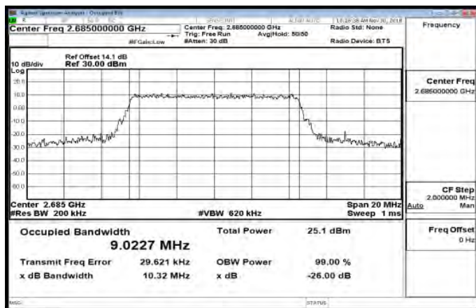
Band41_10MHz_64QAM_50_0_HighCH41540-2685
