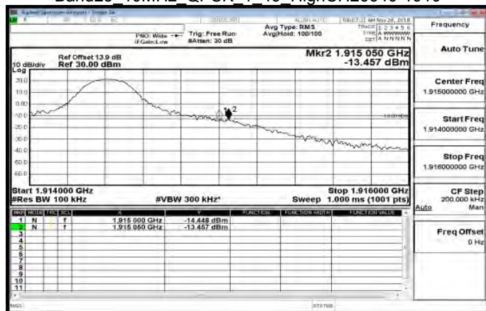
Band25 10MHz QPSK 1 49 HighCH26640-1910
