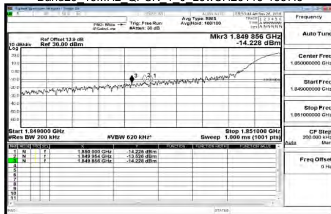
Band25 15MHz QPSK 1 0 LowCH26115-1857.5
