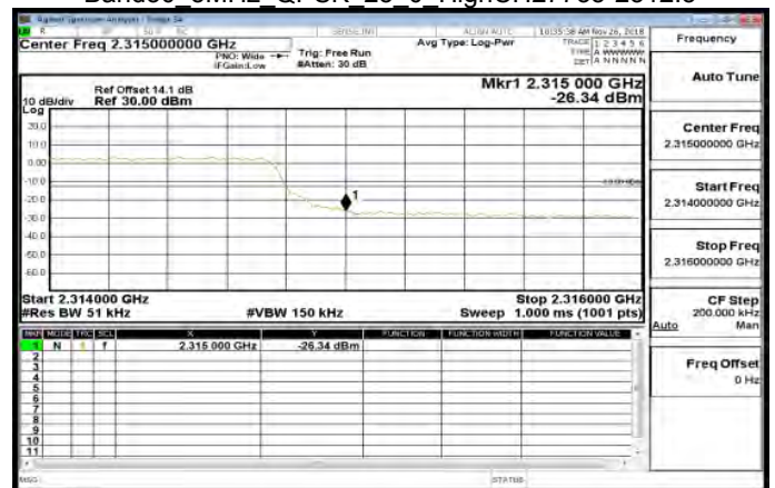
Band30 5MHz QPSK 25 0 HighCH27735-2312.5
