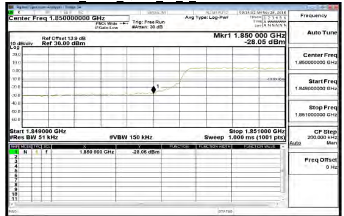
Band25 5MHz QPSK 25 0 LowCH26065-1852.5
