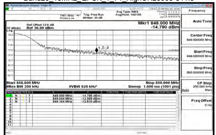
Band26 15MHz QPSK 1_74 HighCH26965-841.5
