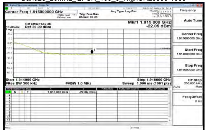
Band25 20MHz QPSK 100 0 HighCH26590-1905
