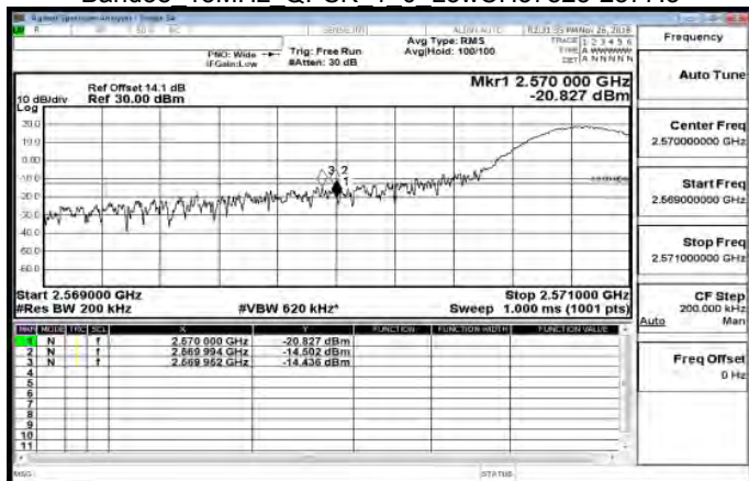
Band38 15MHz QPSK 1 0 LowCH37825-2577.5
