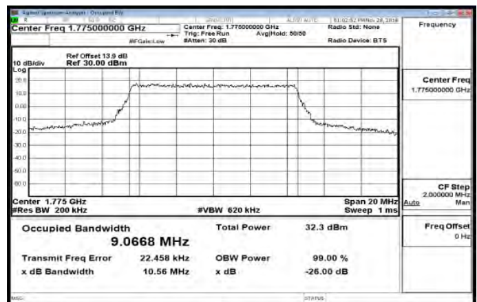
Band66_10MHz_16QAM_50_0_HighCH132622-1775
