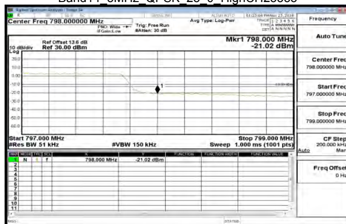
Band14 5MHz QPSK 25 0 HighCH23355
