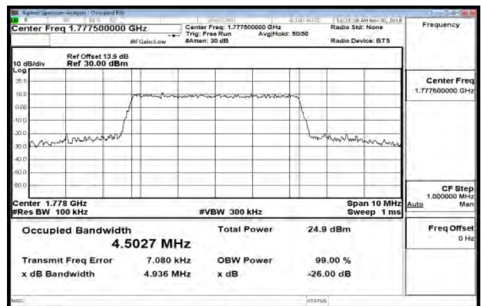
Band66_5MHz_64QAM_25_0_HighCH132647-1777.5
