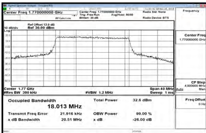
Band66_20MHz_QPSK_100_0_HighCH132572-1770
