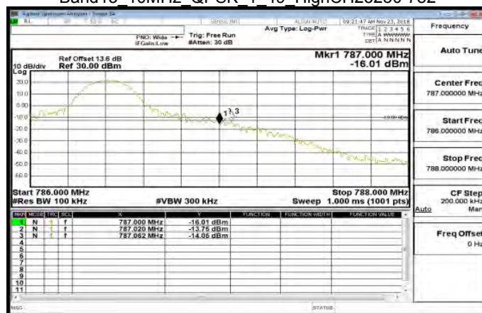
Band13 10MHz QPSK 1 49 HighCH23230-782
