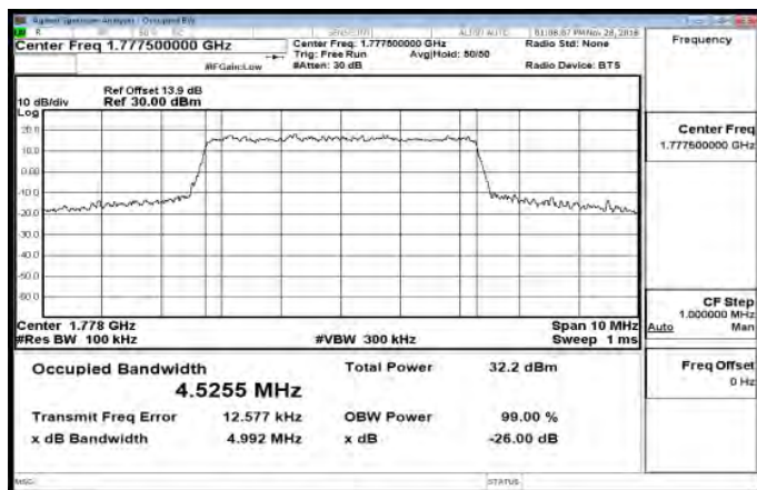
Band66_5MHz_16QAM_25_0_HighCH132647-1777.5
