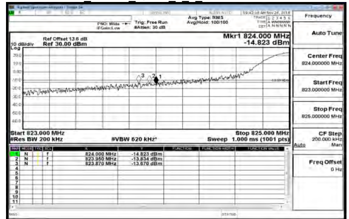
Band26 15MHz QPSK 1_0 LowCH26865-831.5
