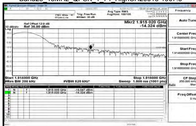
Band25 15MHz QPSK 1 74 HighCH26615-1907.5
