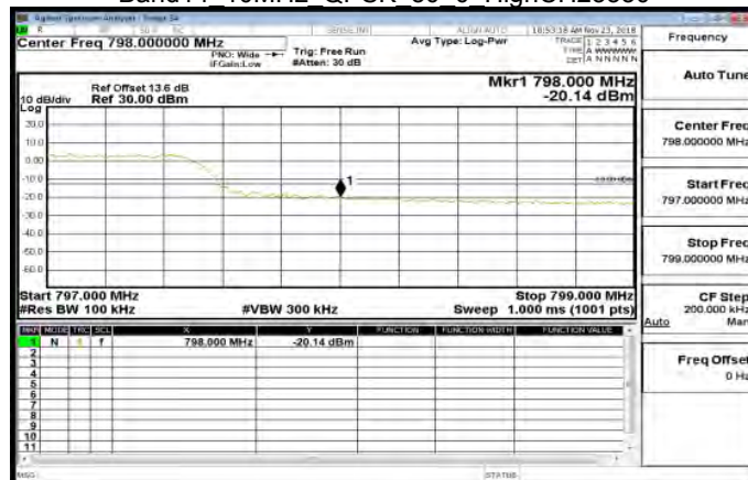
Band14 10MHz QPSK 50 0 HighCH23330
