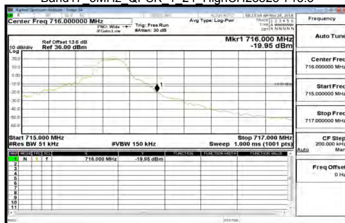
Band17 5MHz QPSK 1 24 HighCH23825-713.5
