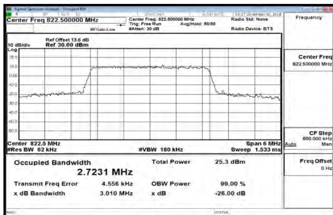
Part 90_Band26_3MHz_64QAM_15_0_HighCH26775-822.5
