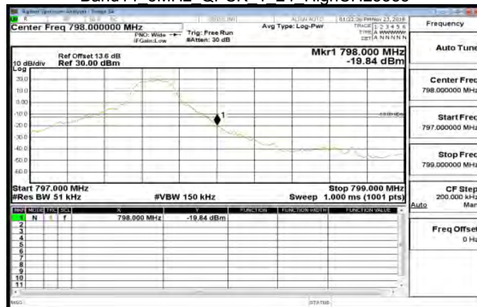
Band14 5MHz QPSK 1 24 HighCH23355
