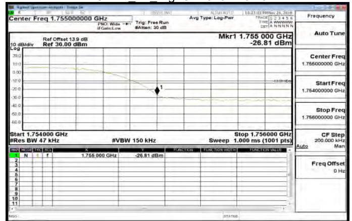
HSDPA B4 HighCH1513-1752.6
