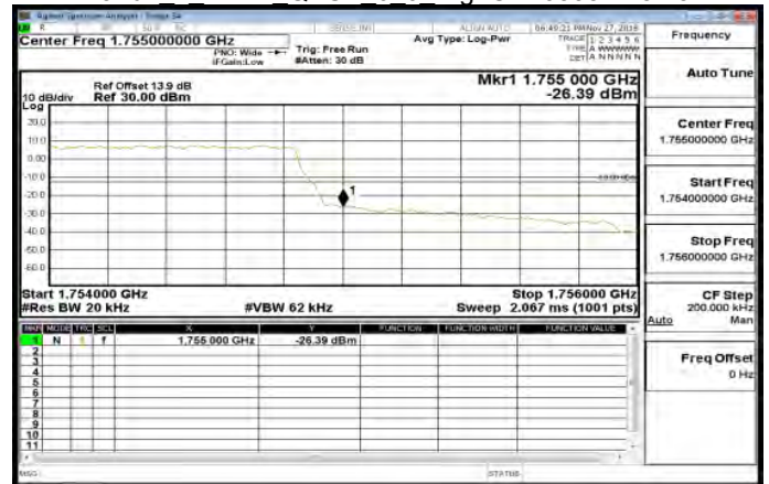
Band4 1 4MHz QPSK 6 0 HighCH20393-1754.3
