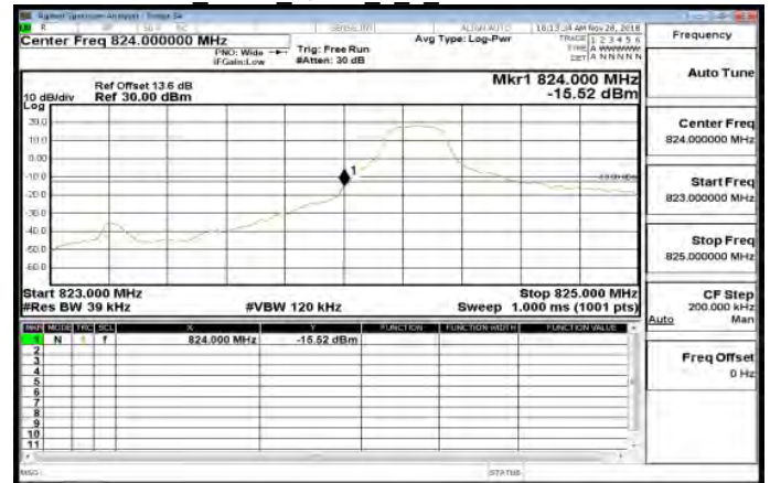
Band26 3MHz QPSK 1 0 LowCH26805-825.5
