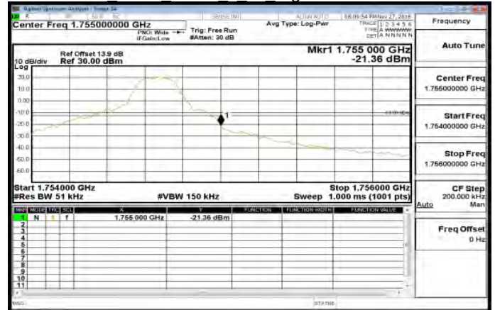
Band4 5MHz QPSK 1 24 HighCH20375-1752.5
