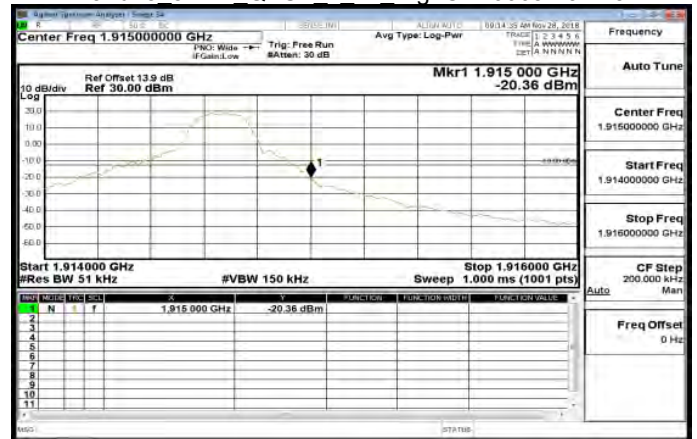
Band25 5MHz QPSK 1 24 HighCH26665-1912.5
