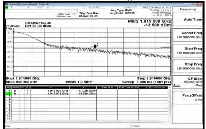
Band25 20MHz QPSK 1 99 HighCH26590-1905
