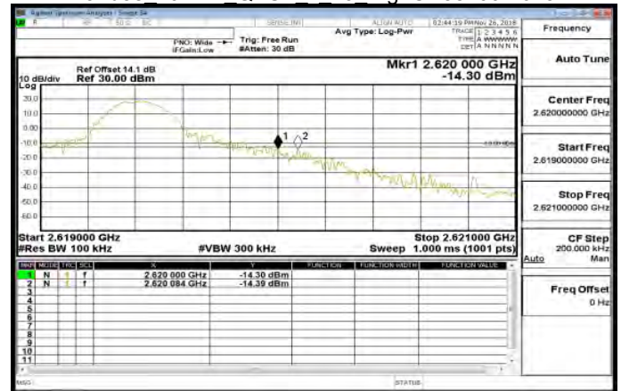
Band38 10MHz QPSK 1 49 HighCH38200-2615
