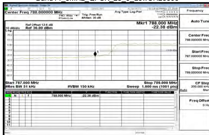
Band14 5MHz QPSK 25 0 LowCH23305
