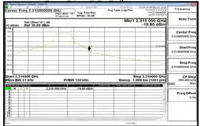
Band30 5MHz QPSK 1 24 HighCH27735-2312.5
