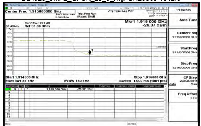
Band25 5MHz QPSK 25 0 HighCH26665-1912.5
