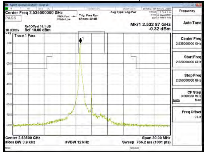
Band 7 64QAM 5M RB1,24
