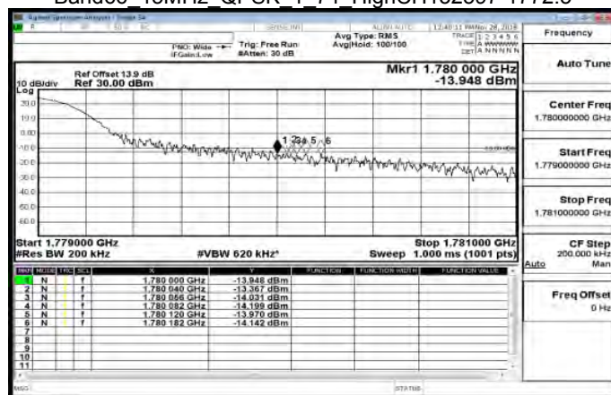
Band66 15MHz QPSK 1 74 HighCH132597-1772.5
