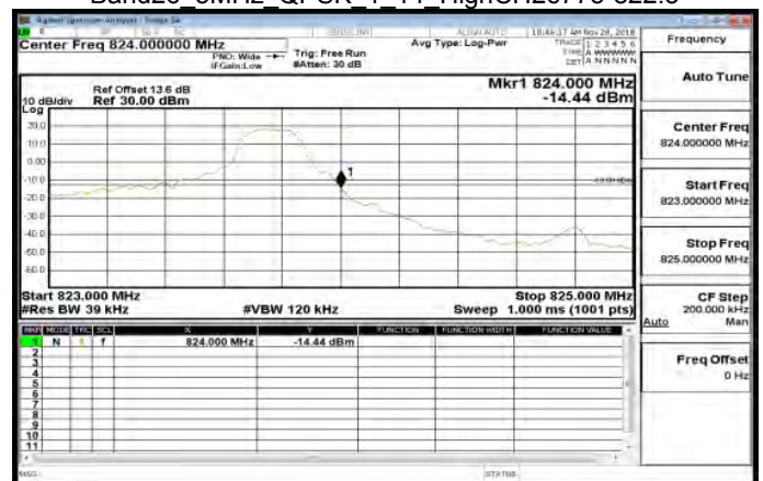
Band26 3MHz QPSK 1 14 HighCH26775-822.5
