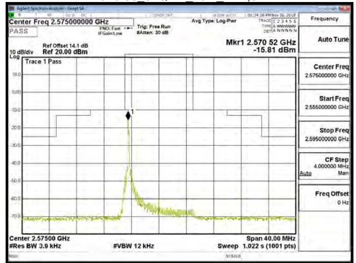
Band 38 64QAM 10M RB1,49
