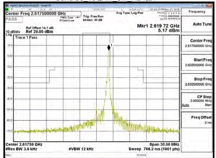
Band 38 16QAM 5M RB25,0
