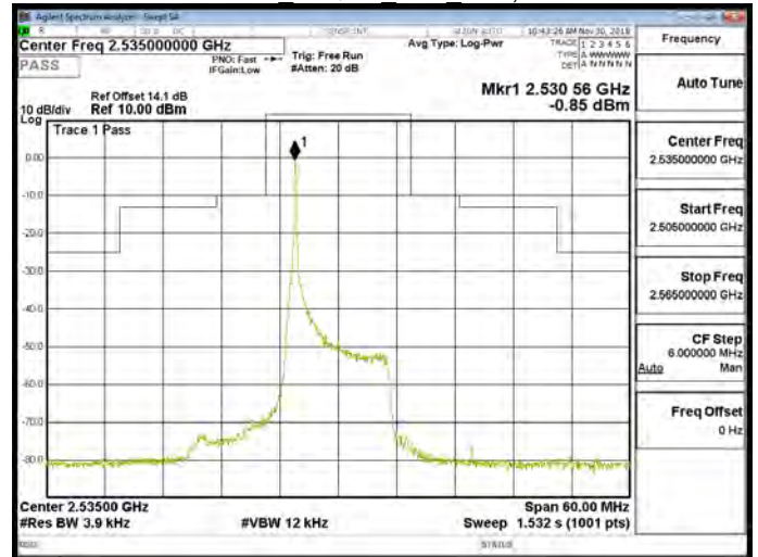
Band 7 64QAM 15M RB75,0
