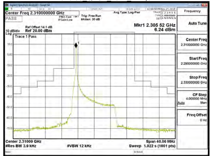
Band 30 QPSK 10M RB1,49
