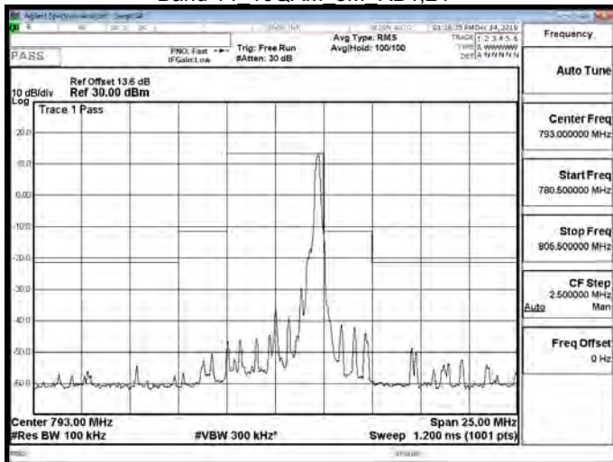
Band 14 16QAM 5M RB25,0
