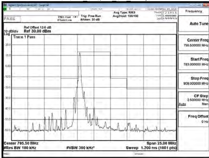
Band 14 64QAM 5M RB1,24
