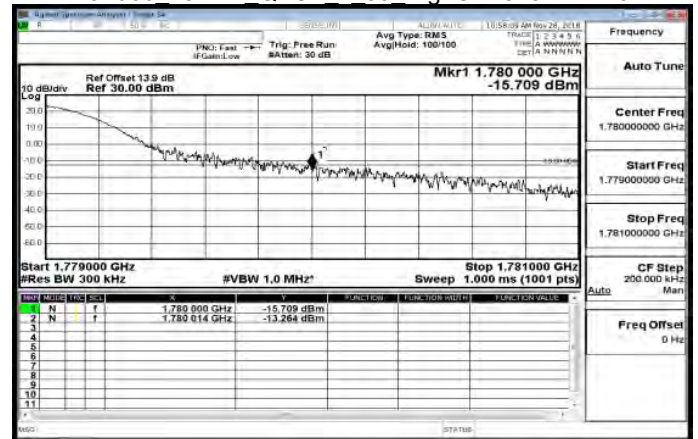
Band66 20MHz QPSK 1 99 HighCH132572-1770
