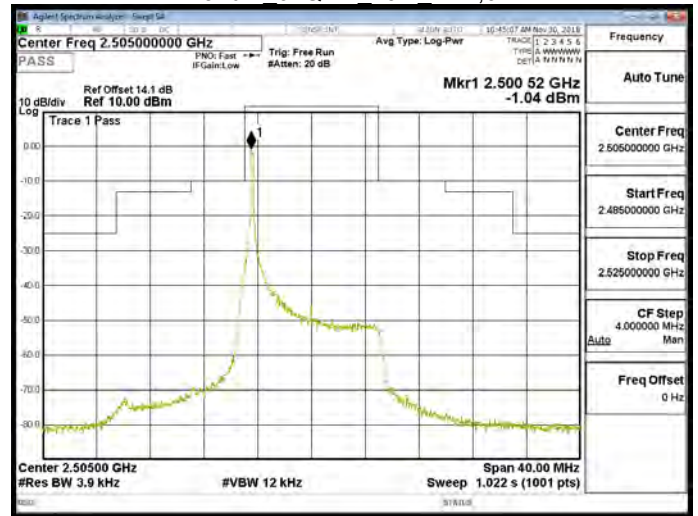
Band 7 64QAM 10M RB1,49
