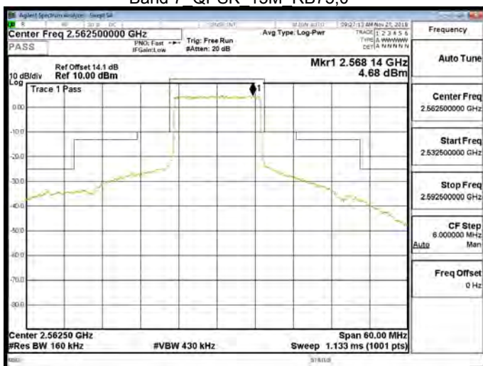
Band 7 QPSK 15M RB75,0
