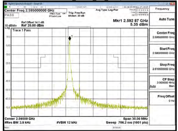
Band 38 QPSK 5M RB1,24
