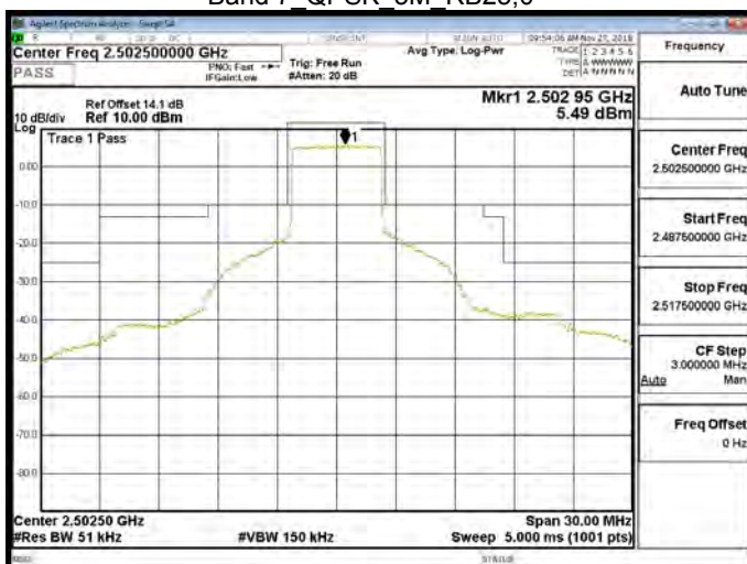
Band 7 QPSK 5M RB25,0
