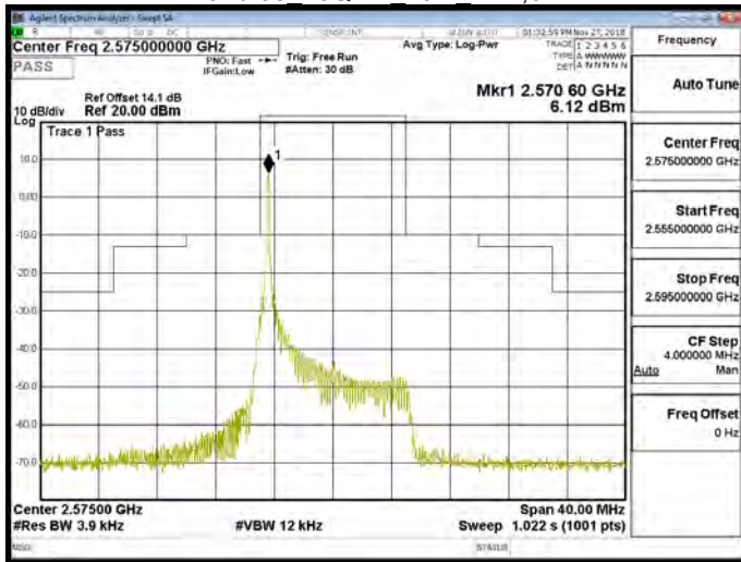
Band 38 16QAM 10M RB1,49
