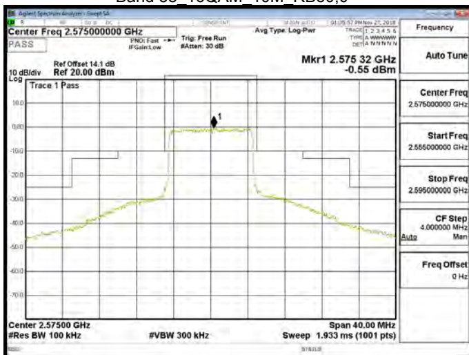
Band 38 16QAM 10M RB50,0
