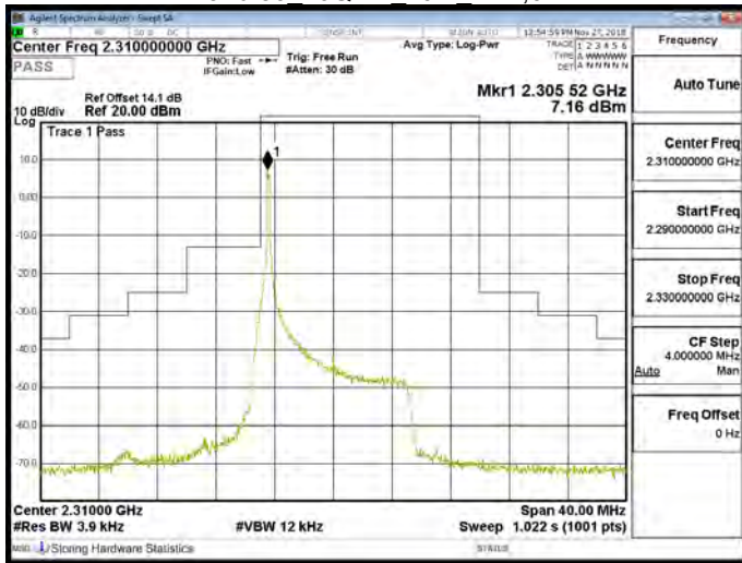
Band 30 16QAM 10M RB1,49
