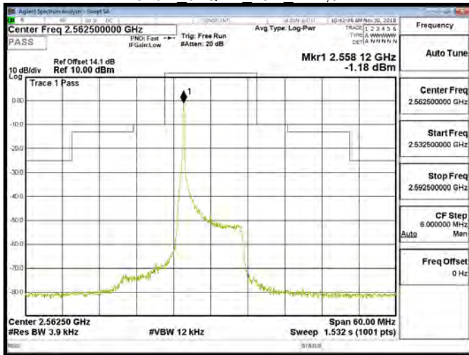
Band 7 64QAM 15M RB1,74
