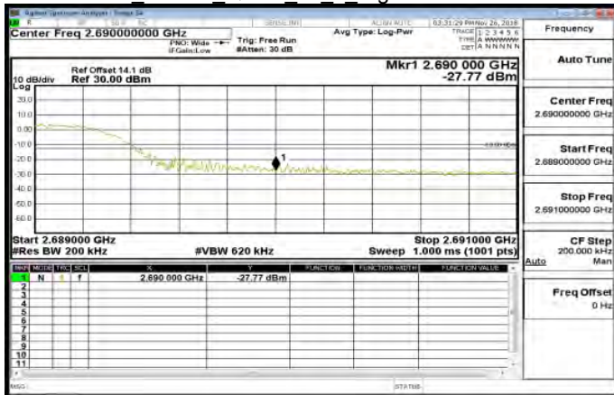
Band41 15MHz QPSK 75 0 HighCH41515-2682.5
