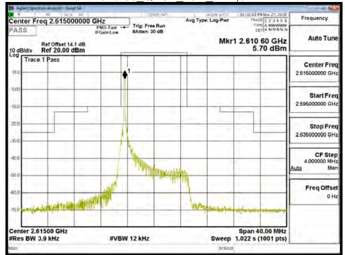
Band 38 QPSK 10M RB1,49
