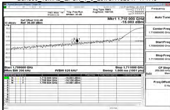
Band66 15MHz QPSK 1 0 LowCH132047-1717.5
