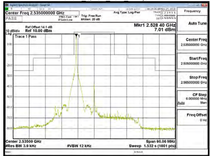
Band 7 QPSK 15M RB1,74
