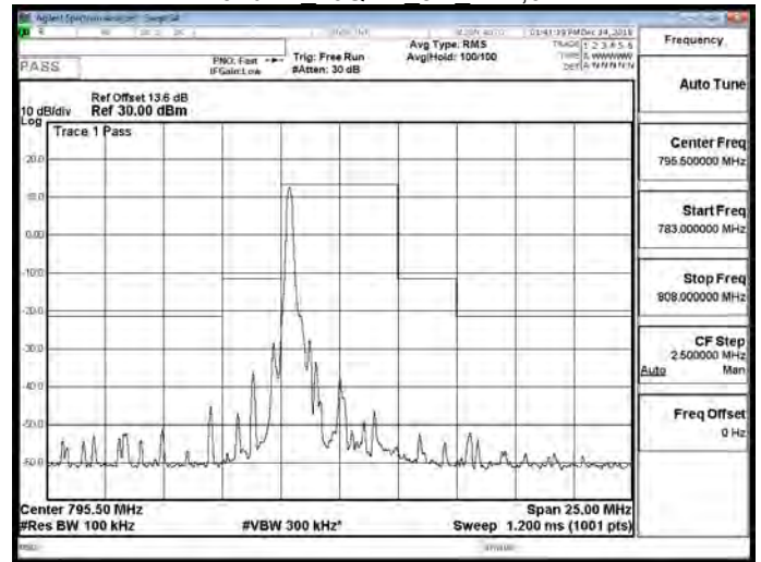
Band 14 16QAM 5M RB1,24
