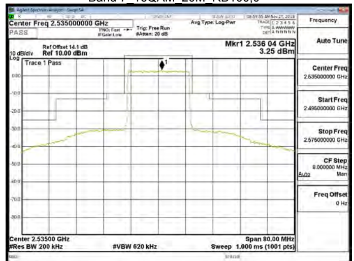
Band 7 16QAM 20M RB100,0
