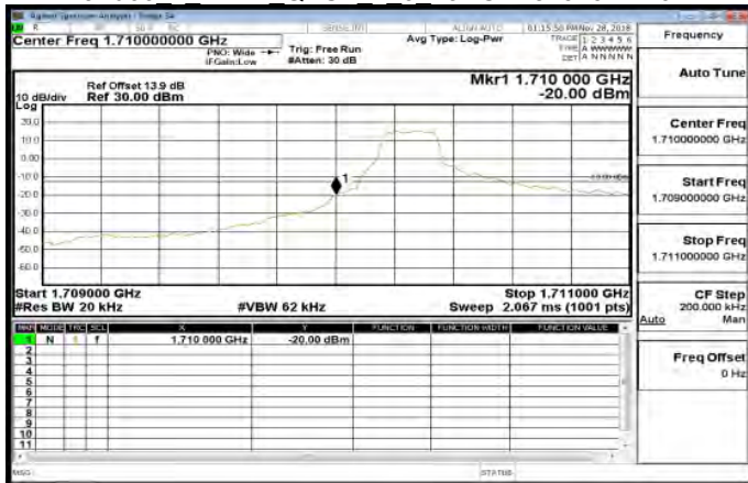
Band66 1 4MHz QPSK 1 0 LowCH131979-1710.7
