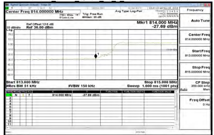
Band26 5MHz QPSK 25 0 LowCH26715-816.5
