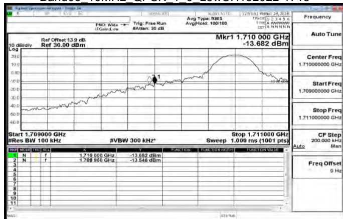
Band66 10MHz QPSK 1 0 LowCH132022-1715
