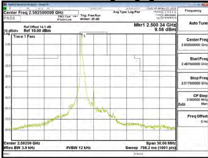
Band 7 QPSK 5M RB1,24
