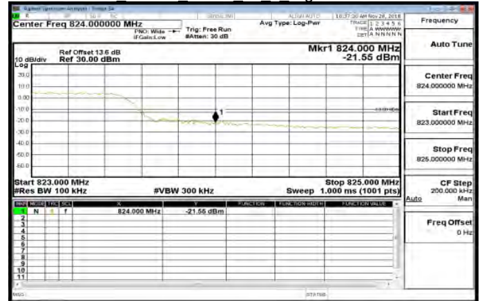
Band26 10MHz QPSK 50 0 HighCH26740-819
