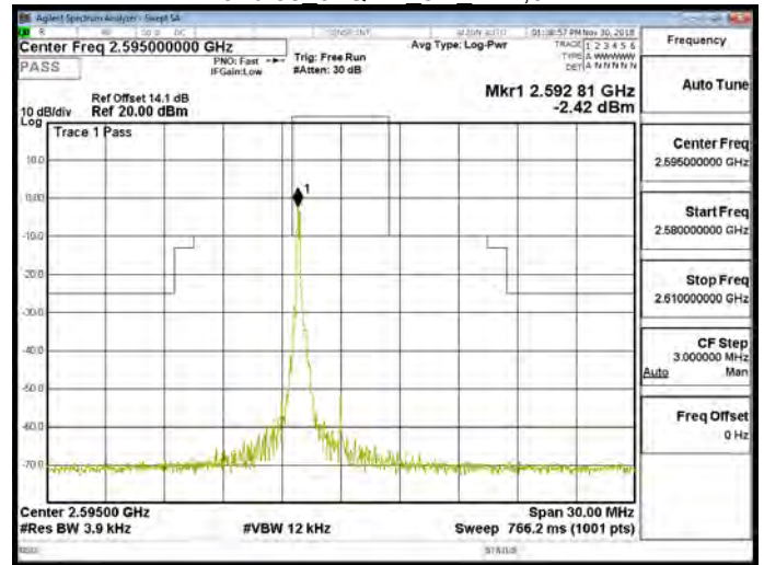
Band 38 64QAM 5M RB1,24
