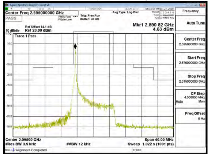
Band 38 16QAM 10M RB1,49
