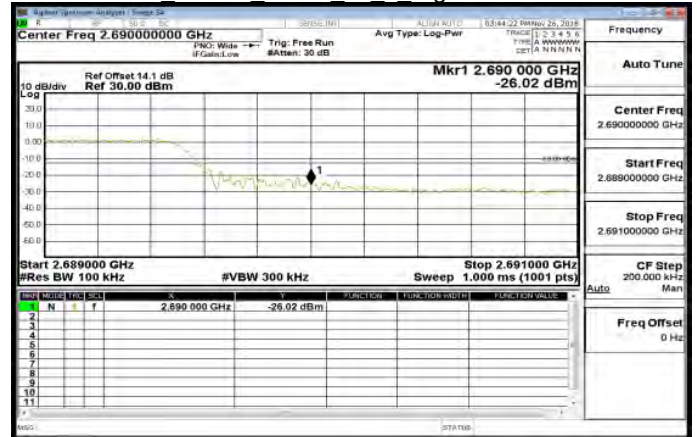
Band41 10MHz QPSK 50 0 HighCH41540-2685
