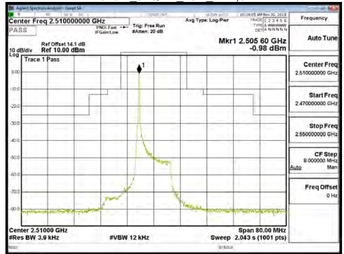
Band 7 64QAM 20M RB1,99
