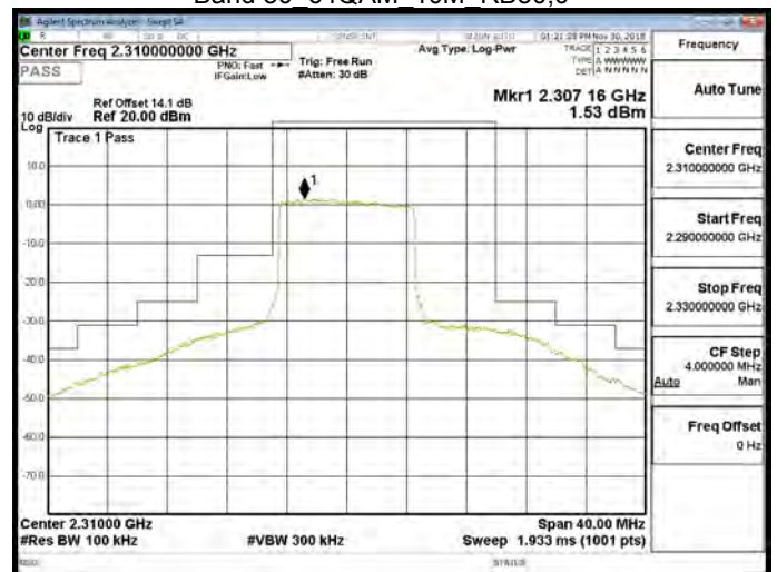
Band 30 64QAM 10M RB50,0
