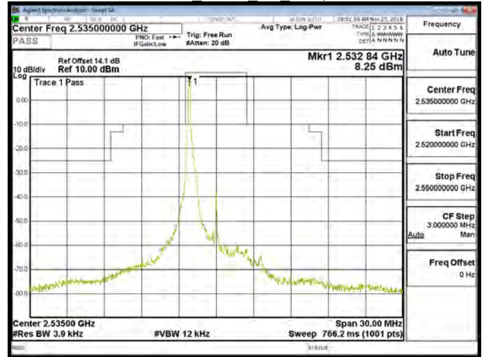
Band 7 QPSK 5M RB1,24
