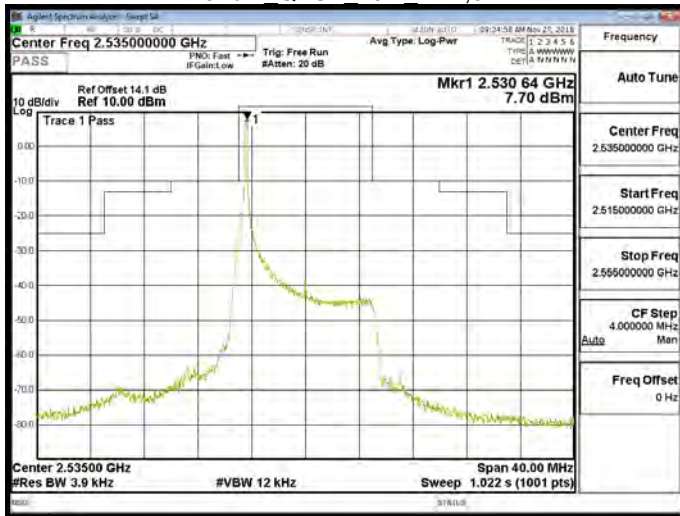
Band 7 QPSK 10M RB1,49
