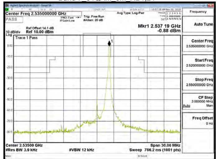
Band 7 64QAM 5M RB25,0
