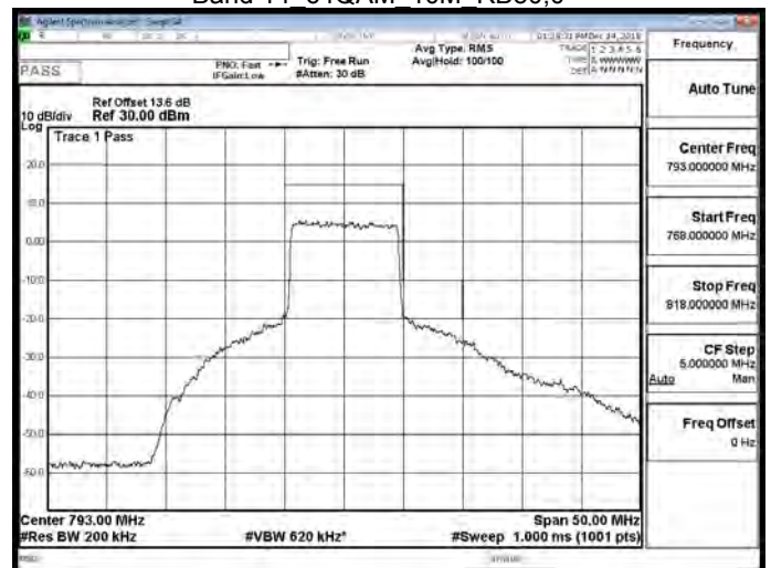
Band 14 64QAM 10M RB50,0
