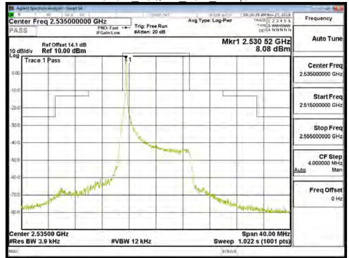
Band 7 16QAM 10M RB1,49
