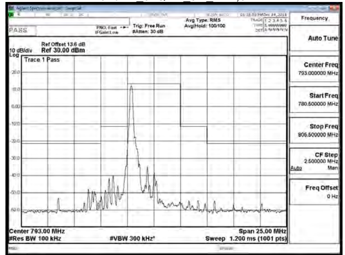
Band 14 64QAM 5M RB1,24
