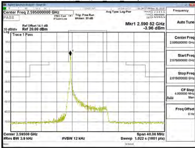
Band 38 64QAM 10M RB1,49
