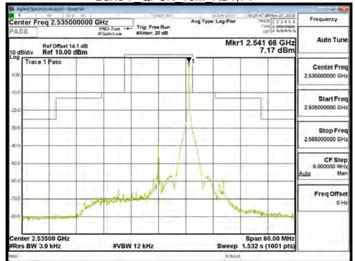
Band 7 QPSK 15M RB75,0
