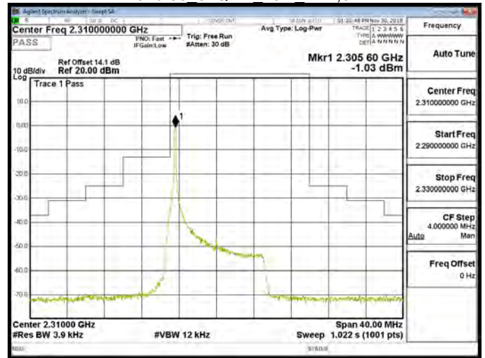
Band 30 64QAM 10M RB1,49
