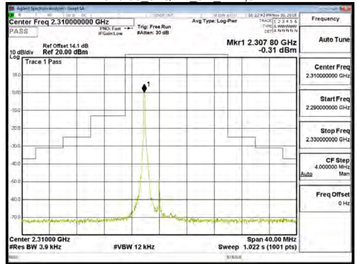
Band 30 64QAM 5M RB1,24
