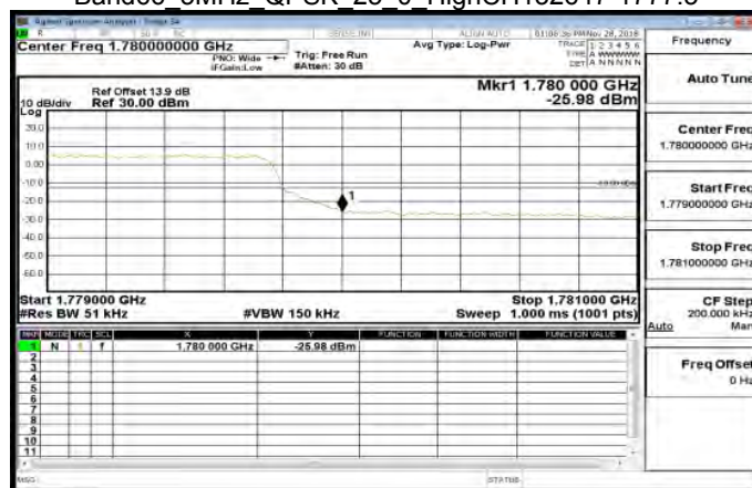
Band66 5MHz QPSK 25 0 HighCH132647-1777.5
