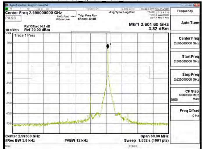
Band 38 QPSK 15M RB75,0
