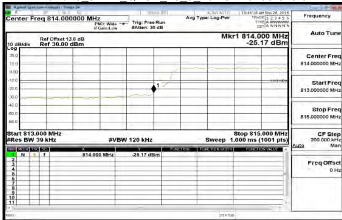
Band26 3MHz QPSK 15 0 LowCH26705-815.5
