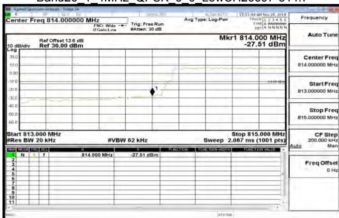
Band26 1 4MHz QPSK 6 0 LowCH26697-814.7
