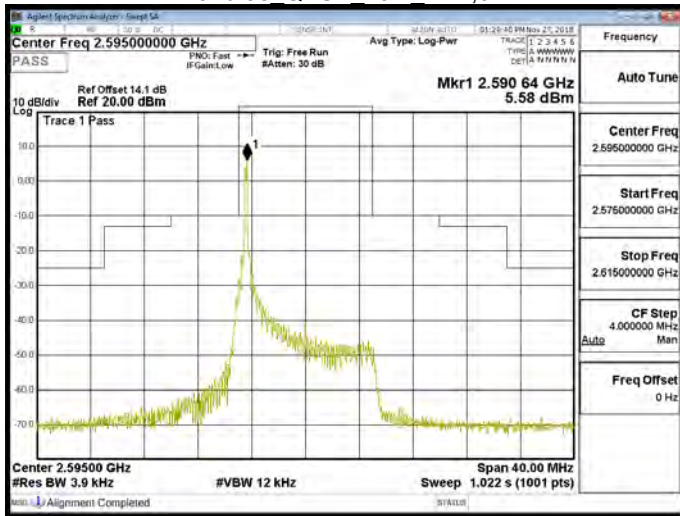
Band 38 QPSK 10M RB1,49
