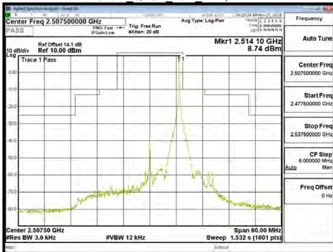
Band 7 QPSK 15M RB75,0
