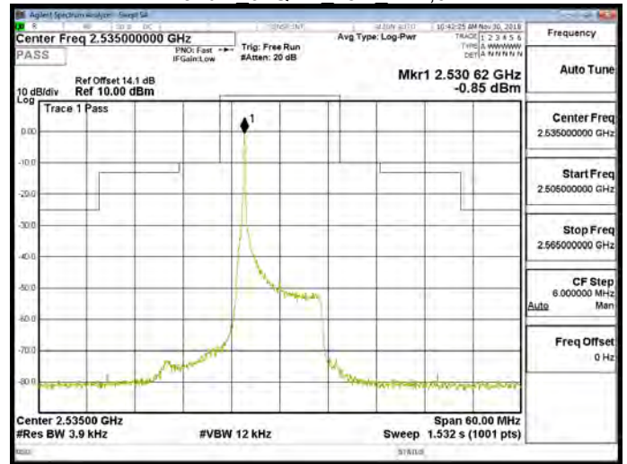
Band 7 64QAM 15M RB1,74
