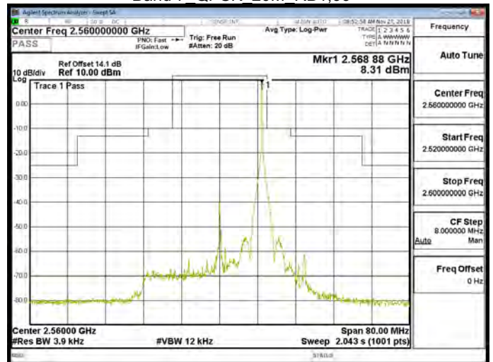
Band 7 QPSK 20M RB100,0
