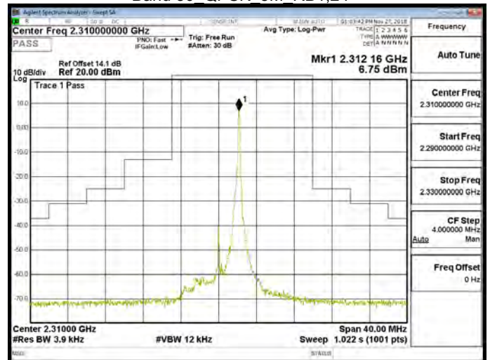
Band 30 QPSK 5M RB25,0
