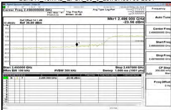
Band41 10MHz QPSK 50 0 LowCH39700-2501
