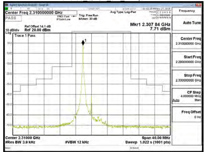
Band 30 QPSK 5M RB1,24
