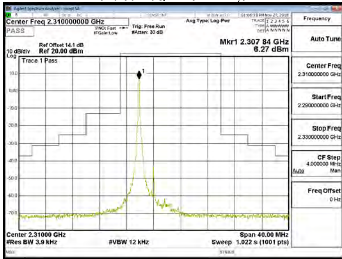
Band 30 16QAM 5M RB1,24
