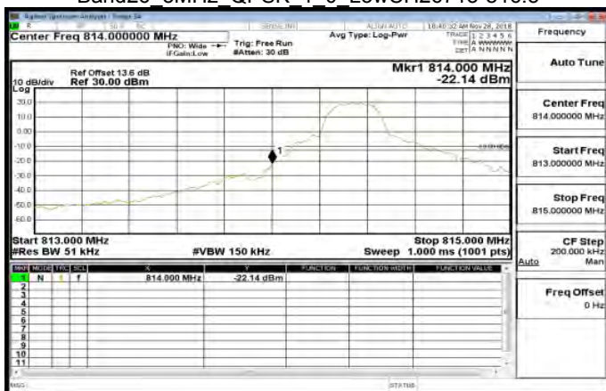
Band26 5MHz QPSK 1 0 LowCH26715-816.5
