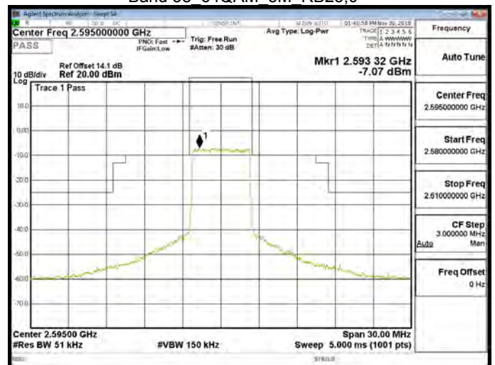
Band 38 64QAM 5M RB25,0
