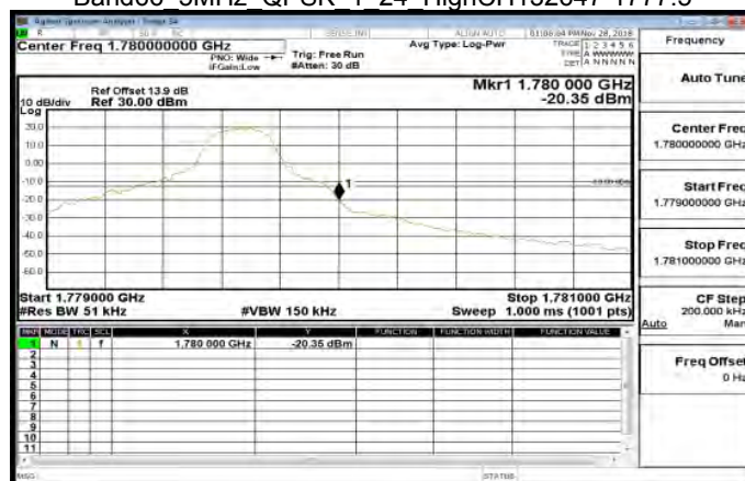
Band66 5MHz QPSK 1 24 HighCH132647-1777.5
