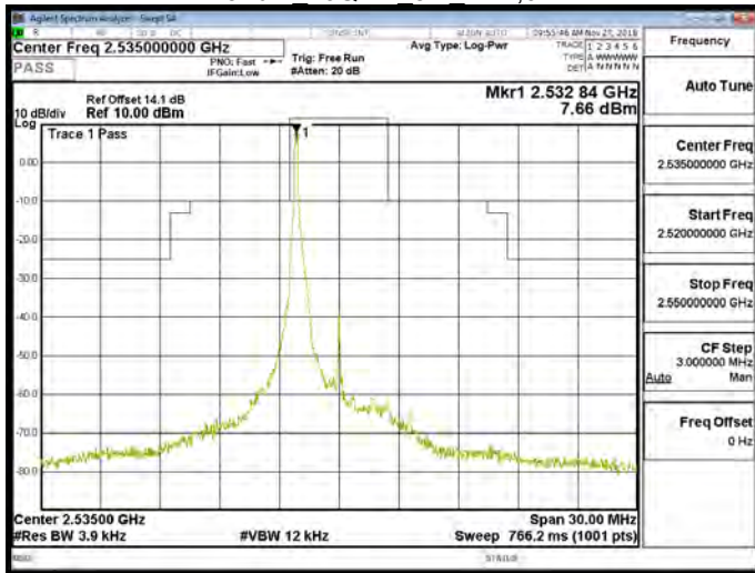
Band 7 16QAM 5M RB1,24
