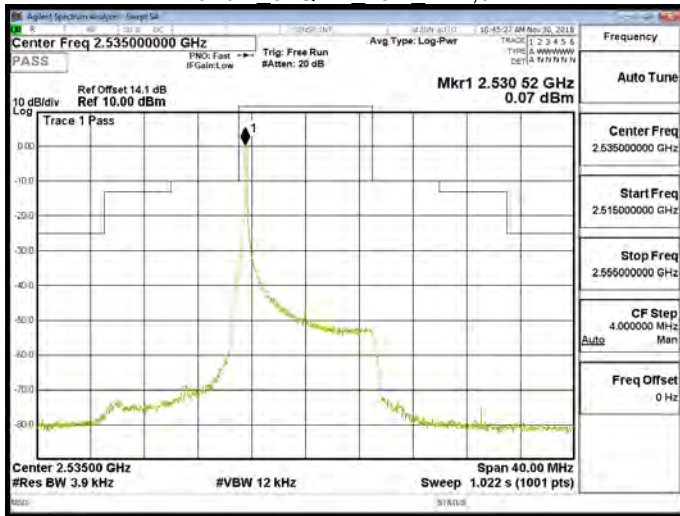
Band 7 64QAM 10M RB1,49
