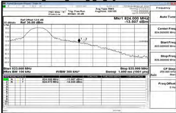
Band26 10MHz QPSK 1 49 HighCH26740-819
