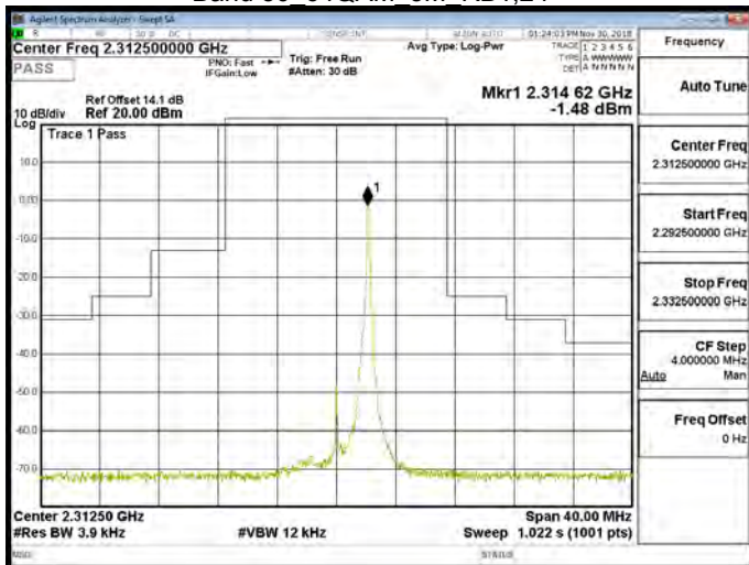
Band 30 64QAM 5M RB25,0
