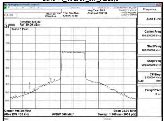
Band 14 16QAM 5M RB25,0
