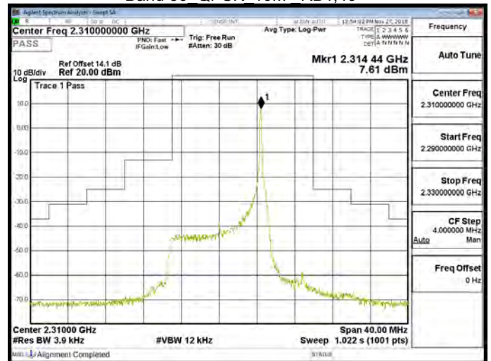
Band 30 QPSK 10M RB50,0
