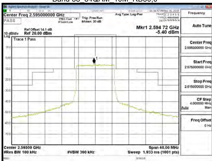
Band 38 64QAM 10M RB50,0
