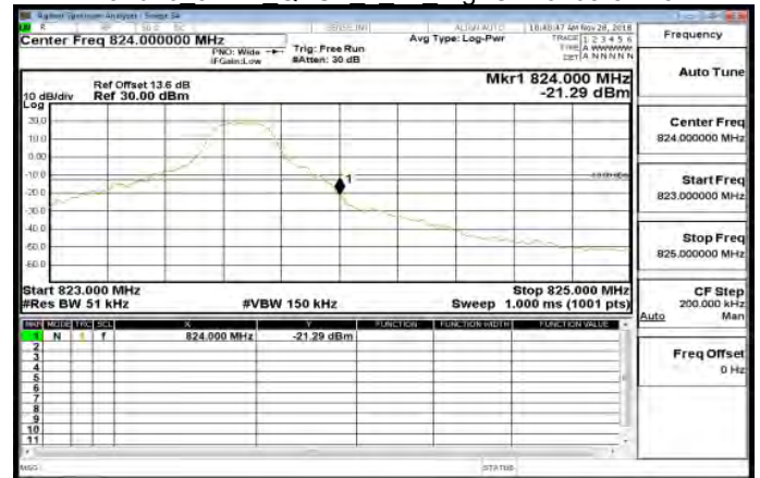
Band26 5MHz QPSK 1 24 HighCH26765-821.5
