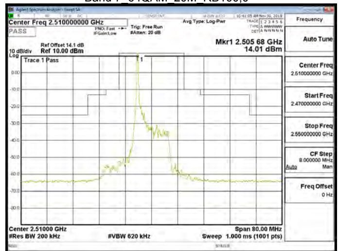
Band 7 64QAM 20M RB100,0
