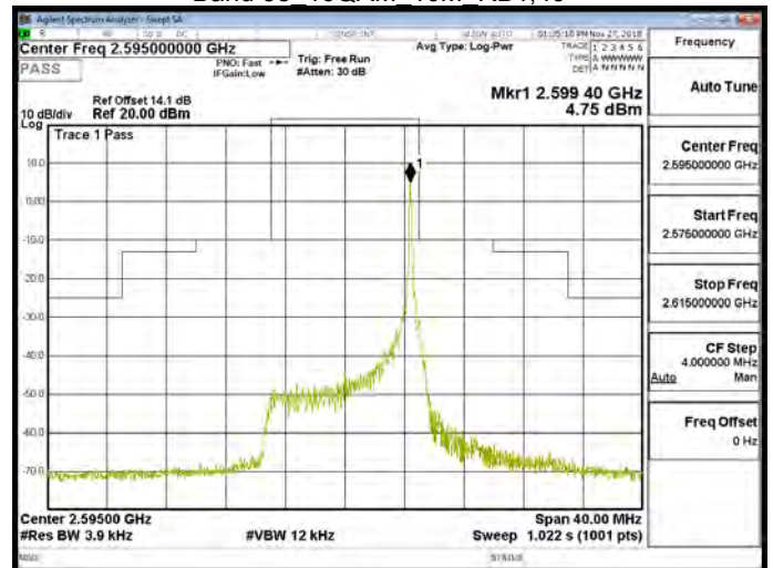
Band 38 16QAM 10M RB50,0
