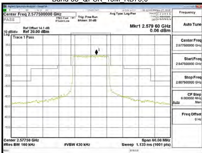
Band 38 QPSK 15M RB75,0
