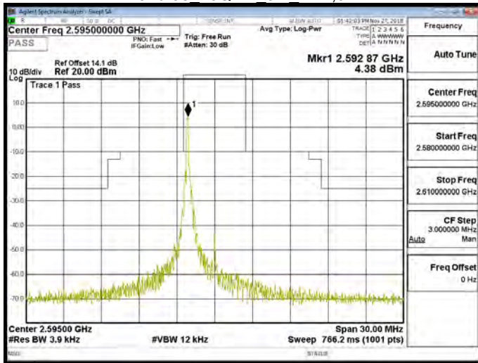
Band 38 16QAM 5M RB1,24
