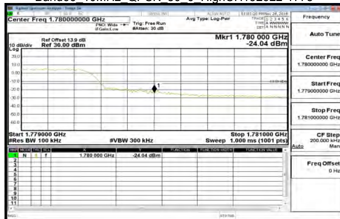
Band66 10MHz QPSK 50 0 HighCH132622-1775
