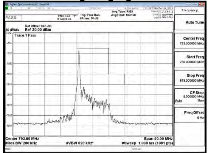
Band 14 64QAM 10M RB1,49
