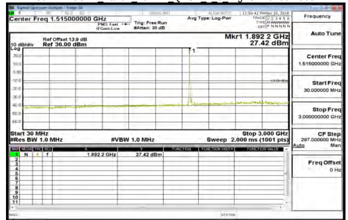
30MHz~3GHz Band2 20MHz QPSK 1 0 HighCH19100-1900
