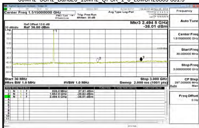
30MHz~3GHz Band26 15MHz QPSK 1 0 LowCH26865-831.5
