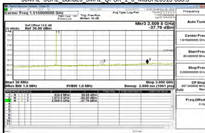
30MHz~3GHz Band26 5MHz QPSK 1 0 MidCH26915-836.5
