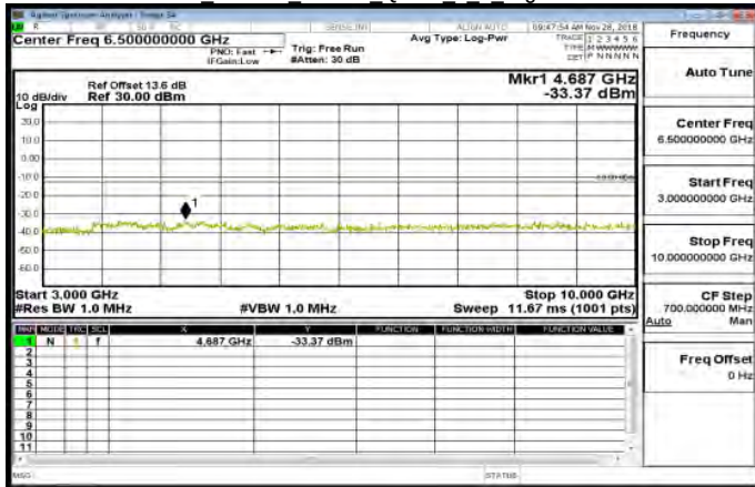
3GHz~10GHz Band26 15MHz QPSK 1 0 HighCH26965-841.5
