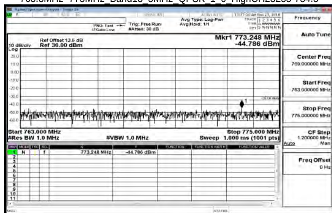
763.3MHz~775MHz Band13 5MHz QPSK 1 0 HighCH23255-784.5
