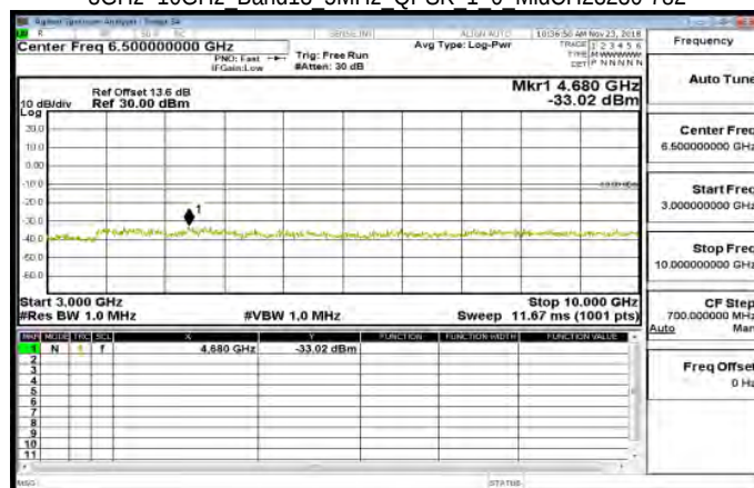
3GHz~10GHz Band13 5MHz QPSK 1 0 MidCH23230-782
