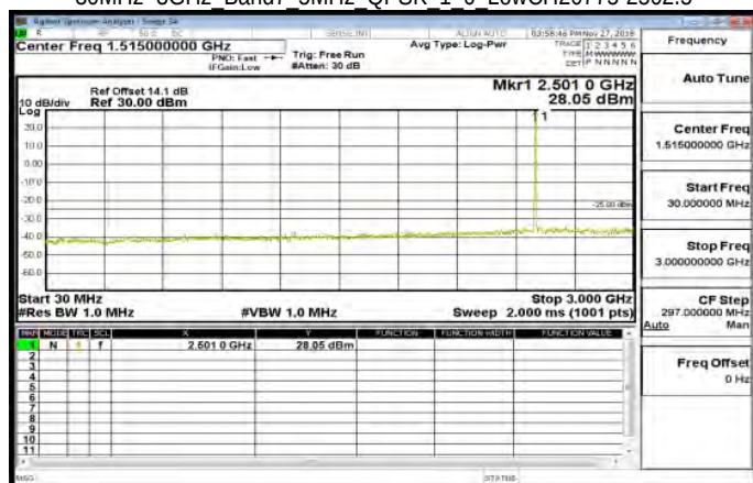
30MHz~3GHz Band7 5MHz QPSK 1 0 LowCH20775-2502.5
