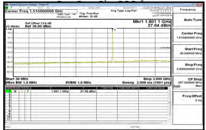
30MHz~3GHz Band2 10MHz QPSK 1 0 HighCH19150-1905
