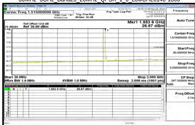
30MHz~3GHz Band25 20MHz QPSK 1 0 LowCH26140-1860
