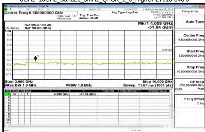
3GHz~10GHz Band26 5MHz QPSK 1 0 HighCH27015-846.5
