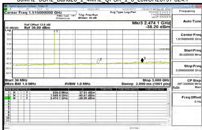
30MHz~3GHz Band26 1 4MHz QPSK 1 0 LowCH26797-824.7
