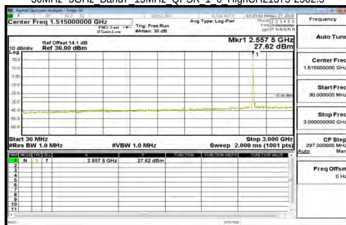
30MHz~3GHz Band7 15MHz QPSK 1 0 HighCH21375-2562.5
