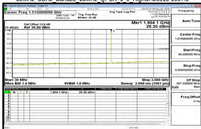
30MHz~3GHz Band25 15MHz QPSK 1 0 HighCH26615-1907.5
