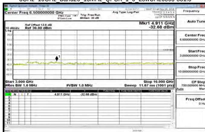
3GHz~10GHz Band26 15MHz QPSK 1 0 LowCH26865-831.5
