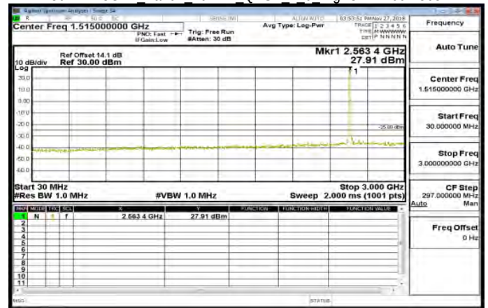
30MHz~3GHz Band7 10MHz QPSK 1 0 HighCH21400-2565
