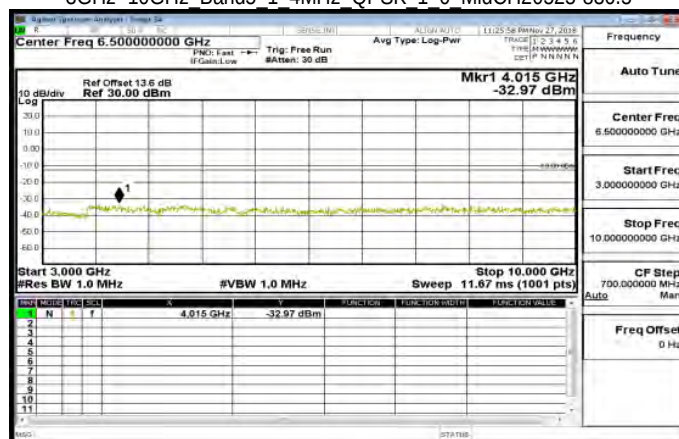
3GHz~10GHz Band5 1 4MHz QPSK 1 0 MidCH20525-836.5
