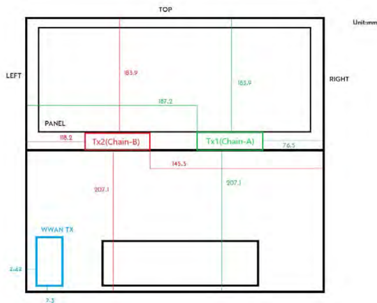
Fig.10 Antenna location of EUT (Laptop mode)
