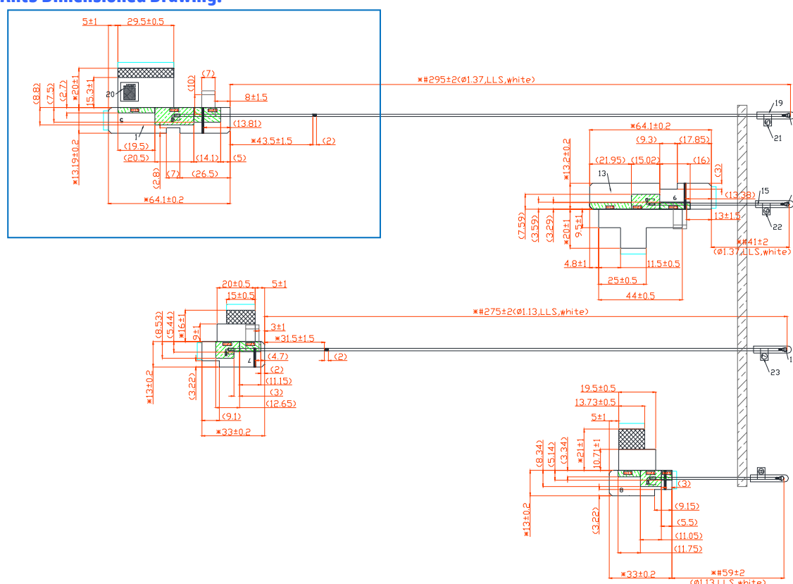
Ant5 Dimensioned Drawing:
