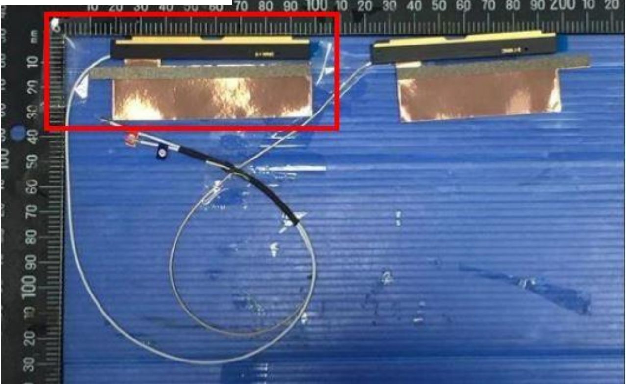
WWAN Main Antenna for Vendor 1
