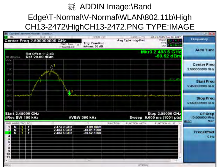
802.11b: Band Edges Test Data CH-13
