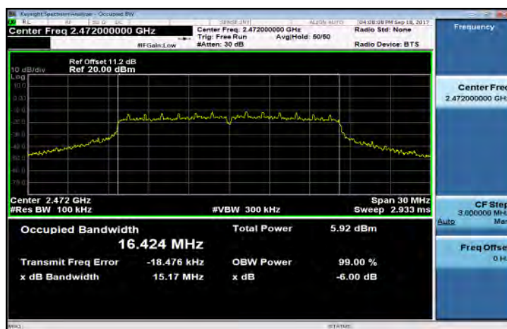
802.11g (Main) CH-13
