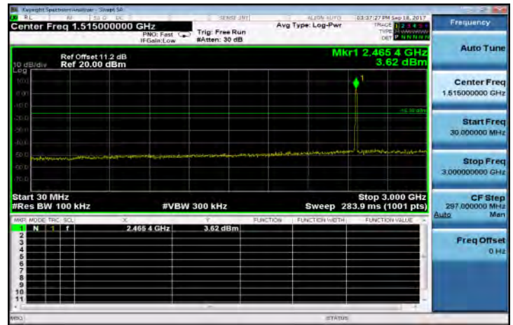
802.11b: Spurious Emission Test Data CH-12
