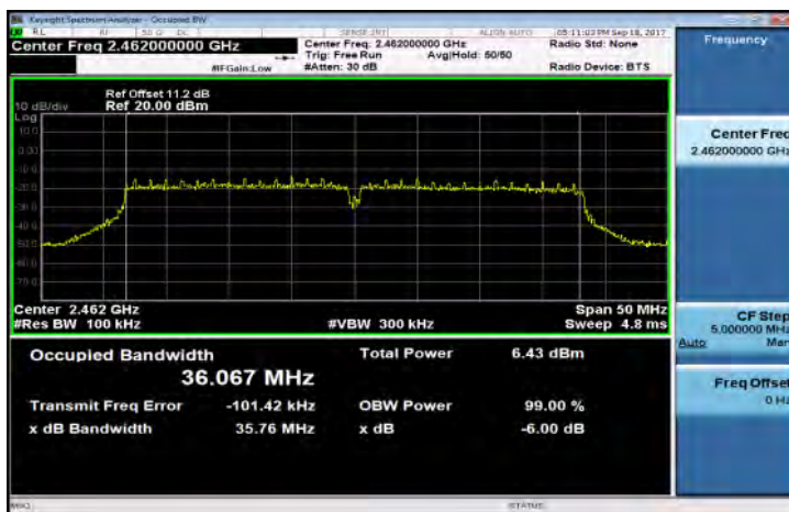
802.11n_40M (Main) CH-11
