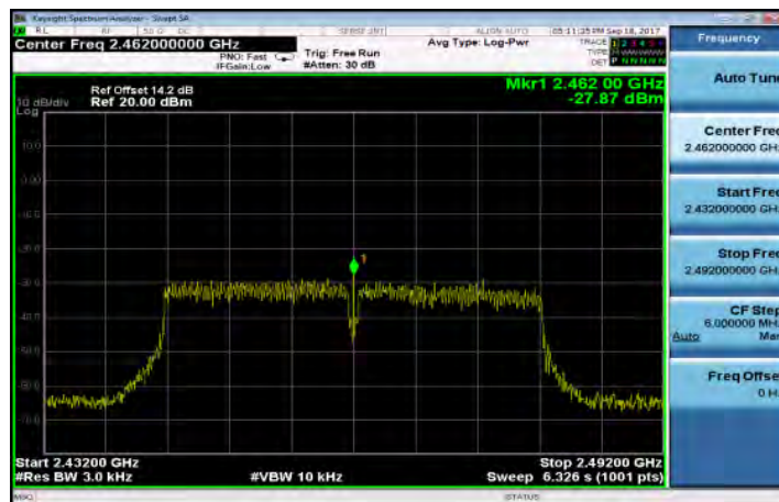
802.11n_HT40 PSD (CH-11)
