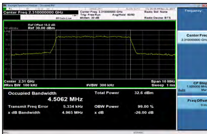
Band30_5MHz_16QAM_25_0_HighCH27735
