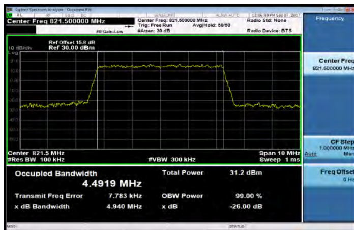
Part 90_Band26_5MHz_16QAM_25_0_HighCH26765
