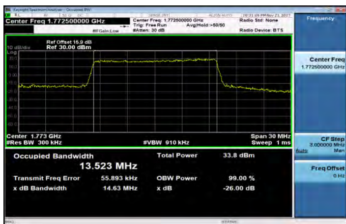
Band66_15MHz_QPSK_75_0_HighCH132597
