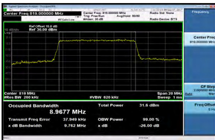
Part 90_Band26_10MHz_64QAM_50_0_MidCH26740
