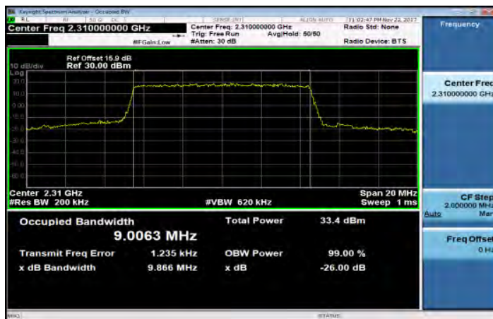
Band30_10MHz_16QAM_50_0_MidCH27710
