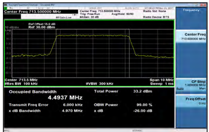
Band17_5MHz_64QAM_25_0_HighCH23825-713.5
