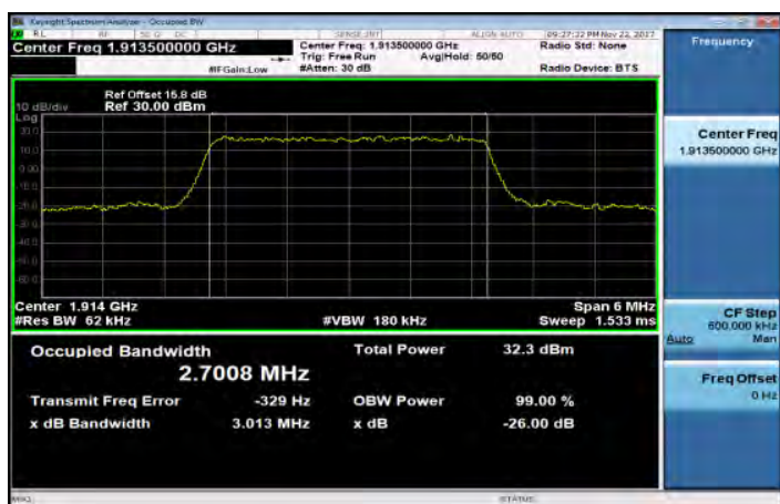
Band25_3MHz_QPSK_15_0_HighCH26675-1913.5
