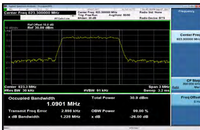
Part 90_Band26_1_4MHz_16QAM_6_0_HighCH26783
