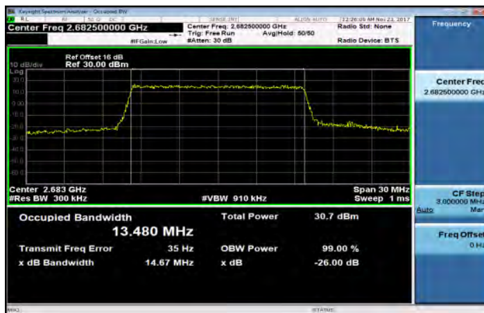
Band41_15MHz_16QAM_75_0_HighCH41515
