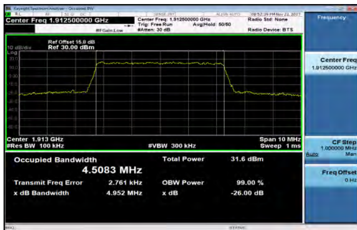
Band25_5MHz_16QAM_25_0_HighCH26665-1912.5
