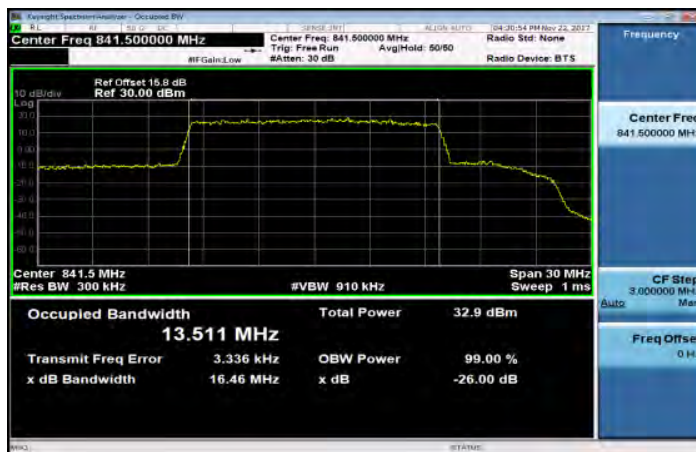
Band26_15MHz_64QAM_75_0_HighCH26965-841.5
