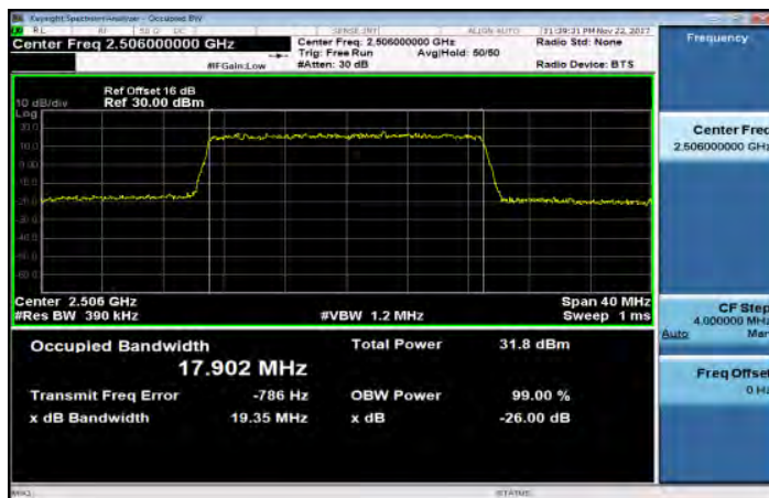
Band41_20MHz_64QAM_100_0_MidCH40620
