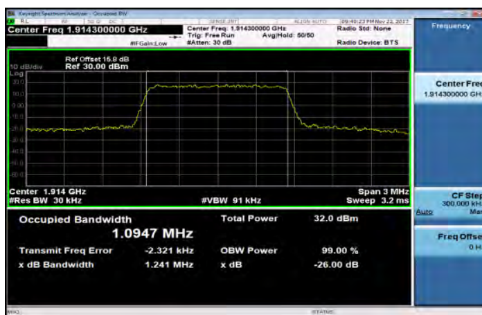
Band25_1_4MHz_QPSK_6_0_HighCH26683-1914.3
