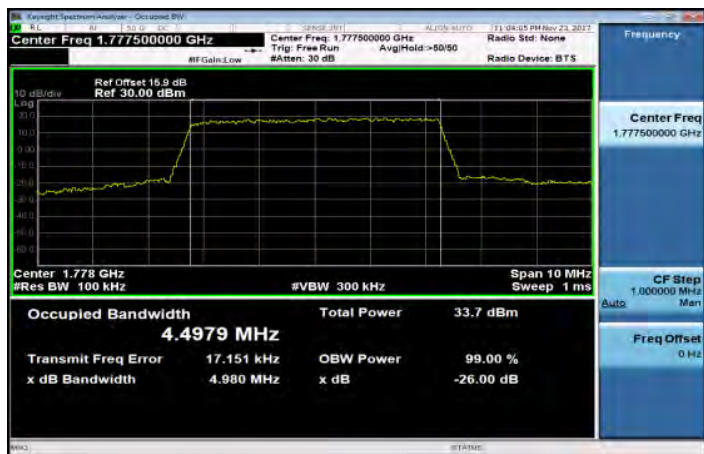
Band66_5MHz_QPSK_25_0_HighCH132647
