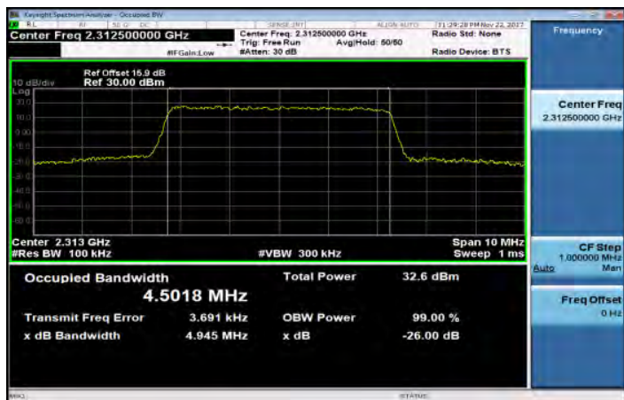
Band30_5MHz_64QAM_25_0_HighCH27735
