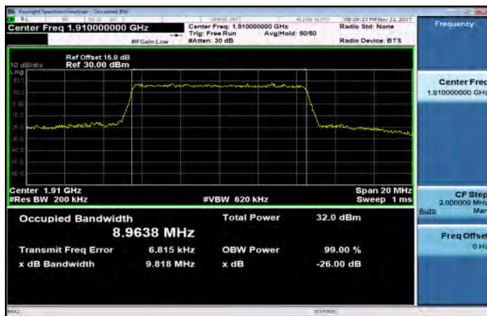
Band25_10MHz_16QAM_50_0_HighCH26640-1910
