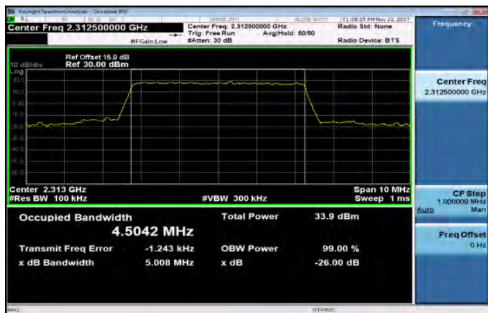
Band30_5MHz_QPSK_25_0_HighCH27735
