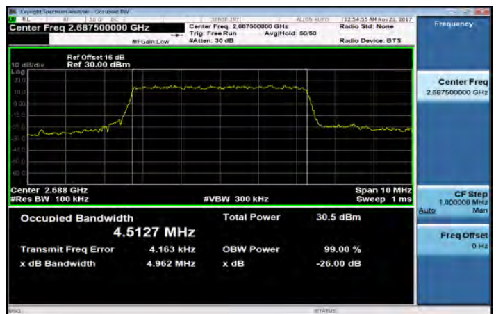
Band41_5MHz_16QAM_25_0_HighCH41565
