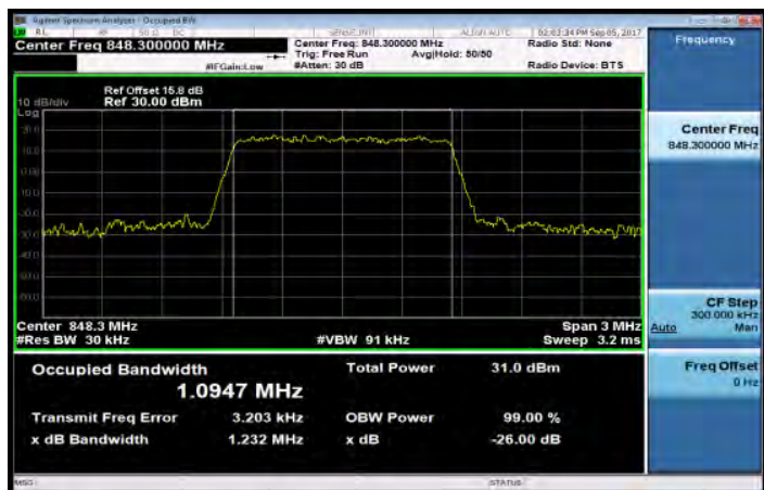
Band26_1_4MHz_16QAM_6_0_HighCH27033-848.3
