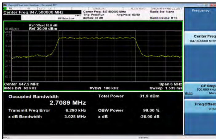
Band26_3MHz_64QAM_15_0_HighCH27025-847.5
