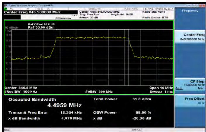
Band26_5MHz_16QAM_25_0_HighCH27015-846.5
