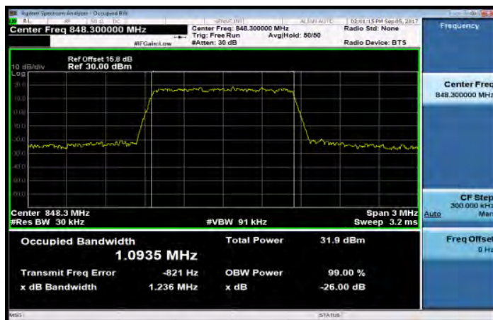
Band26_1_4MHz_QPSK_6_0_HighCH27033-848.3
