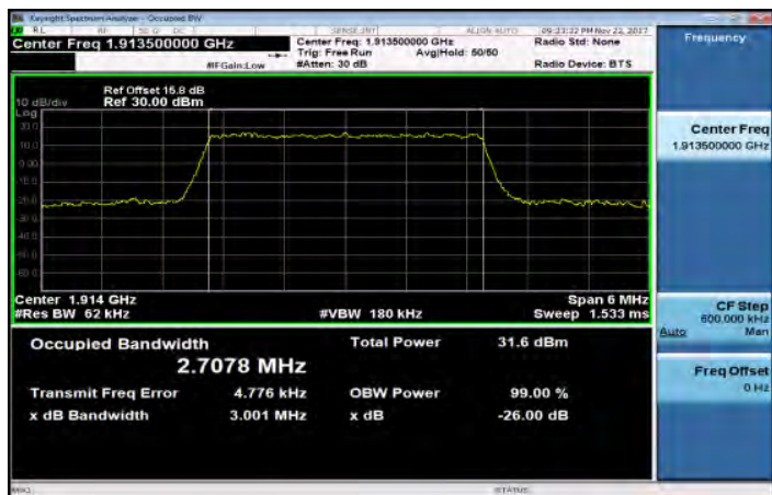
Band25_3MHz_64QAM_15_0_HighCH26675-1913.5
