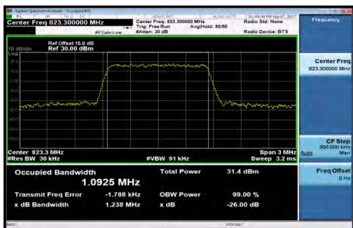
Part 90_Band26_1_4MHz_QPSK_6_0_HighCH26783
