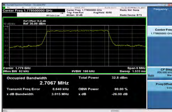
Band66_3MHz_64QAM_15_0_HighCH132657
