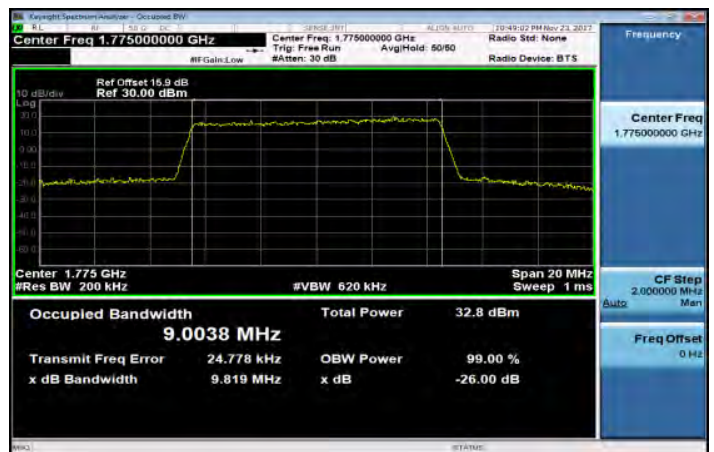
Band66_10MHz_64QAM_50_0_HighCH132622
