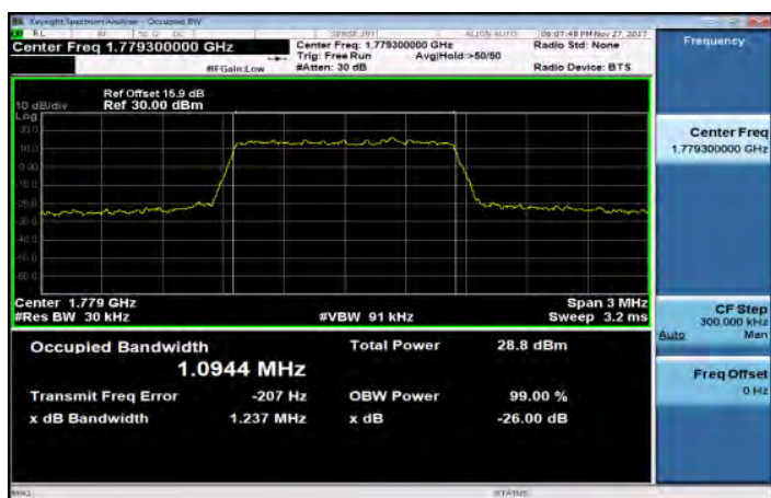
Band66_1_4MHz_64QAM_6_0_HighCH132665
