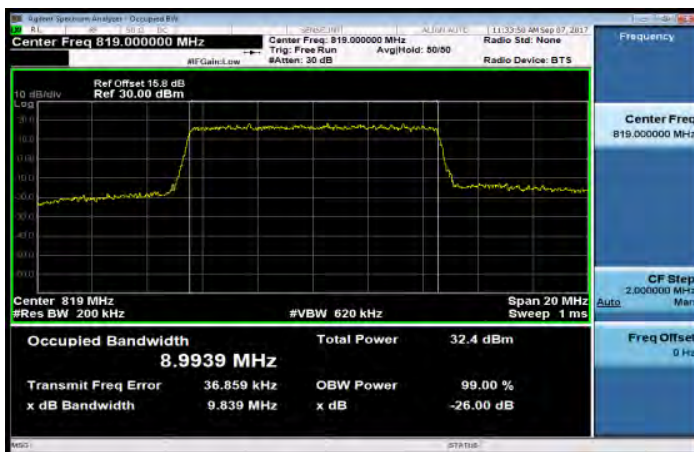
Part 90_Band26_10MHz_16QAM_50_0_MidCH26740
