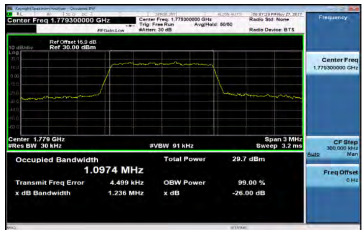
Band66_1_4MHz_16QAM_6_0_HighCH132665
