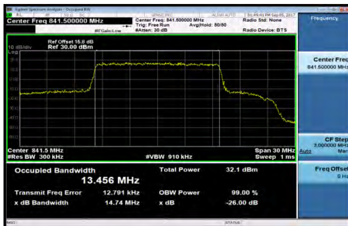
Band26_15MHz_QPSK_75_0_HighCH26965-841.5
