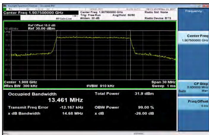
Band25_15MHz_16QAM_75_0_HighCH26615-1907.5
