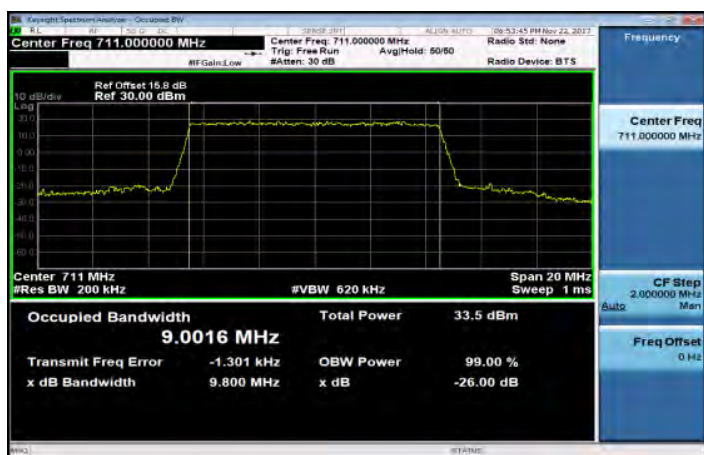
Band17_10MHz_QPSK_50_0_HighCH23800
