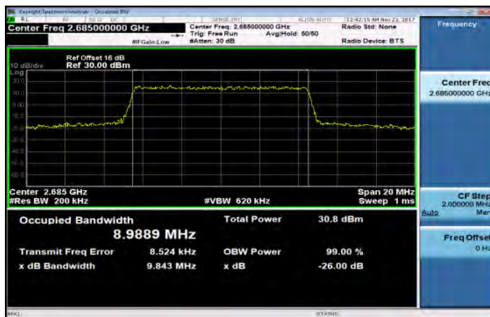
Band41_10MHz_64QAM_50_0_HighCH41540
