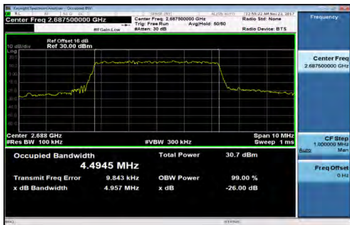
Band41_5MHz_64QAM_25_0_HighCH41565
