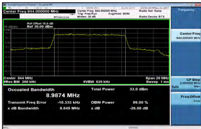
Band26_10MHz_64QAM_50_0_HighCH26990
