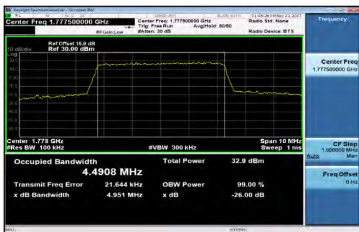
Band66_5MHz_64QAM_25_0_HighCH132647
