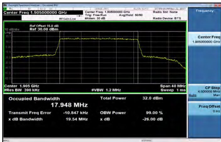
Band25_20MHz_64QAM_100_0_HighCH26590-1905
