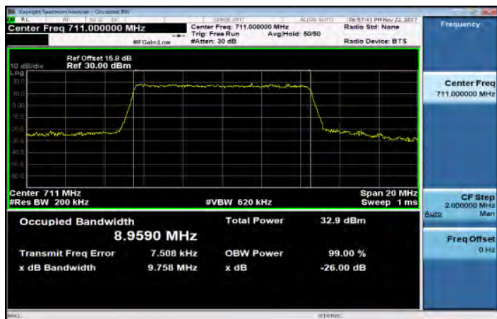
Band17_10MHz_64QAM_50_0_MidCH23790
