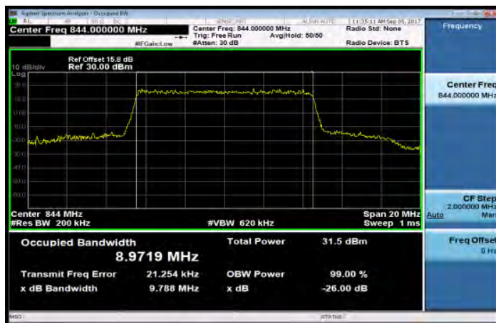
Band26_10MHz_16QAM_50_0_HighCH26990-844
