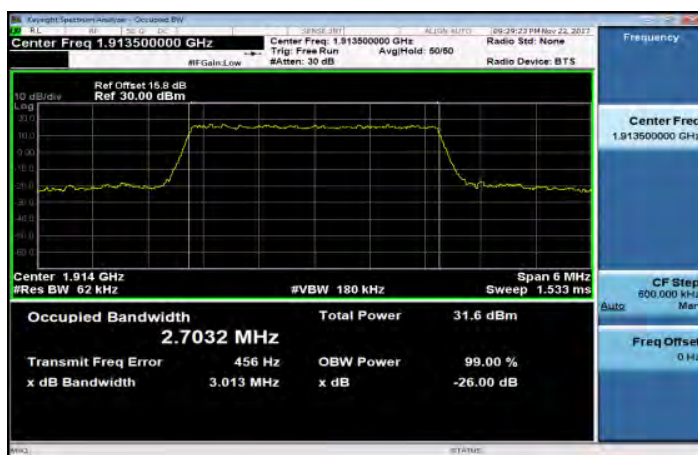
Band25_3MHz_16QAM_15_0_HighCH26675-1913.5
