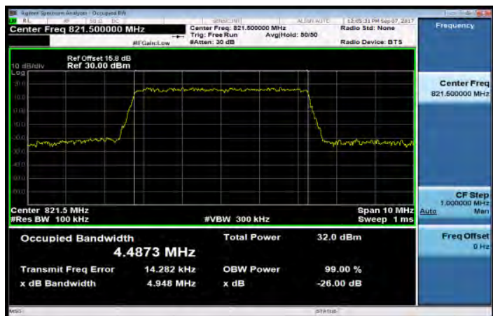
Part 90_Band26_5MHz_QPSK_25_0_HighCH26765
