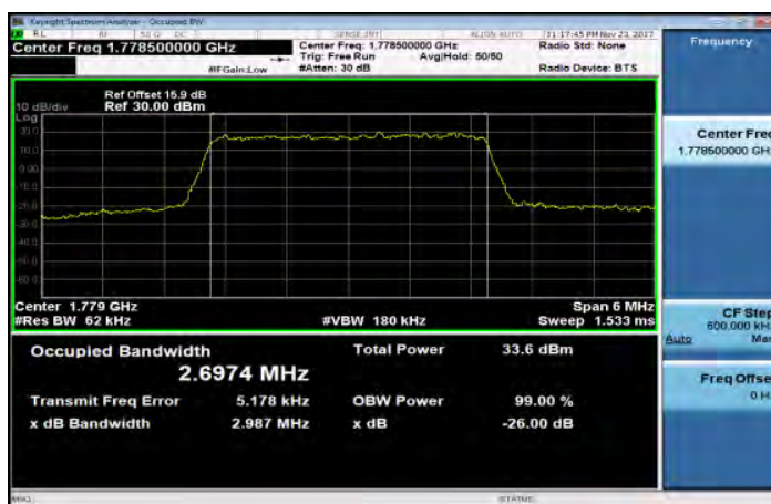
Band66_3MHz_QPSK_15_0_HighCH132657
