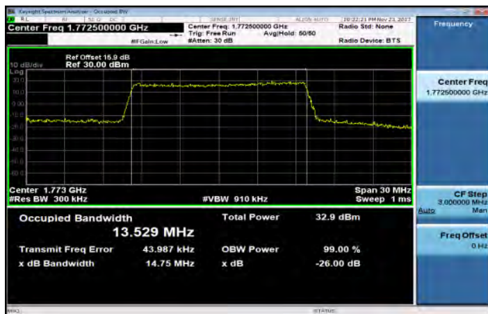
Band66_15MHz_64QAM_75_0_HighCH132597
