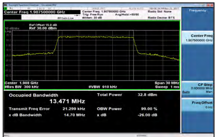
Band25_15MHz_QPSK_75_0_HighCH26615-1907.5
