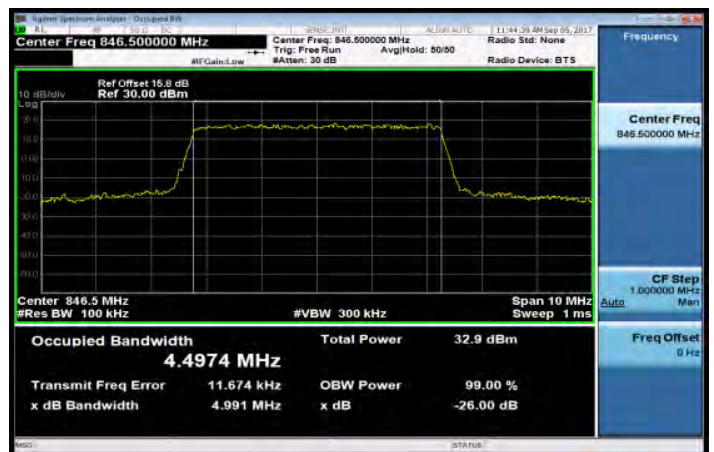
Band26_5MHz_QPSK_25_0_HighCH27015-846.5
