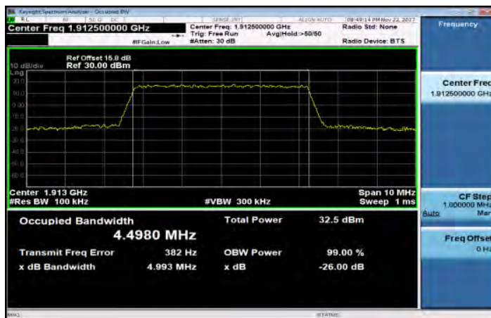
Band25_5MHz_QPSK_25_0_HighCH26665-1912.5
