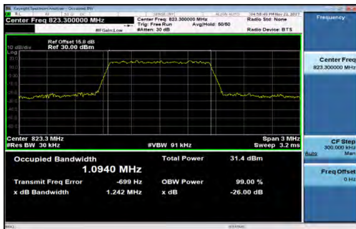
Part 90_Band26_1_4MHz_64QAM_6_0_HighCH26783
