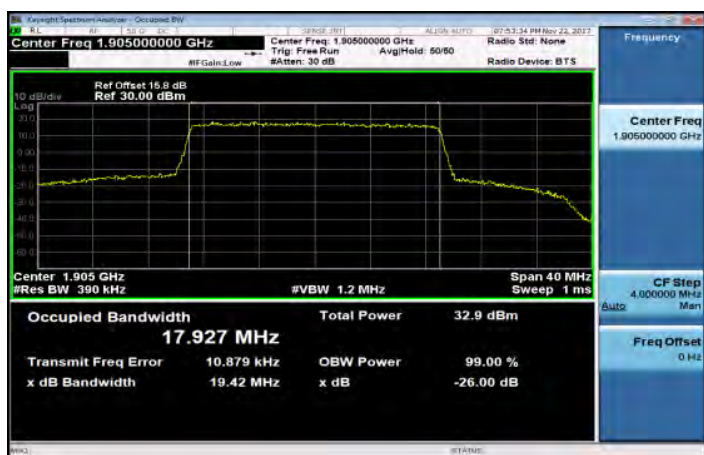
Band25_20MHz_QPSK_100_0_HighCH26590-1905
