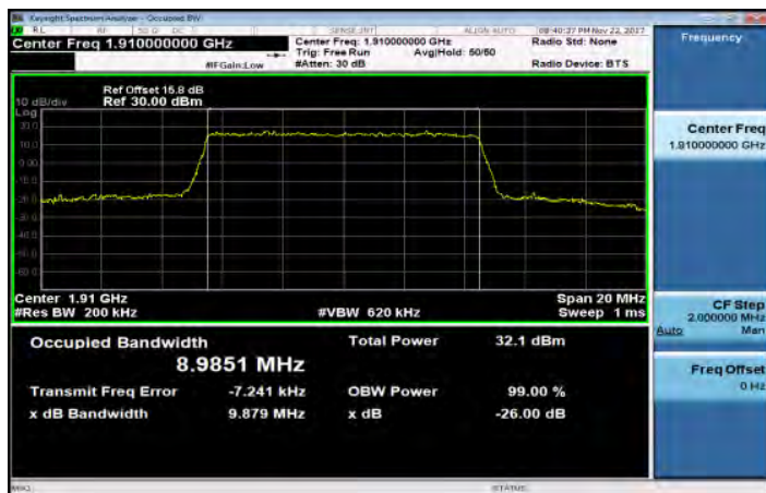
Band25_10MHz_64QAM_50_0_HighCH26640-1910
