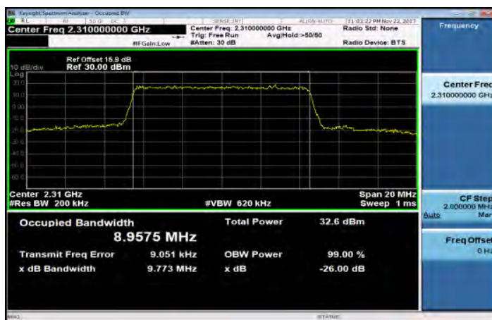
Band30_10MHz_64QAM_50_0_MidCH27710
