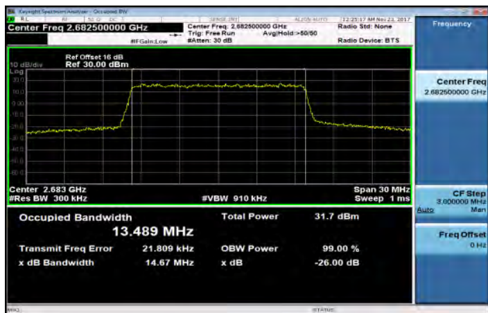
Band41_15MHz_QPSK_75_0_HighCH41515
