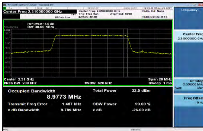
Band30_10MHz_64QAM_50_0_MidCH27710
