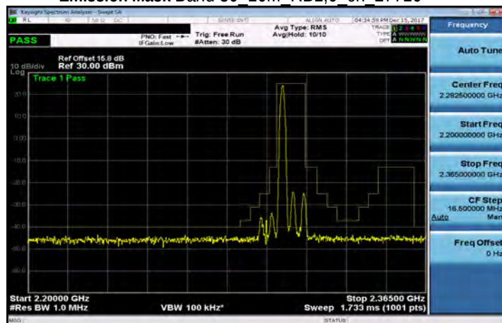
Emission Mask Band 30 10M RB1,0 ch 27710
