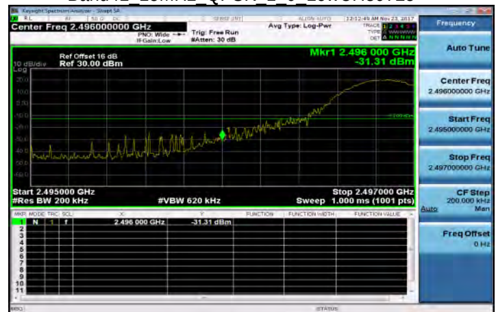
Band41 15MHz QPSK 1 0 LowCH39725
