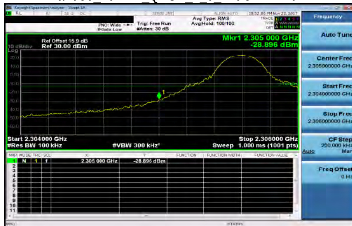
Band30 10MHz QPSK 1 0 MidCH27710
