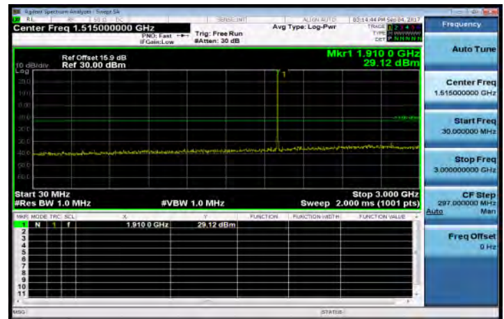
30MHz~3GHz_Band2_3MHz_QPSK_1_0_HighCH19185-1908.5
