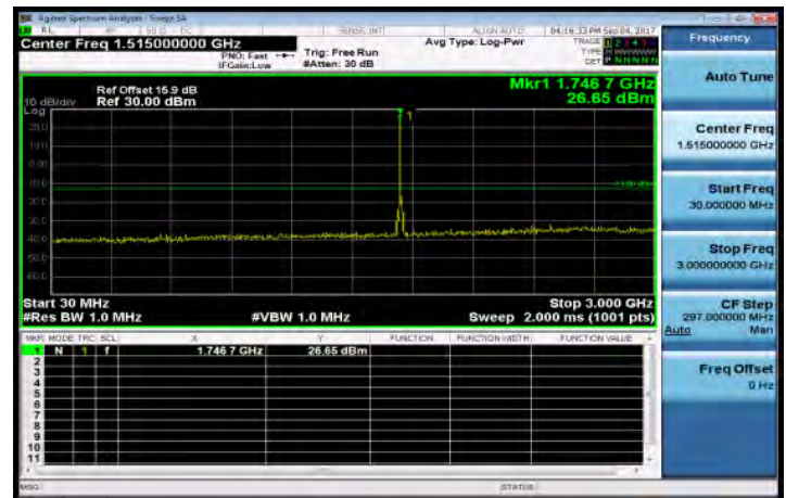
30MHz~3GHz_Band4_10MHz_QPSK_1_0_HighCH20350-1750
