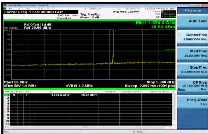
30MHz~3GHz_Band2_15MHz_QPSK_1_0_MidCH18900-1880
