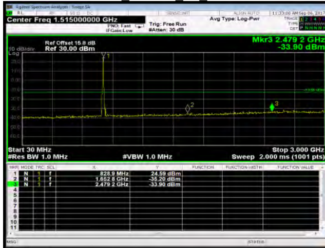
30MHz~3GHz HSDPA B5 LowCH4132-826.4
