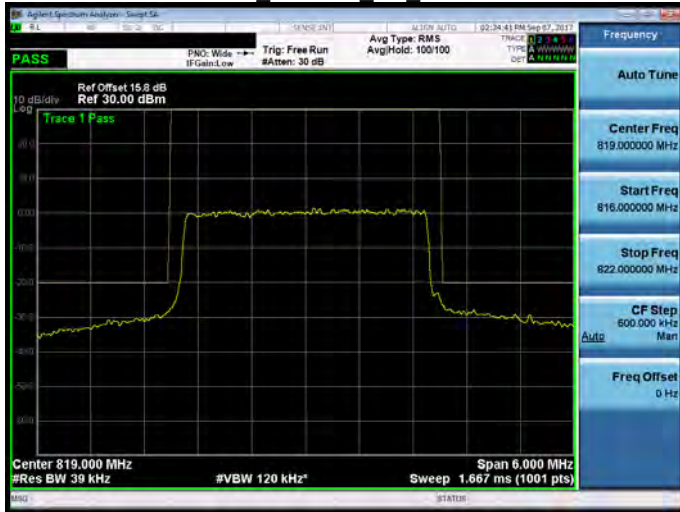
Part 90 Band 26 3M 1RB0
