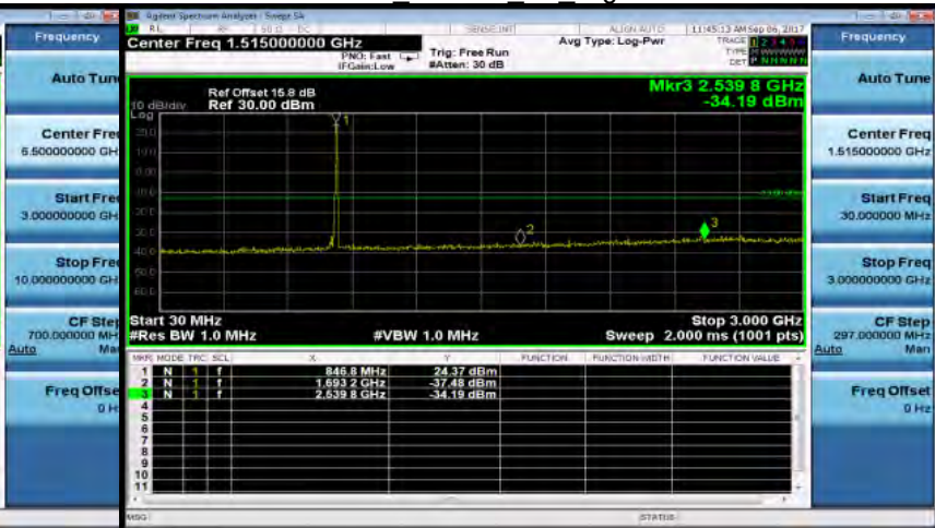
30MHz~3GHz HSUPA B5 HighCH4233-846.6
