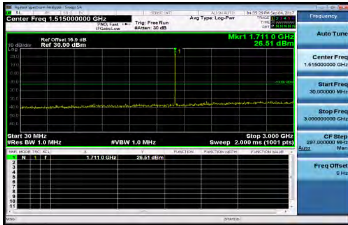
30MHz-3GHz_Band4_3MHz_QPSK_1_0_LowCH19965-1711.5
