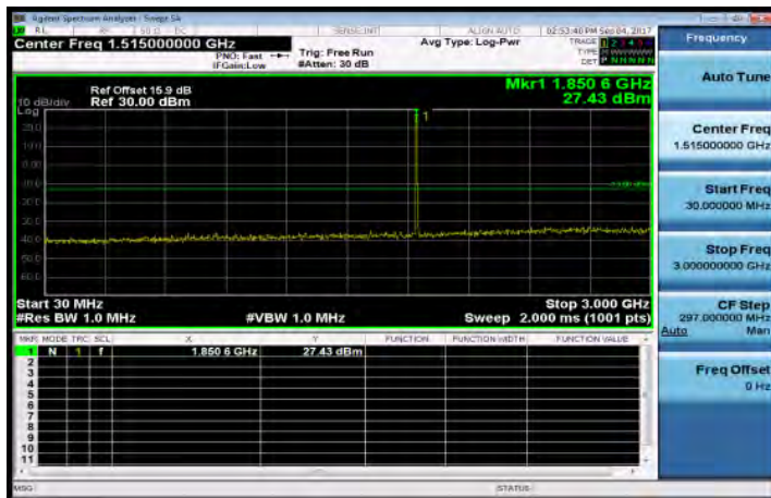
30MHz~3GHz_Band2_5MHz_QPSK_1_0_LowCH18625-1852.5
