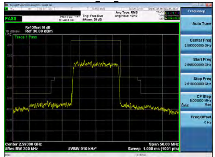
Band 41 15M RB75,0
