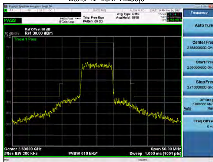
Band 41 10M RB50,0
