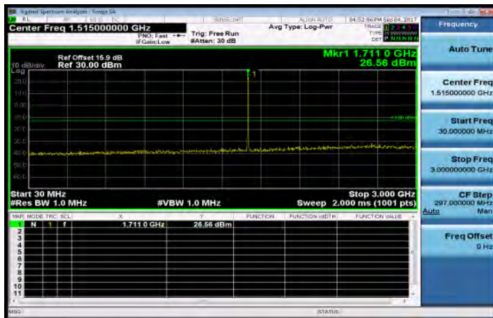
30MHz~3GHz_Band4_1_4MHz_QPSK_1_0_LowCH19957-1710.7
