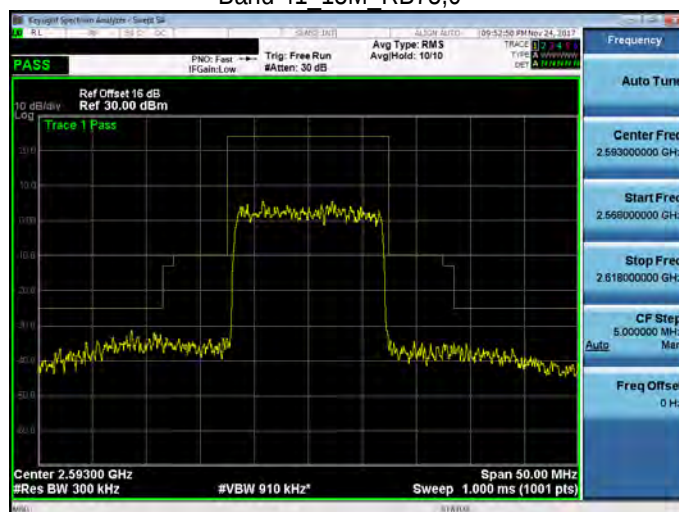
Band 41 15M RB75,0
