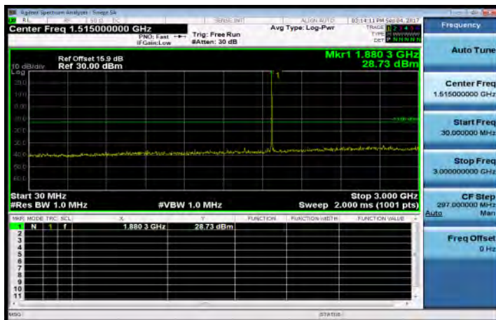
30MHz~3GHz_Band2_3MHz_QPSK_1_0_MidCH18900-1880
