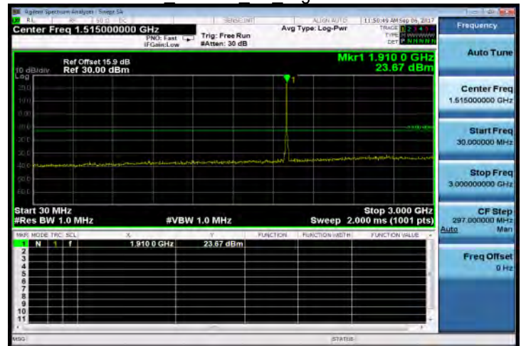
30MHz~3GHz HSUPA B2 HighCH9538-1907.6
