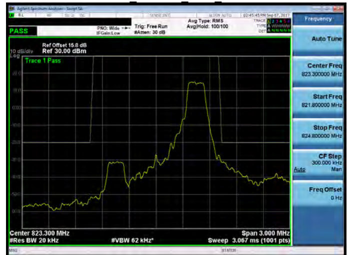
Part 90 Band 26 1.4M 6RB0
