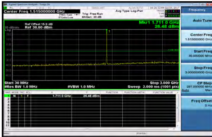
30MHz-3GHz_Band4_5MHz_QPSK_1_0_LowCH19975-1712.5
