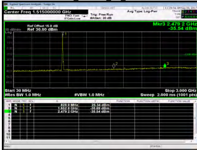
30MHz~3GHz HSUPA B5 LowCH4132-826.4
