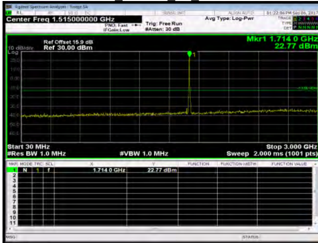
30MHz~3GHz HSUPA B4 LowCH1312-1712.4
