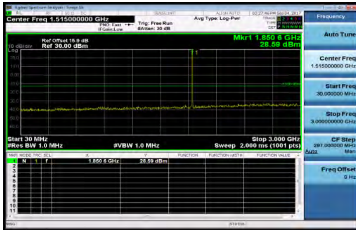
30MHz-3GHz_Band2_1_4MHz_QPSK_1_0_LowCH18607-1850.7
