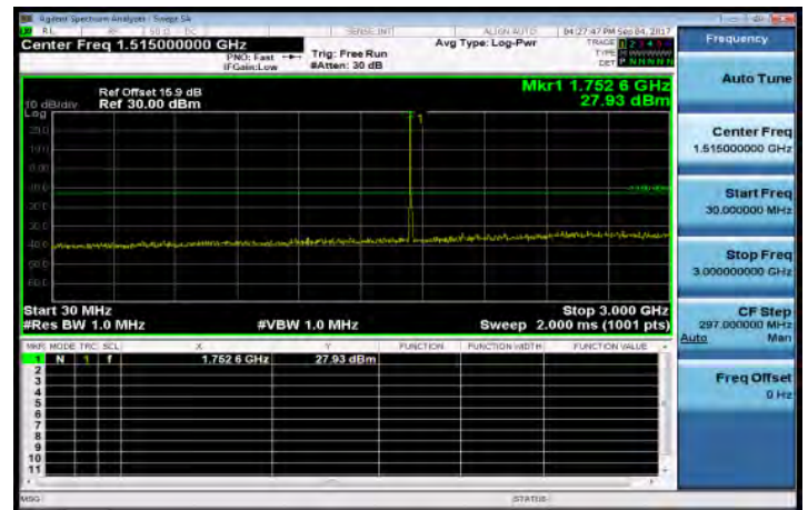
30MHz-3GHz_Band4_5MHz_QPSK_1_0_HighCH20375-1752.5
