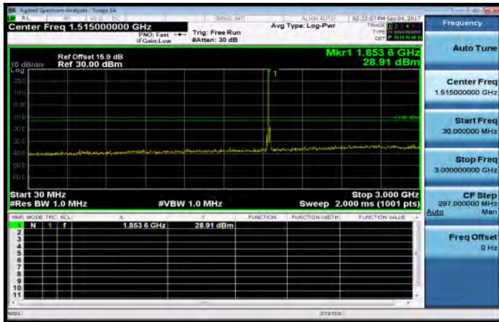
30MHz~3GHz_Band2_15MHz_QPSK_1_0_LowCH18675-1857.5
