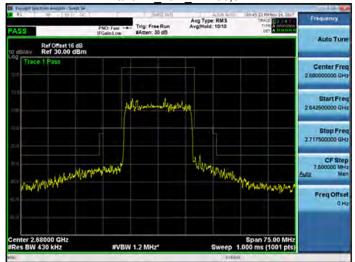
Band 41 20M RB100,0
