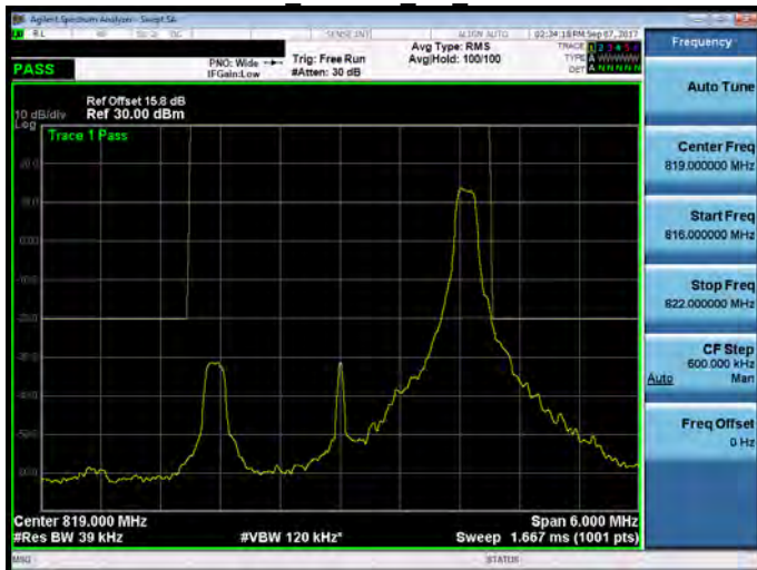
Part 90 Band 26 3M 1RB14
