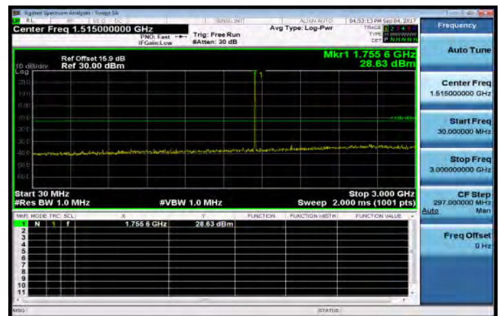
30MHz~3GHz_Band4_1_4MHz_QPSK_1_0_HighCH20393-1754.3
