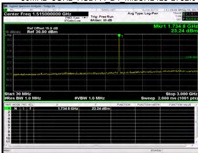
30MHz~3GHz HSDPA B4 MidCH1413-1732.6
