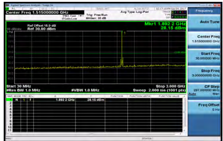
30MHz~3GHz_Band2_20MHz_QPSK_1_0_HighCH19100-1900
