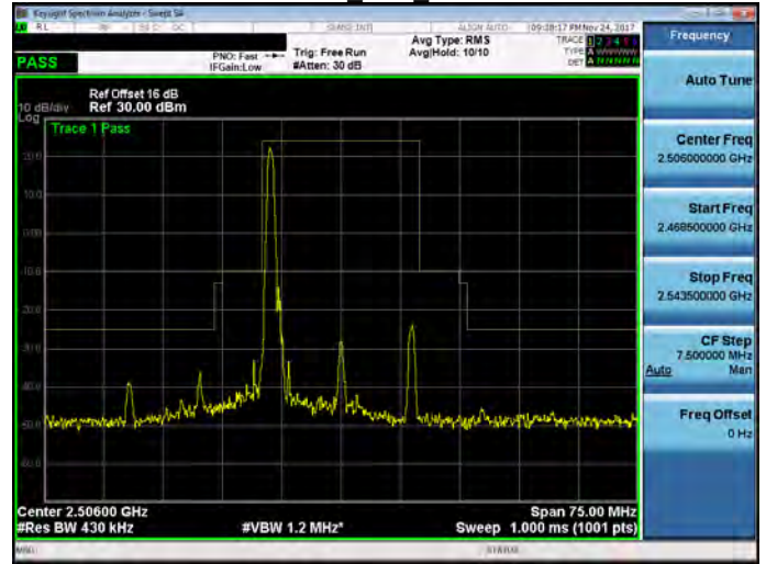
Band 41 20M RB1,99
