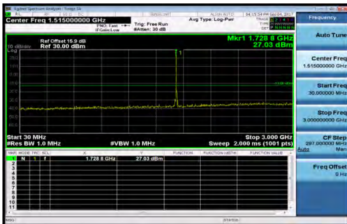
30MHz~3GHz_Band4_10MHz_QPSK_1_0_MidCH20175-1732.5
