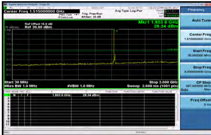
30MHz~3GHz_Band2_20MHz_QPSK_1_0_LowCH18700-1860
