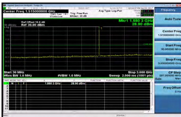
30MHz~3GHz_Band2_5MHz_QPSK_1_0_MidCH18900-1880
