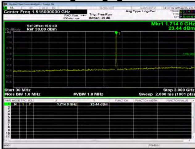
30MHz~3GHz HSDPA B4 LowCH1312-1712.4
