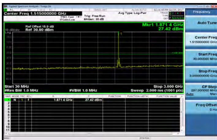
30MHz~3GHz_Band2_20MHz_QPSK_1_0_MidCH18900-1880
