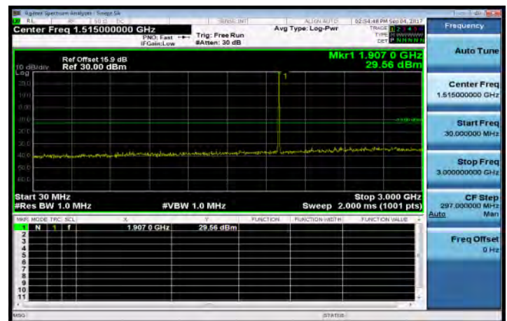
30MHz~3GHz_Band2_5MHz_QPSK_1_0_HighCH19175-1907.5
