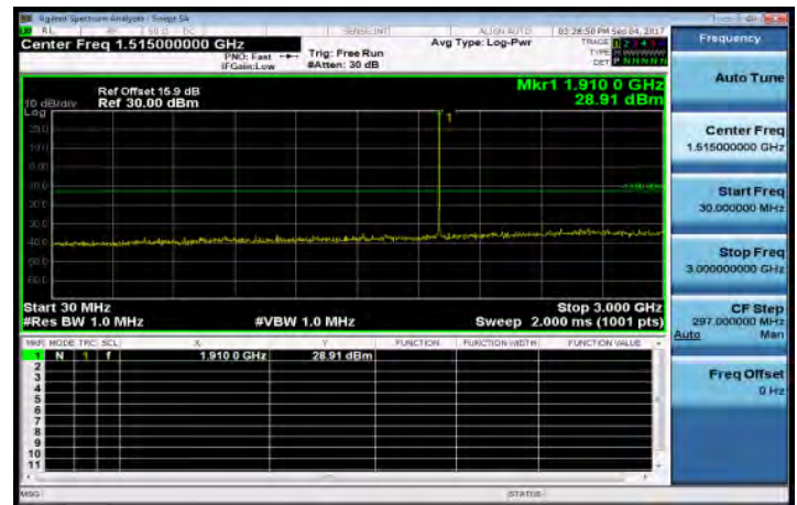
30MHz-3GHz_Band2_1_4MHz_QPSK_1_0_HighCH19193-1909.3
