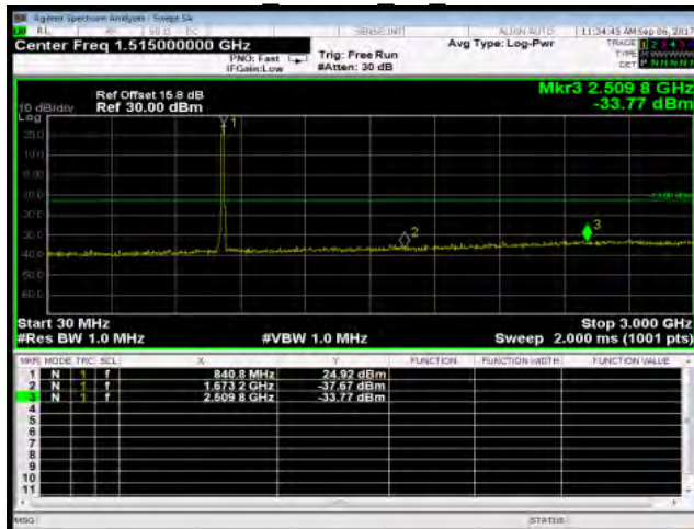
30MHz~3GHz HSDPA B5 MidCH4183-836.6
