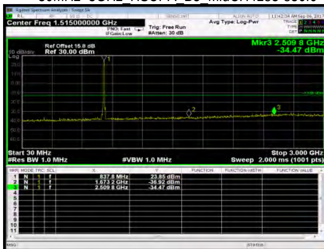
30MHz~3GHz HSUPA B5 MidCH4183-836.6
