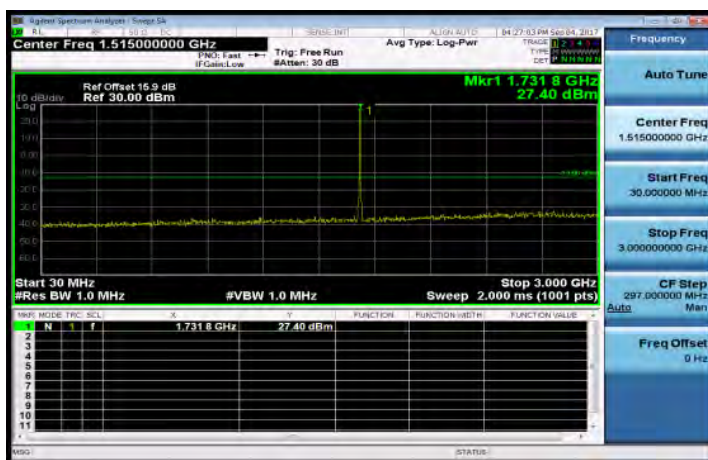
30MHz-3GHz_Band4_5MHz_QPSK_1_0_MidCH20175-1732.5
