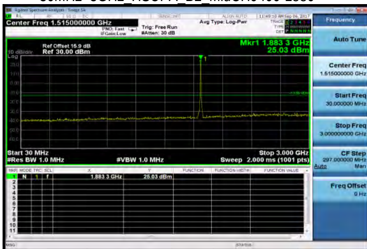
30MHz~3GHz HSUPA B2 MidCH9400-1880
