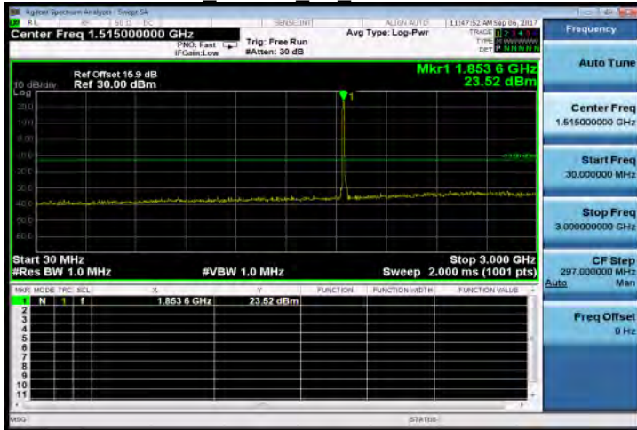
30MHz~3GHz HSUPA B2 LowCH9262-1852.4
