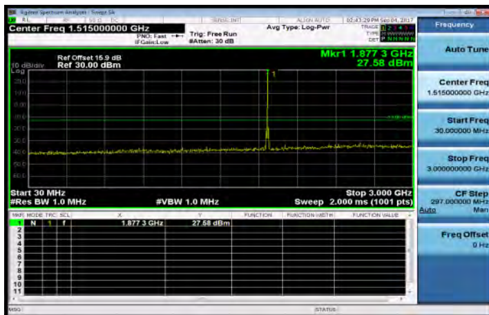
30MHz~3GHz_Band2_10MHz_QPSK_1_0_MidCH18900-1880
