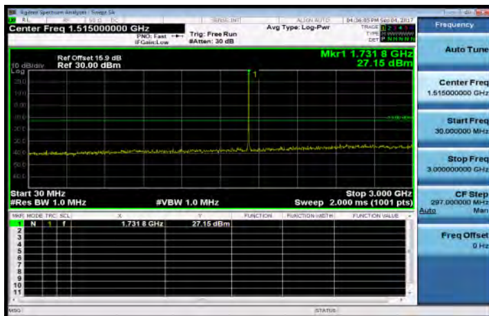
30MHz-3GHz_Band4_3MHz_QPSK_1_0_MidCH20175-1732.5
