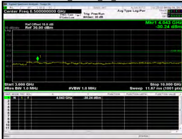
3GHz~10GHz HSDPA B5 LowCH4132-826.4
