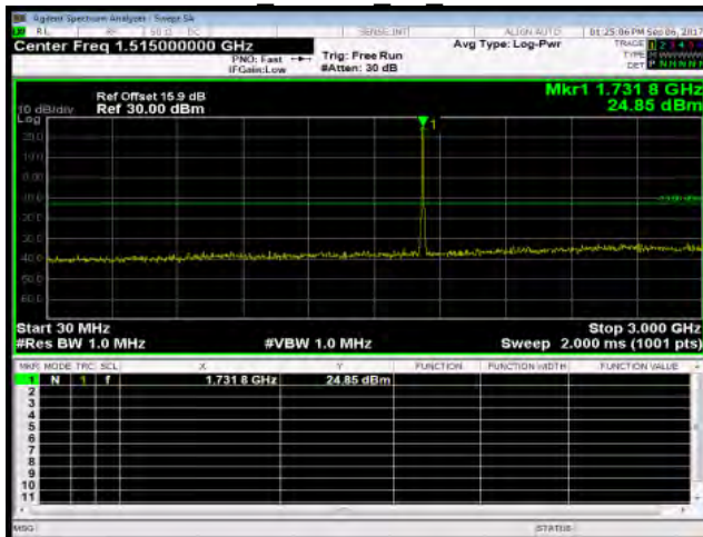
30MHz~3GHz HSUPA B4 MidCH1413-1732.6
