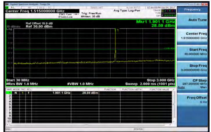
30MHz~3GHz_Band2_10MHz_QPSK_1_0_HighCH19150-1905
