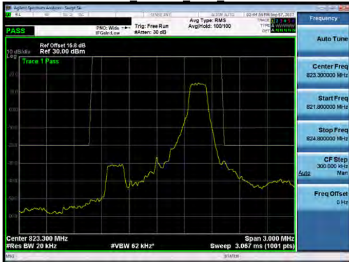
Part 90 Band 26 1.4M 6RB0
