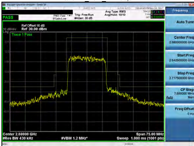
Band 41 20M RB100,0
