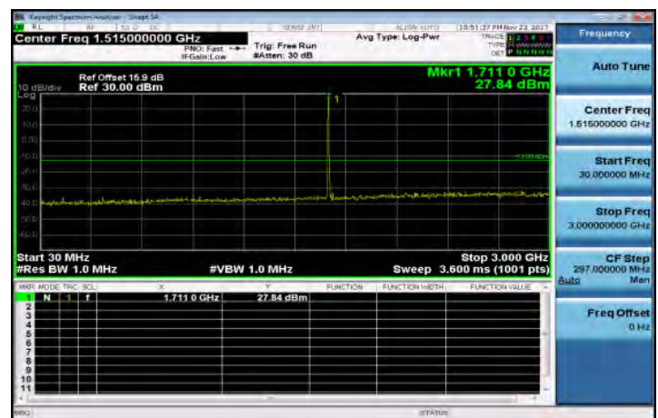
30MHz~3GHz_Band66_5MHz_QPSK_1_0_LowCH131997
