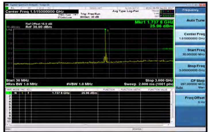
30MHz~3GHz_Band4_20MHz_QPSK_1_0_HighCH20300-1745
