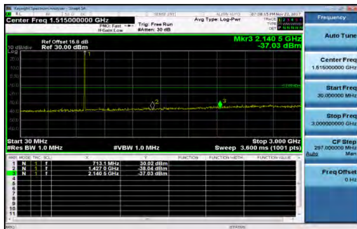
30MHz-3GHz_Band17_5MHz_QPSK_1_0_HighCH23825-713.5
