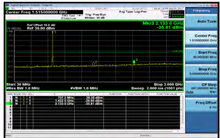
30MHz~3GHz_Band12_10MHz_QPSK_1_0_HighCH23130-711
