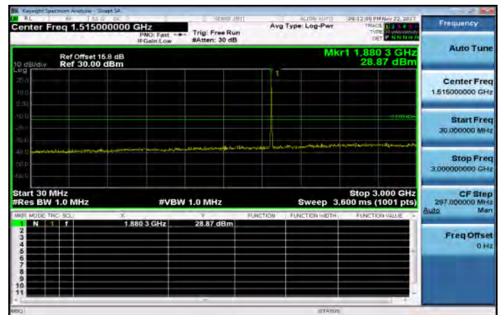
30MHz~3GHz_Band25_5MHz_QPSK_1_0_MidCH26365-1882.5
