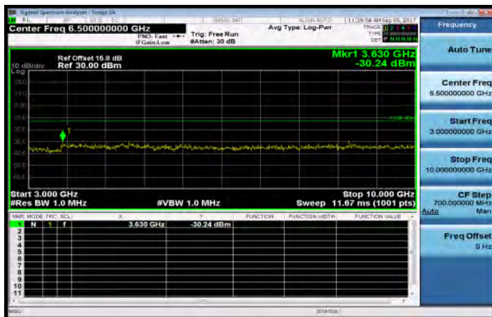
3GHz~10GHz_Band26_10MHz_QPSK_1_0_HighCH26990-844
