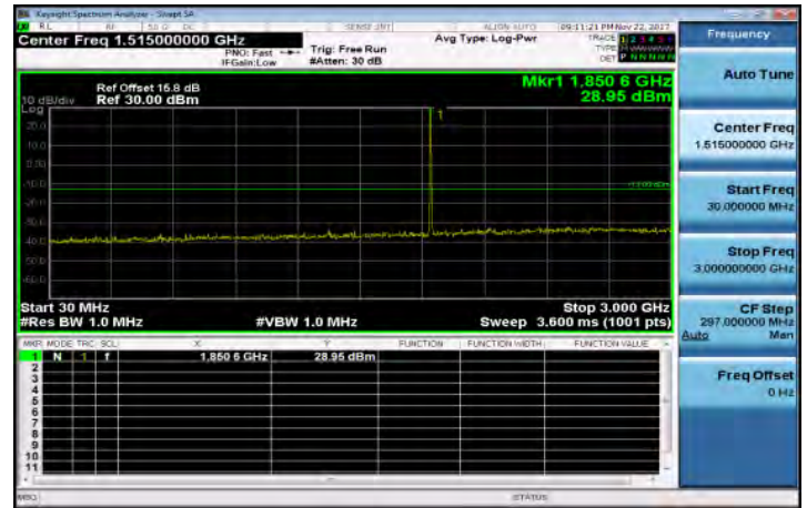
30MHz~3GHz_Band25_5MHz_QPSK_1_0_LowCH26065-1852.5
