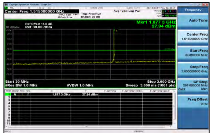
30MHz~3GHz_Band25_15MHz_QPSK_1_0_MidCH26365-1882.5
