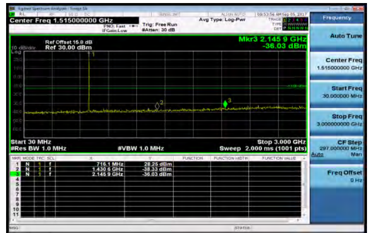
30MHz~3GHz_Band12_1_4MHz_QPSK_1_0_HighCH23173-715.3
