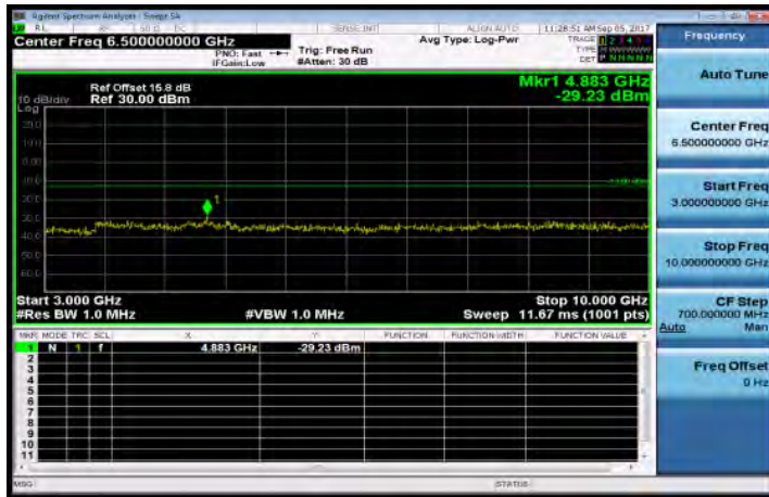
3GHz~10GHz_Band26_10MHz_QPSK_1_0_MidCH26865-831.5
