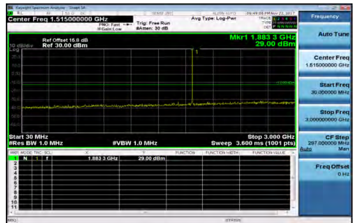
30MHz~3GHz_Band25_1_4MHz_QPSK_1_0_MidCH26365-1882.5
