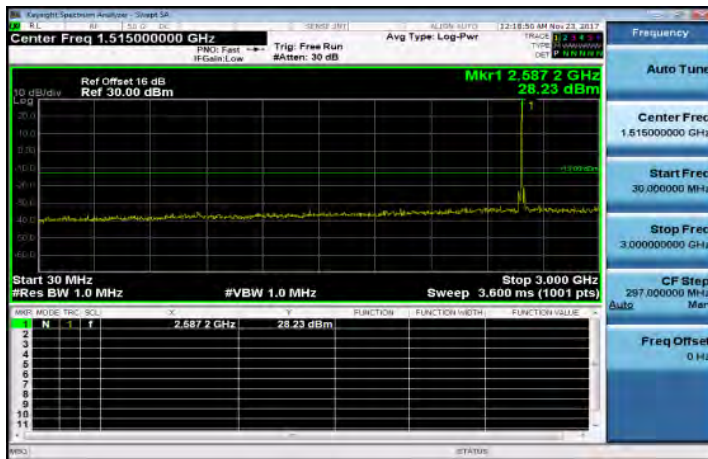
30MHz~3GHz_Band41_15MHz_QPSK_1_0_MidCH40620
