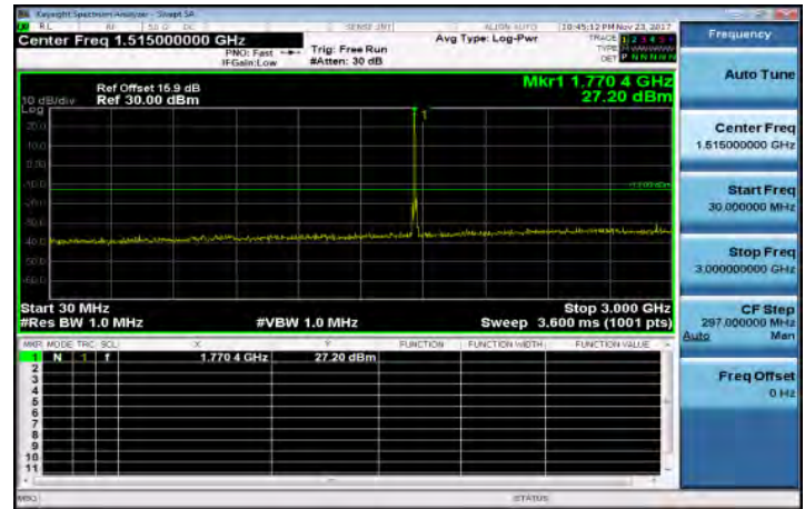
30MHz~3GHz_Band66_10MHz_QPSK_1_0_HighCH132622
