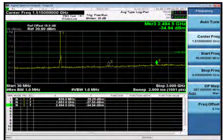
30MHz~3GHz_Band26_15MHz_QPSK_1_0_MidCH26865-831.5
