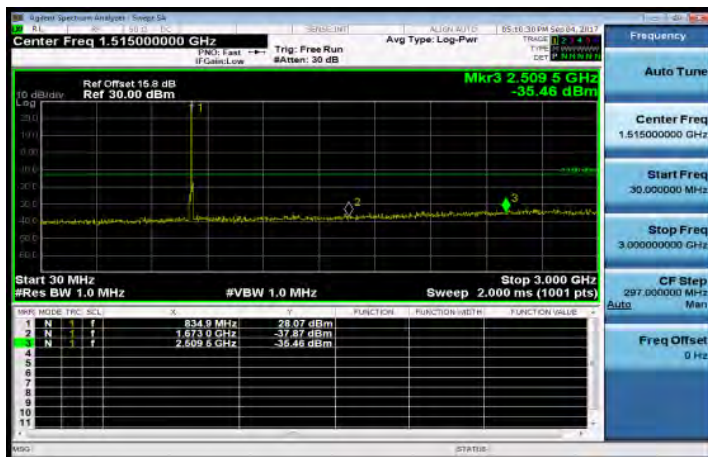
30MHz~3GHz_Band5_10MHz_QPSK_1_0_MidCH20525-836.5
