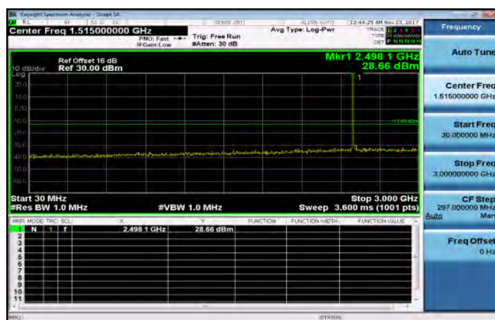
30MHz~3GHz_Band41_5MHz_QPSK_1_0_LowCH39675
