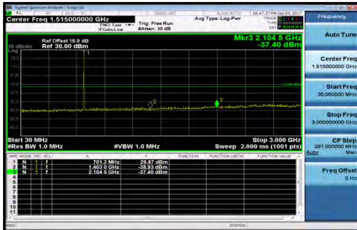
30MHz-3GHz_Band12_5MHz_QPSK_1_0_LowCH23035-701.5
