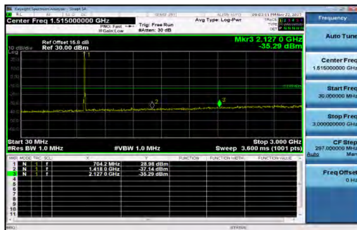
30MHz-3GHz_Band17_10MHz_QPSK_1_0_LowCH23780-709
