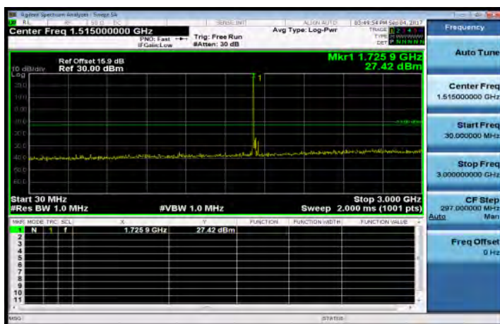
30MHz~3GHz_Band4_20MHz_QPSK_1_0_MidCH20175-1732.5
