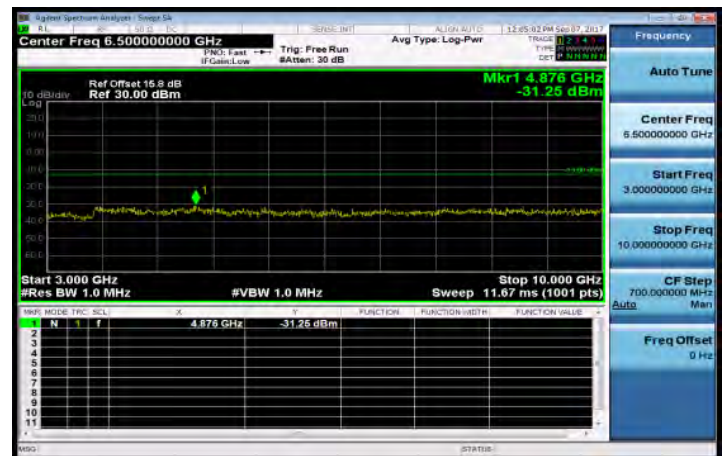
3GHz~10GHz_Band26_5MHz_QPSK_1_0_HighCH26765
