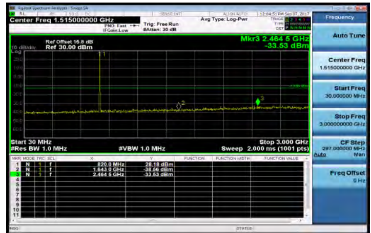
30MHz~3GHz_Band26_5MHz_QPSK_1_0_HighCH26765
