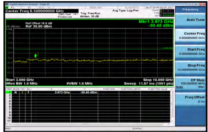
3GHz~10GHz_Band5_5MHz_QPSK_1_0_MidCH20525-836.5
