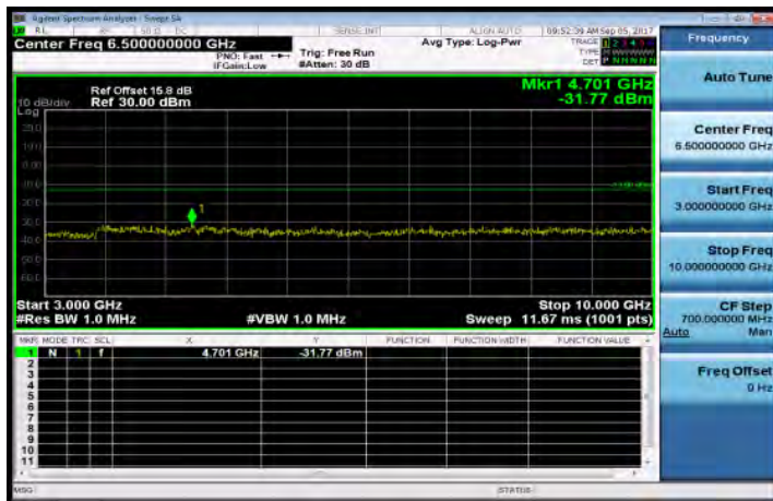
3GHz~10GHz_Band12_1_4MHz_QPSK_1_0_LowCH23017-699.7
