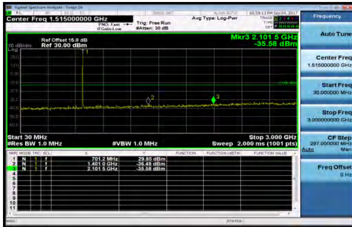
30MHz-3GHz_Band12_3MHz_QPSK_1_0_LowCH23025-700.5
