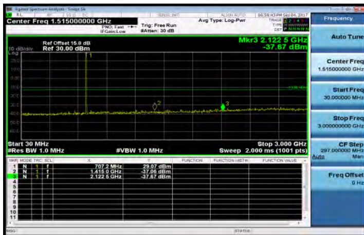
30MHz-3GHz_Band12_3MHz_QPSK_1_0_MidCH23095-707.5
