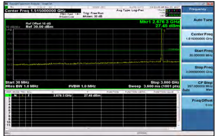
30MHz~3GHz_Band41_15MHz_QPSK_1_0_HighCH41515
