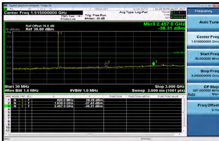
30MHz-3GHz_Band26_3MHz_QPSK_1_0_MidCH26740
