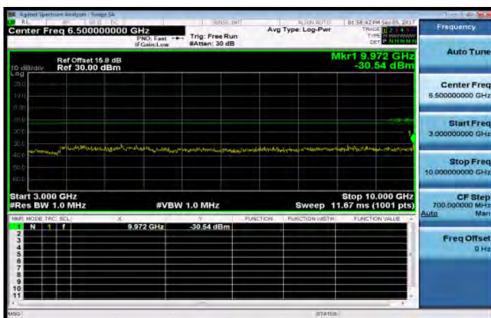
3GHz~10GHz_Band26_1_4MHz_QPSK_1_0_HighCH27033-848.3
