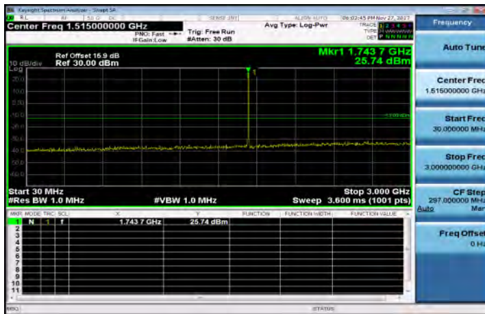
30MHz-3GHz_Band66_1_4MHz_QPSK_1_0_MidCH132322
