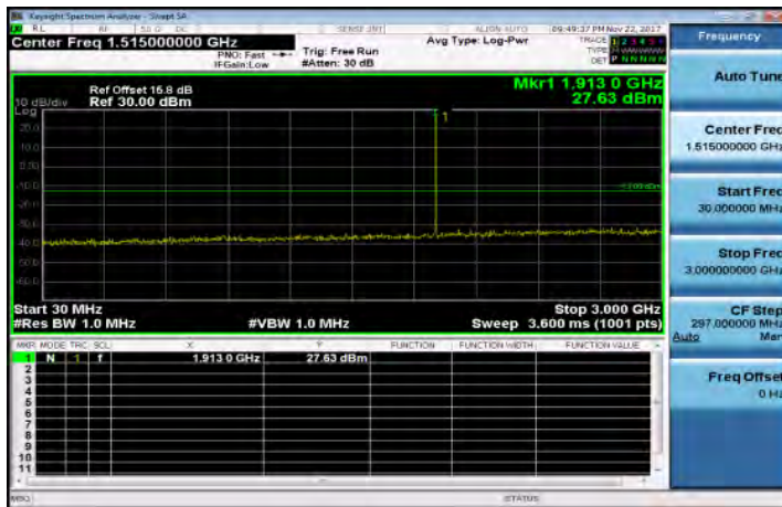
30MHz~3GHz_Band25_1_4MHz_QPSK_1_0_HighCH26683-1914.3
