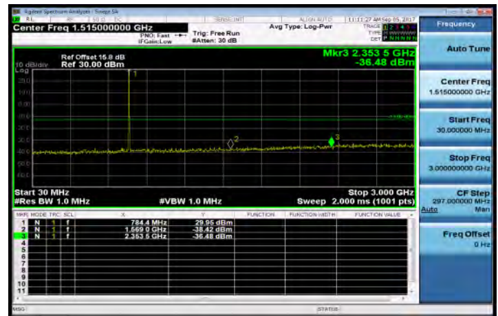
30MHz~3GHz_Band13_5MHz_QPSK_1_0_HighCH23255-784.5
