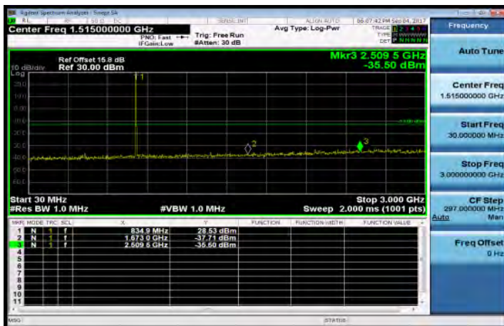
30MHz~3GHz_Band5_5MHz_QPSK_1_0_MidCH20525-836.5
