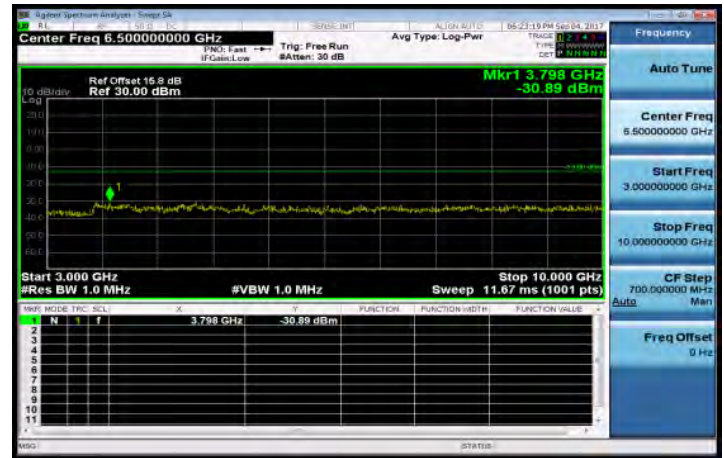
3GHz~10GHz_Band5_3MHz_QPSK_1_0_MidCH20525-836.5
