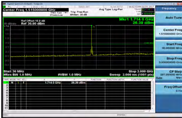
30MHz~3GHz_Band4_15MHz_QPSK_1_0_LowCH20025-1717.5
