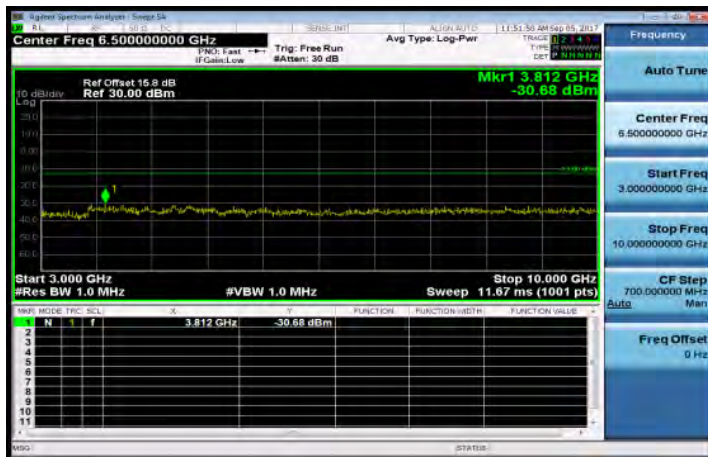
3GHz~10GHz_Band26_3MHz_QPSK_1_0_MidCH26865-831.5
