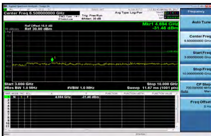
3GHz~10GHz_Band26_3MHz_QPSK_1_0_HighCH27025-847.5
