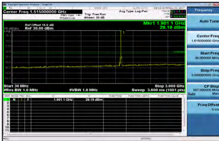
30MHz~3GHz_Band25_15MHz_QPSK_1_0_HighCH26615-1907.5
