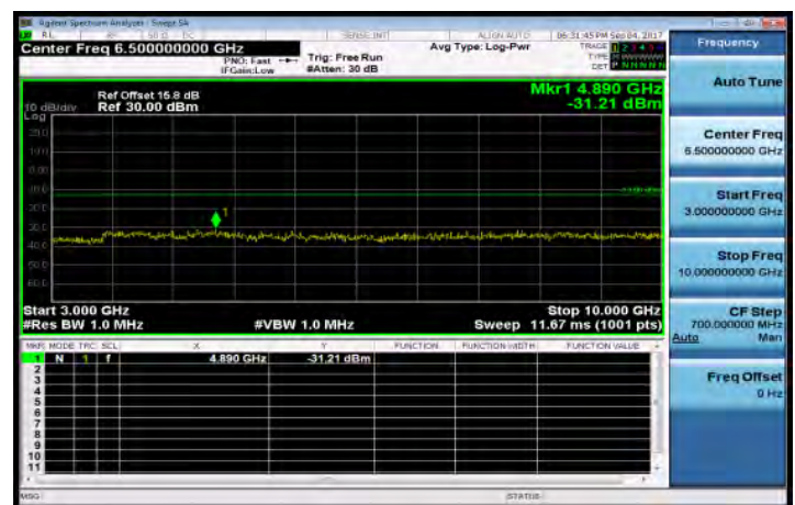
3GHz~10GHz_Band5_1_4MHz_QPSK_1_0_HighCH20643-848.3
