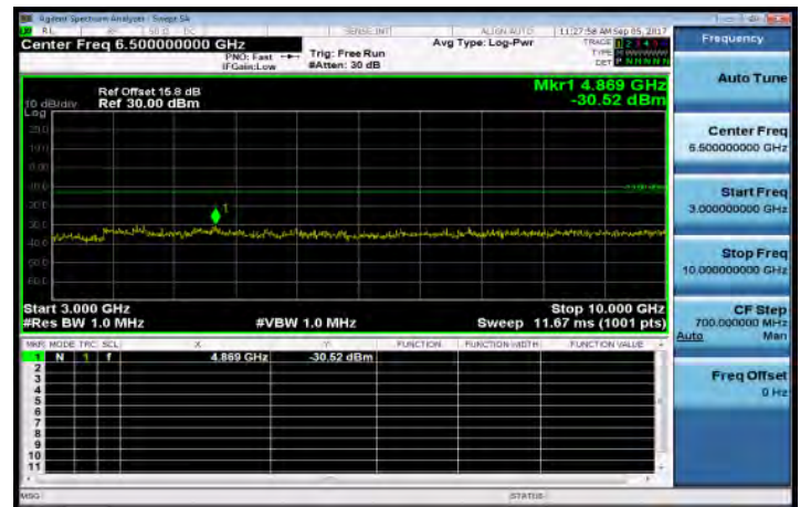
3GHz~10GHz_Band26_10MHz_QPSK_1_0_LowCH26750-820
