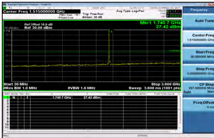
30MHz~3GHz_Band66_10MHz_QPSK_1_0_MidCH132322
