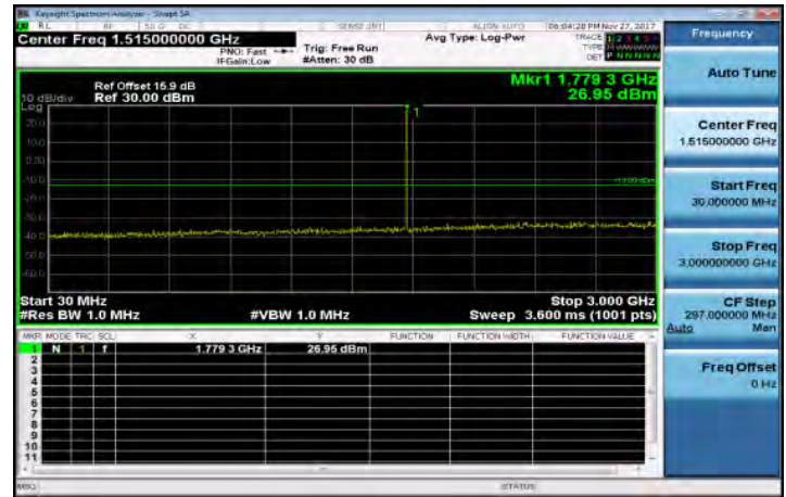
30MHz-3GHz_Band66_1_4MHz_QPSK_1_0_HighCH132665
