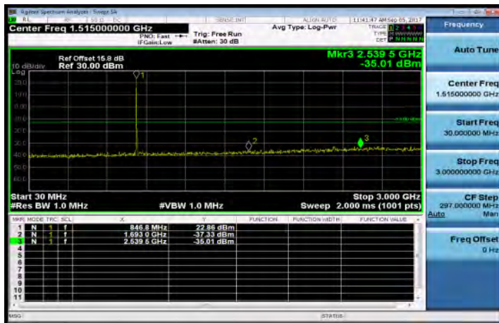
30MHz~3GHz_Band26_5MHz_QPSK_1_0_HighCH27015-846.5
