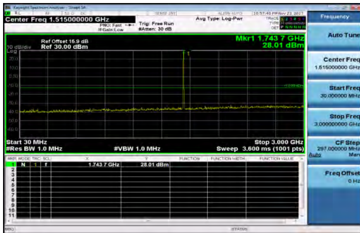
30MHz~3GHz_Band66_5MHz_QPSK_1_0_MidCH132322
