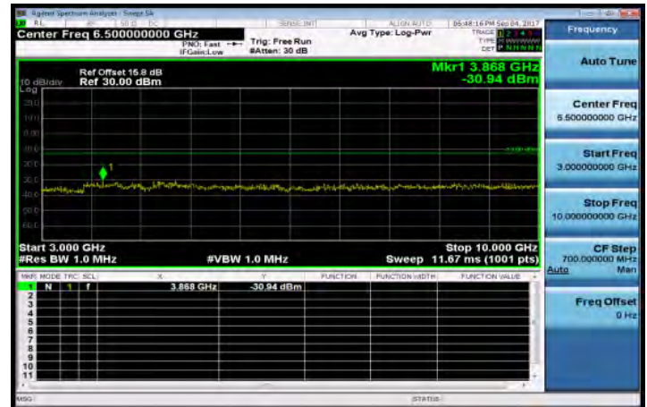
3GHz-10GHz_Band12_5MHz_QPSK_1_0_MidCH23095-707.5
