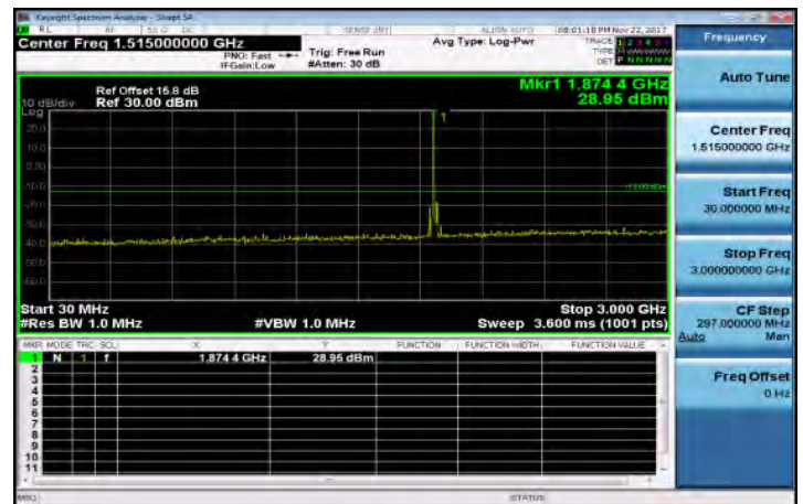
30MHz~3GHz_Band25_20MHz_QPSK_1_0_MidCH26365-1882.5
