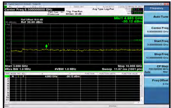
3GHz~10GHz_Band26_3MHz_QPSK_1_0_LowCH26705-815.5
