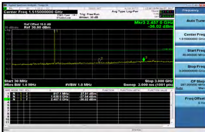
30MHz~3GHz_Band26_5MHz_QPSK_1_0_MidCH26740
