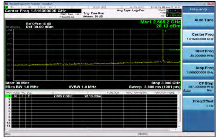
30MHz~3GHz_Band41_5MHz_QPSK_1_0_HighCH41565
