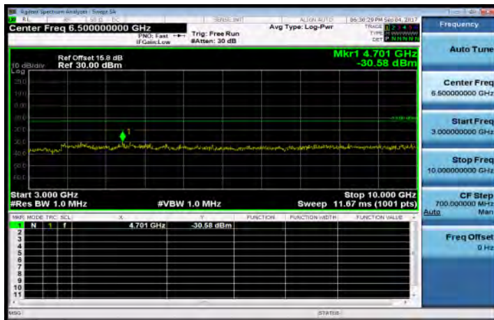
3GHz~10GHz_Band5_1_4MHz_QPSK_1_0_LowCH20407-824.7
