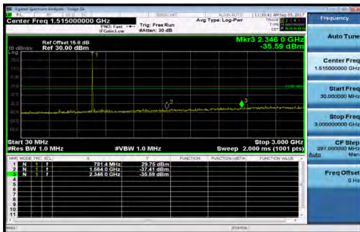
30MHz~3GHz_Band13_5MHz_QPSK_1_0_MidCH23230-782
