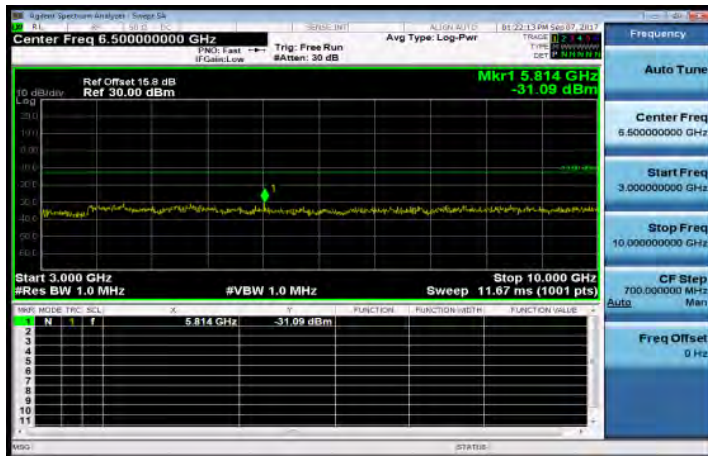
3GHz-10GHz_Band26_3MHz_QPSK_1_0_LowCH26705
