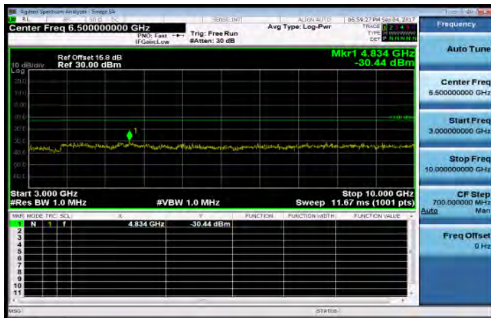
3GHz-10GHz_Band12_3MHz_QPSK_1_0_LowCH23025-700.5
