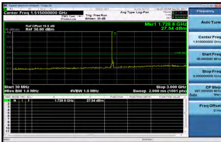
30MHz~3GHz_Band4_15MHz_QPSK_1_0_MidCH20175-1732.5
