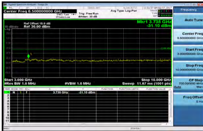
3GHz~10GHz_Band26_5MHz_QPSK_1_0_LowCH26715
