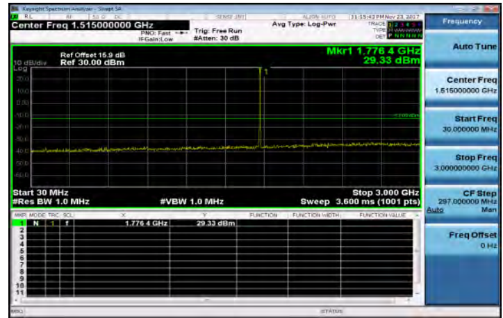
30MHz~3GHz_Band66_3MHz_QPSK_1_0_HighCH132657
