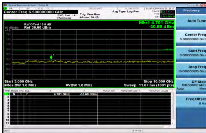
3GHz~10GHz_Band26_15MHz_QPSK_1_0_HighCH26965-841.5
