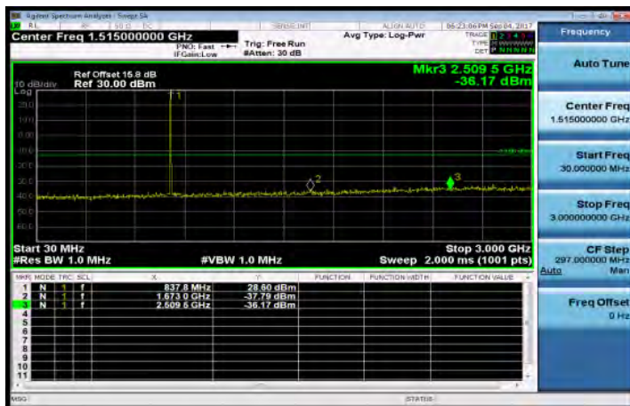
30MHz~3GHz_Band5_3MHz_QPSK_1_0_MidCH20525-836.5
