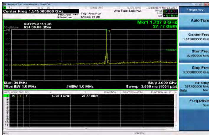
30MHz~3GHz_Band66_20MHz_QPSK_1_0_MidCH132322
