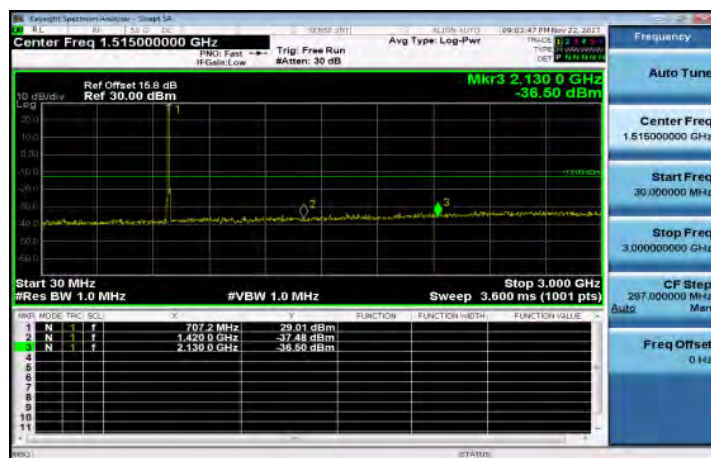
30MHz-3GHz_Band17_10MHz_QPSK_1_0_MidCH23790-710
