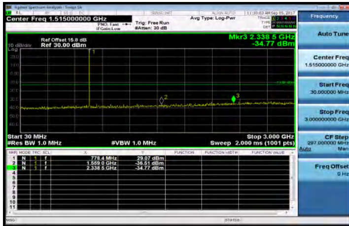
30MHz~3GHz_Band13_5MHz_QPSK_1_0_LowCH23205-779.5
