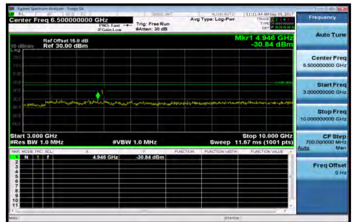
3GHz~10GHz_Band13_5MHz_QPSK_1_0_HighCH23255-784.5
