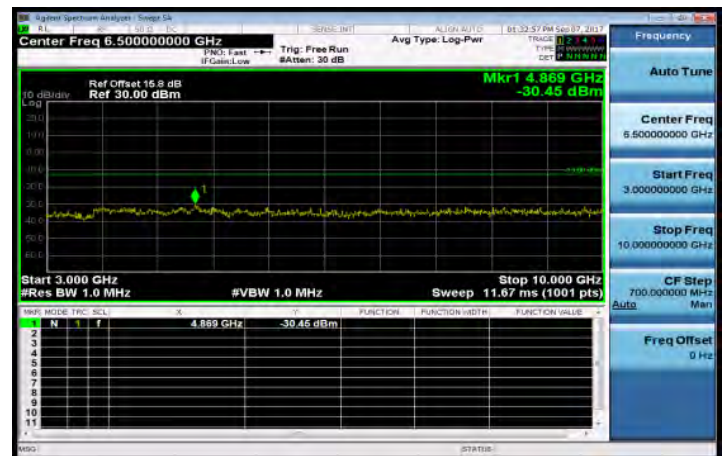
3GHz-10GHz_Band26_3MHz_QPSK_1_0_HighCH26775
