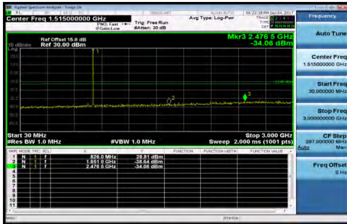
30MHz~3GHz_Band5_3MHz_QPSK_1_0_LowCH20415-825.5
