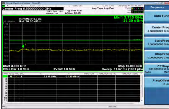
3GHz~10GHz_Band17_10MHz_QPSK_1_0_MidCH23790-710
