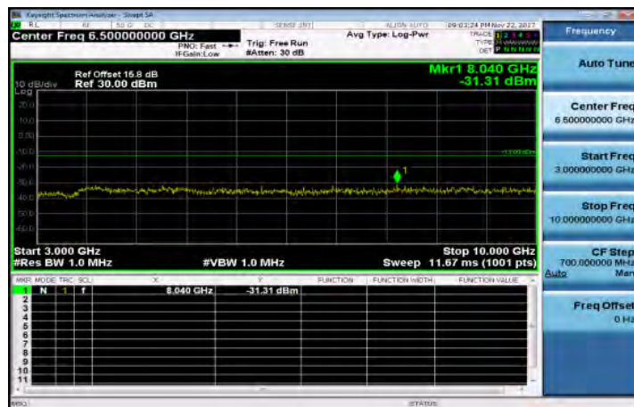
3GHz-10GHz_Band17_10MHz_QPSK_1_0_LowCH23780-709
