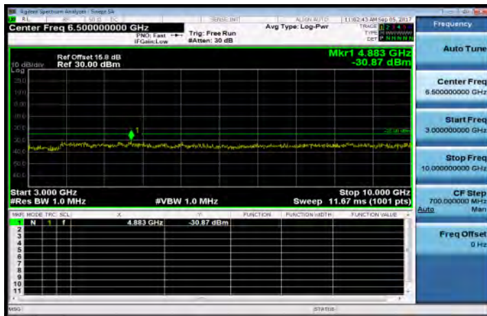
3GHz~10GHz_Band13_10MHz_QPSK_1_0_LowCH23230-782
