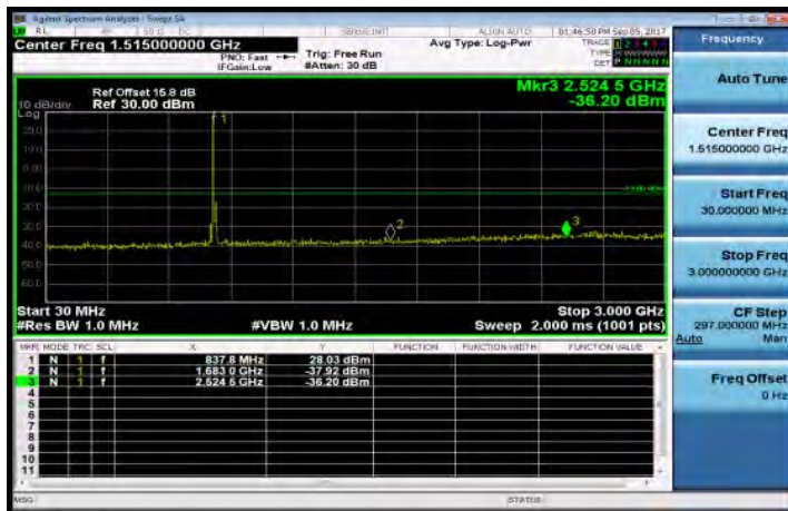
30MHz~3GHz_Band26_15MHz_QPSK_1_0_HighCH26965-841.5
