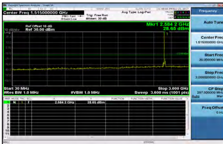
30MHz~3GHz_Band41_20MHz_QPSK_1_0_MidCH40620
