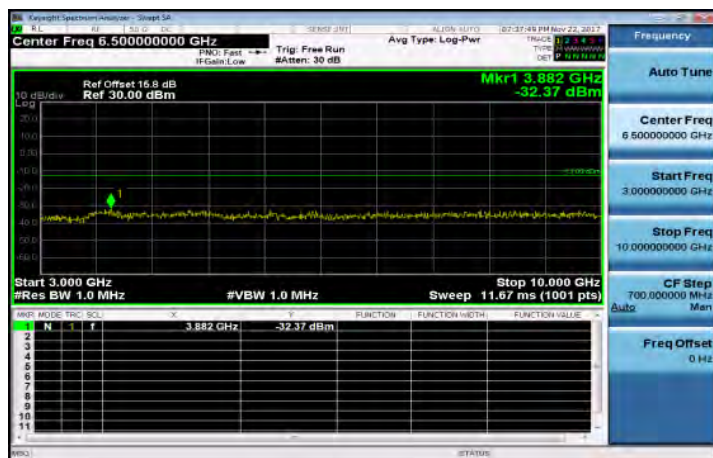
3GHz-10GHz_Band17_5MHz_QPSK_1_0_MidCH23790-710
