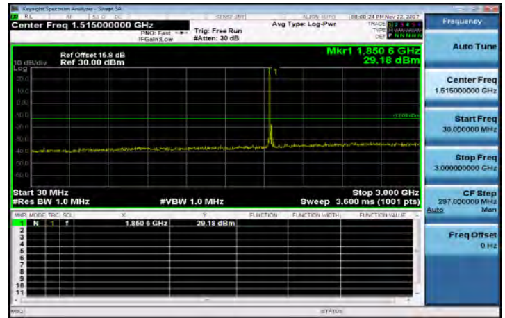
30MHz~3GHz_Band25_20MHz_QPSK_1_0_LowCH26140-1860
