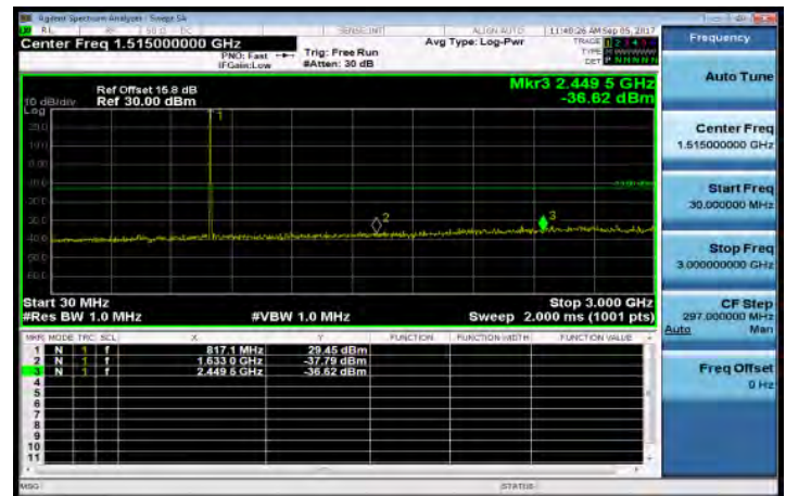
30MHz~3GHz_Band26_5MHz_QPSK_1_0_LowCH26715-816.5
