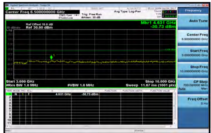
3GHz~10GHz_Band5_10MHz_QPSK_1_0_HighCH20600-844
