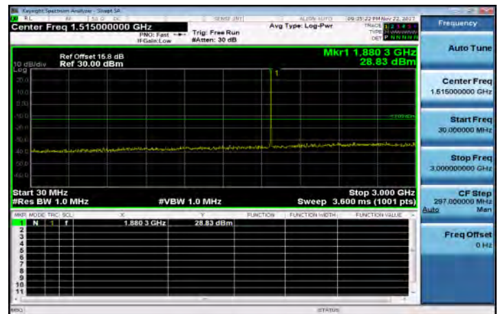
30MHz~3GHz_Band25_3MHz_QPSK_1_0_MidCH26365-1882.5
