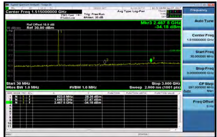
30MHz-3GHz_Band26_3MHz_QPSK_1_0_HighCH26775
