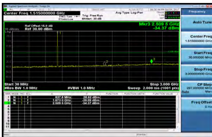
30MHz~3GHz_Band5_1_4MHz_QPSK_1_0_MidCH20525-836.5
