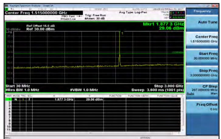
30MHz~3GHz_Band25_10MHz_QPSK_1_0_MidCH26365-1882.5
