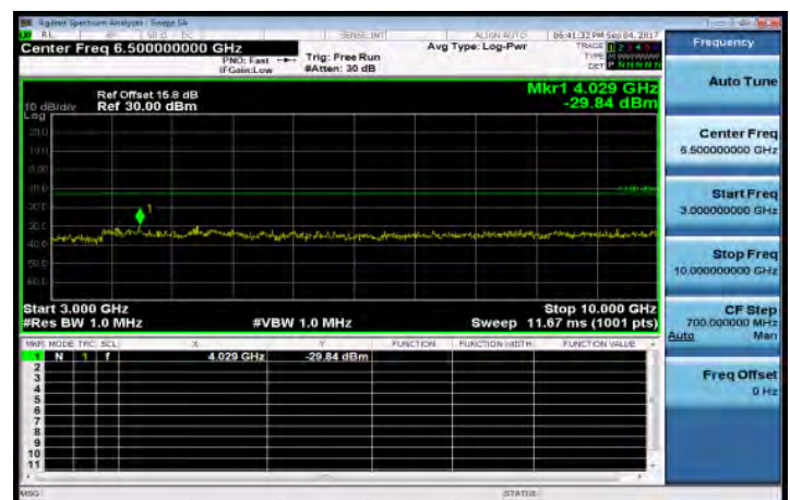
3GHz~10GHz_Band12_10MHz_QPSK_1_0_HighCH23130-711
