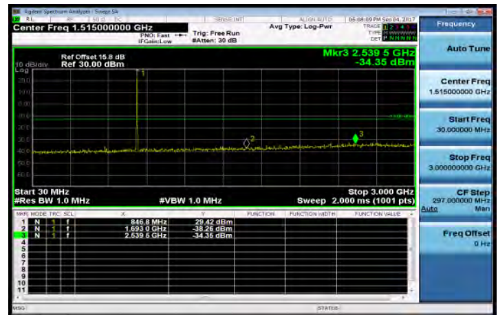
30MHz~3GHz_Band5_5MHz_QPSK_1_0_HighCH20625-846.5
