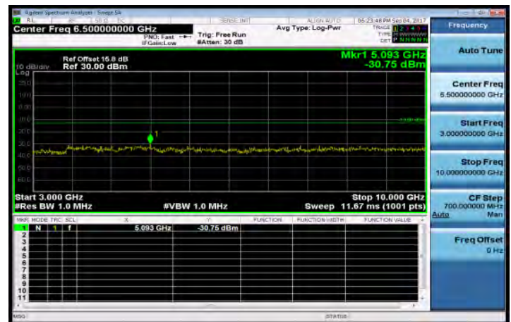
3GHz~10GHz_Band5_3MHz_QPSK_1_0_HighCH20635-847.5
