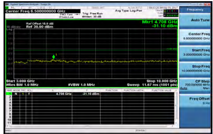
3GHz~10GHz_Band12_1_4MHz_QPSK_1_0_MidCH23095-707.5
