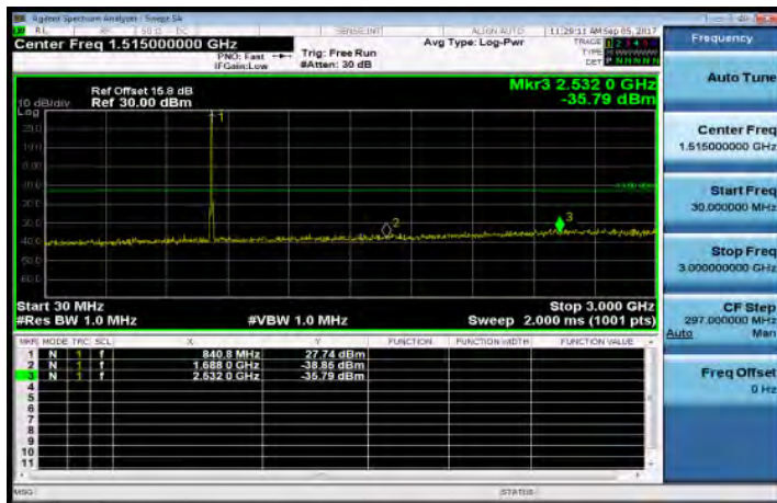
30MHz~3GHz_Band26_10MHz_QPSK_1_0_HighCH26990-844
