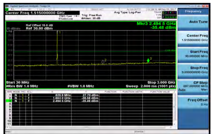
30MHz~3GHz_Band26_10MHz_QPSK_1_0_MidCH26865-831.5
