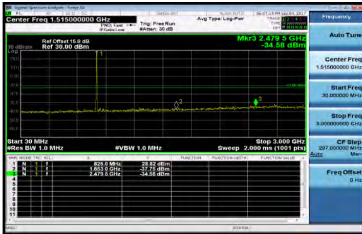
30MHz~3GHz_Band5_5MHz_QPSK_1_0_LowCH20425-826.5
