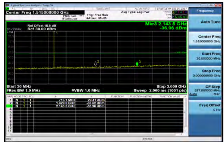
30MHz-3GHz_Band12_3MHz_QPSK_1_0_HighCH23165-714.5
