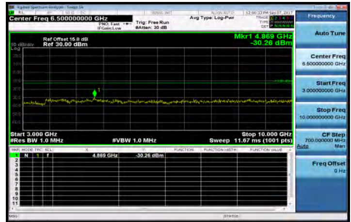
3GHz~10GHz_Band26_5MHz_QPSK_1_0_MidCH26740
