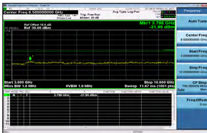
3GHz-10GHz_Band17_5MHz_QPSK_1_0_HighCH23825-713.5
