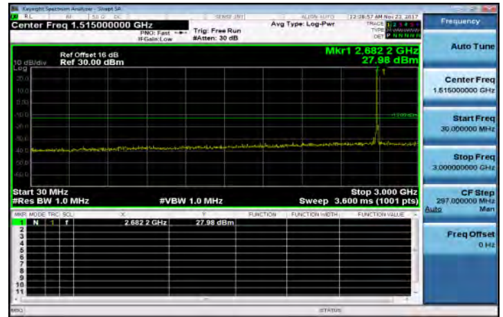
30MHz~3GHz_Band41_10MHz_QPSK_1_0_HighCH41540
