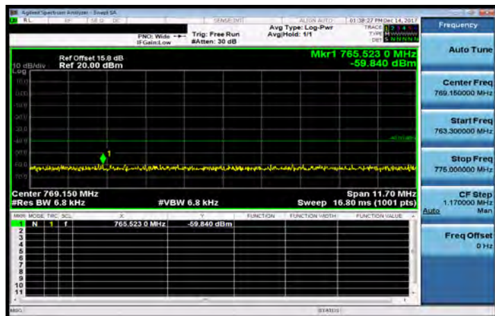
763.3MHz~775MHz_Band13_5MHz_QPSK_1_0_MidCH23230-782
