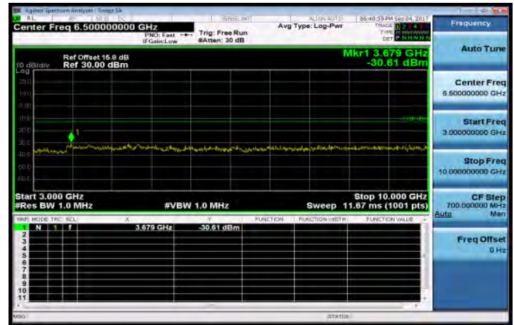
3GHz~10GHz_Band12_10MHz_QPSK_1_0_MidCH23095-707.5
