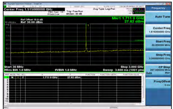
30MHz~3GHz_Band66_10MHz_QPSK_1_0_LowCH132022
