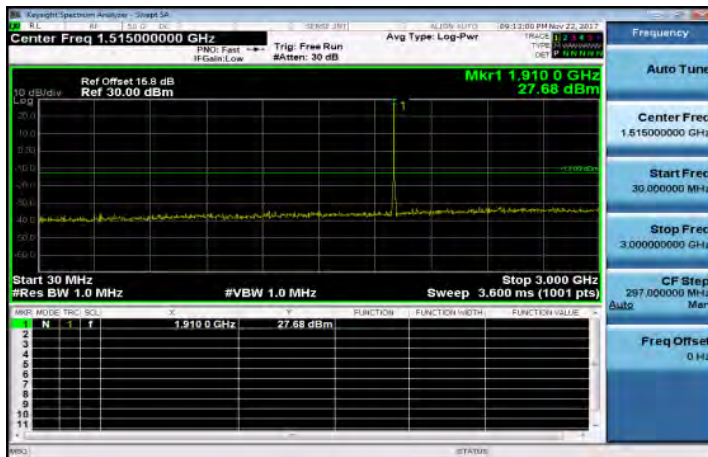
30MHz~3GHz_Band25_5MHz_QPSK_1_0_HighCH26665-1912.5
