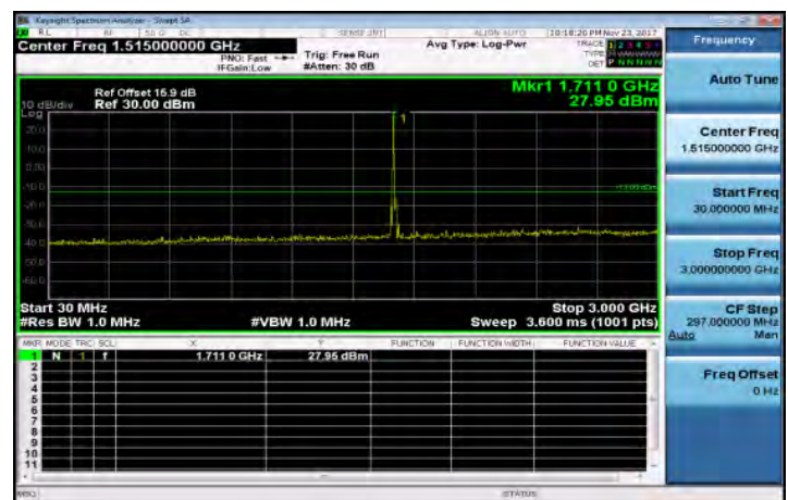
30MHz~3GHz_Band66_15MHz_QPSK_1_0_LowCH132047
