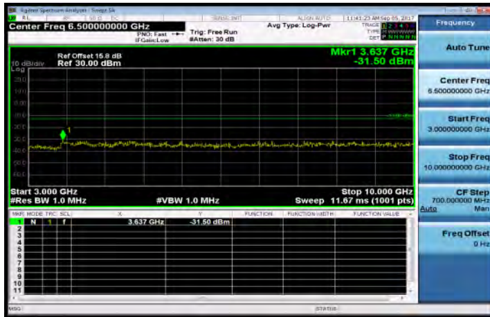
3GHz~10GHz_Band26_5MHz_QPSK_1_0_MidCH26865-831.5
