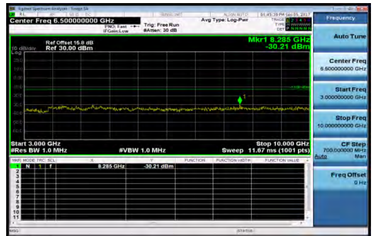
3GHz~10GHz_Band26_15MHz_QPSK_1_0_LowCH26825-822.5
