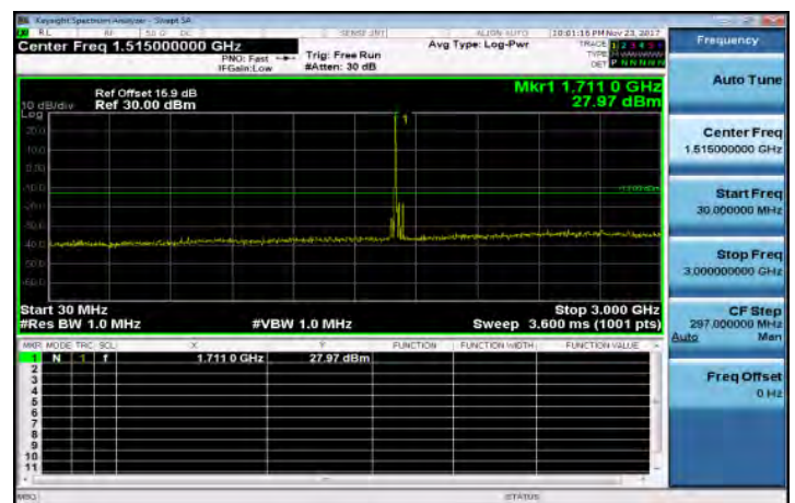
30MHz~3GHz_Band66_20MHz_QPSK_1_0_LowCH132072
