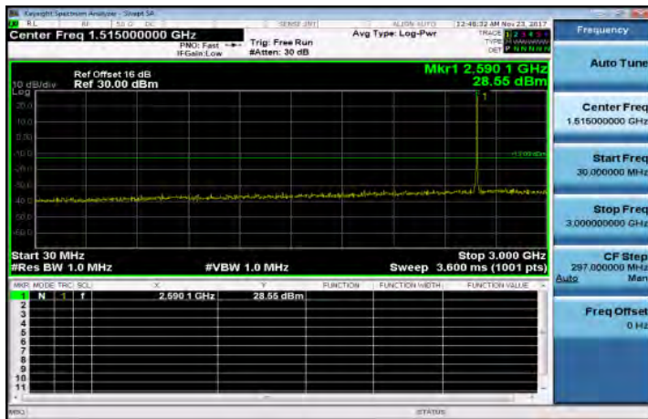
30MHz~3GHz_Band41_5MHz_QPSK_1_0_MidCH40620
