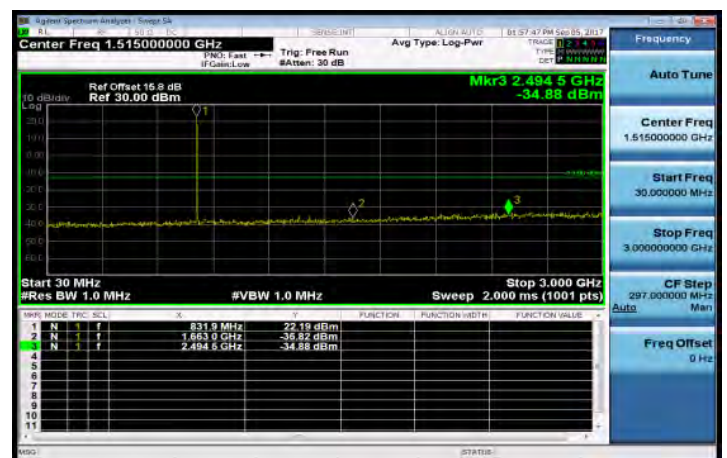
30MHz~3GHz_Band26_1_4MHz_QPSK_1_0_MidCH26865-831.5
