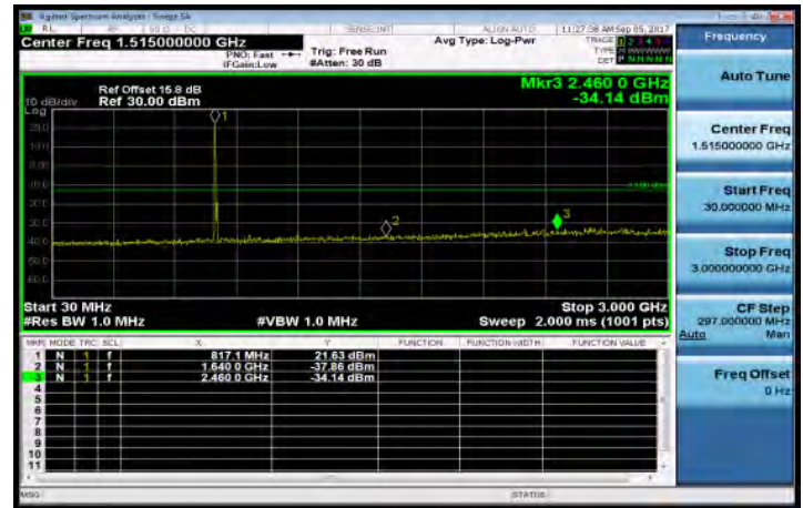
30MHz~3GHz_Band26_10MHz_QPSK_1_0_LowCH26750-820
