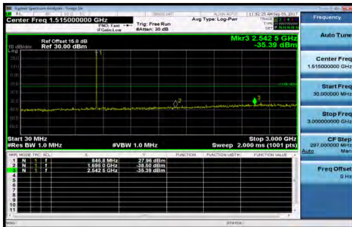
30MHz~3GHz_Band26_3MHz_QPSK_1_0_HighCH27025-847.5
