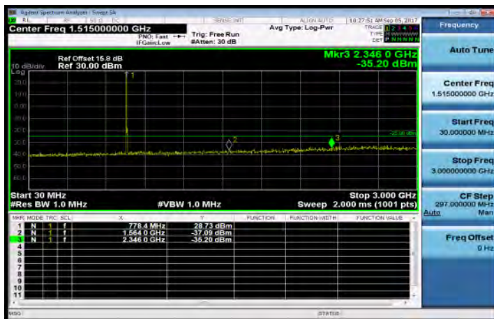
30MHz~3GHz_Band13_10MHz_QPSK_1_0_MidCH23230-782
