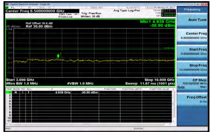
3GHz~10GHz_Band13_5MHz_QPSK_1_0_MidCH23230-782
