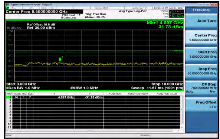
3GHz-10GHz_Band26_3MHz_QPSK_1_0_MidCH26740
