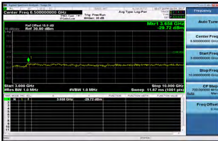
3GHz~10GHz_Band5_5MHz_QPSK_1_0_LowCH20425-826.5
