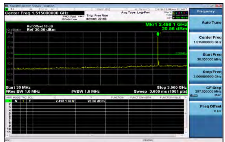
30MHz~3GHz_Band41_20MHz_QPSK_1_0_LowCH39750
