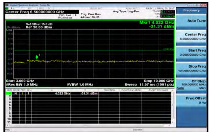
3GHz~10GHz_Band12_1_4MHz_QPSK_1_0_HighCH23173-715.3
