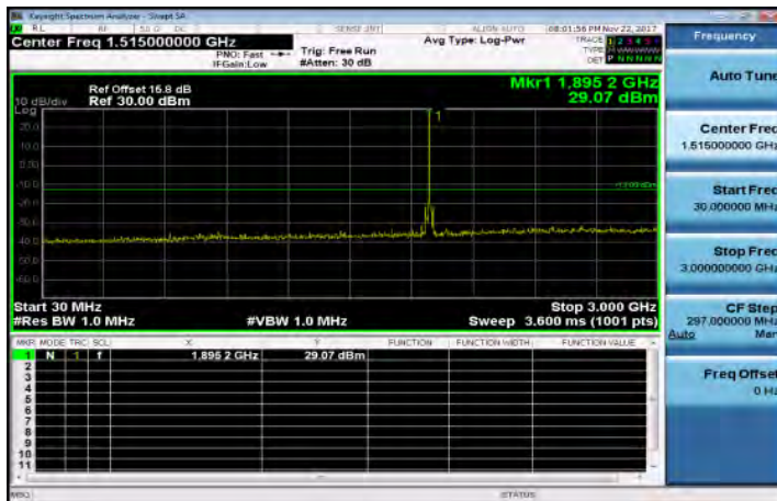
30MHz~3GHz_Band25_20MHz_QPSK_1_0_HighCH26590-1905
