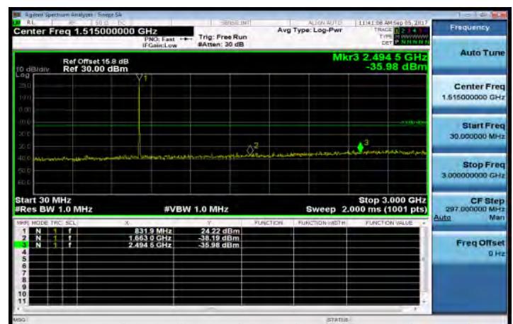
30MHz~3GHz_Band26_5MHz_QPSK_1_0_MidCH26865-831.5
