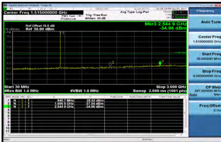
30MHz~3GHz_Band26_1_4MHz_QPSK_1_0_HighCH27033-848.3
