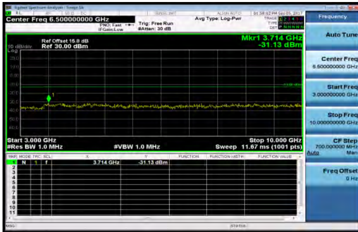
3GHz~10GHz_Band26_1_4MHz_QPSK_1_0_MidCH26865-831.5
