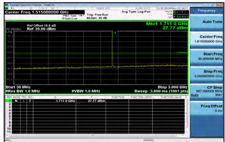
30MHz-3GHz_Band66_3MHz_QPSK_1_0_LowCH131987
