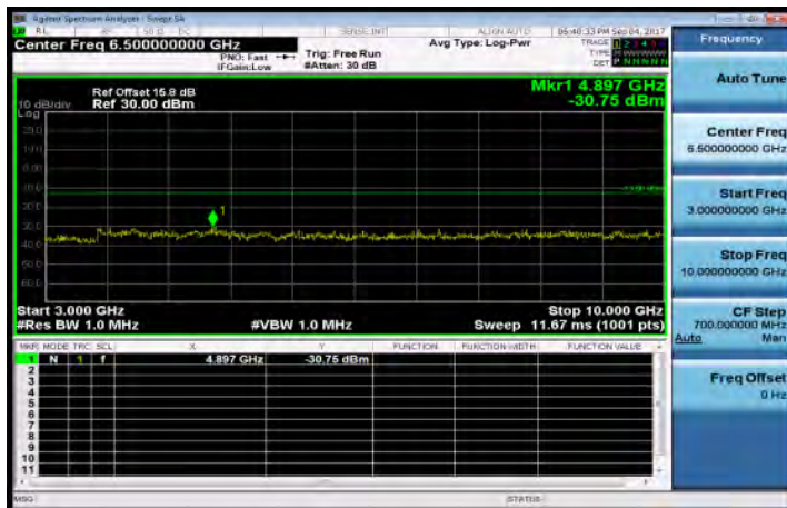
3GHz~10GHz_Band12_10MHz_QPSK_1_0_LowCH23060-704
