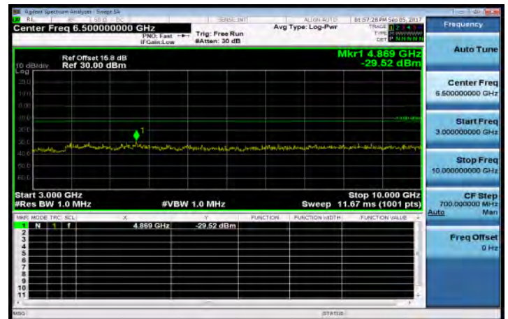
3GHz~10GHz_Band26_1_4MHz_QPSK_1_0_LowCH26697-814.7
