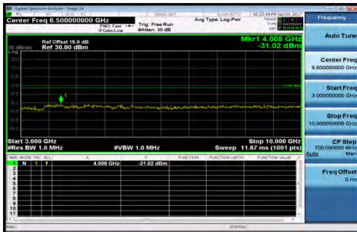
3GHz~10GHz_Band5_3MHz_QPSK_1_0_LowCH20415-825.5
