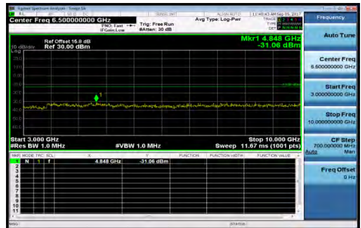
3GHz~10GHz_Band26_5MHz_QPSK_1_0_LowCH26715-816.5
