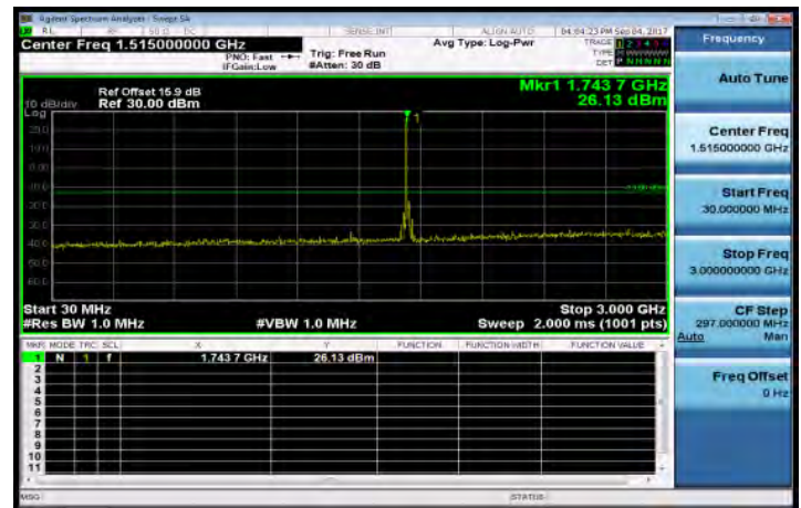
30MHz~3GHz_Band4_15MHz_QPSK_1_0_HighCH20325-1747.5
