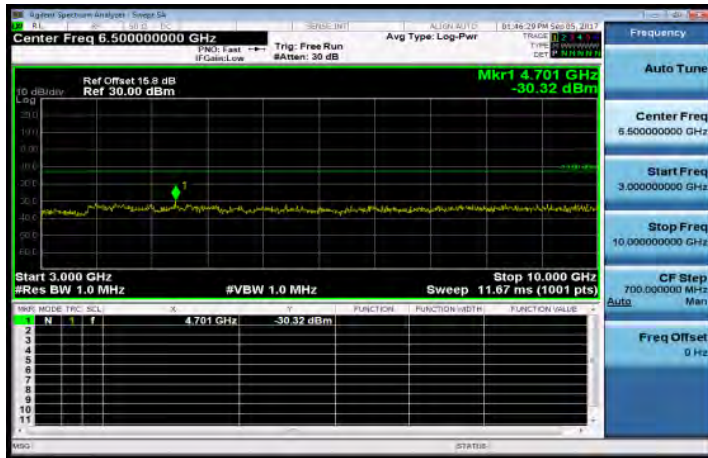
3GHz~10GHz_Band26_15MHz_QPSK_1_0_MidCH26865-831.5
