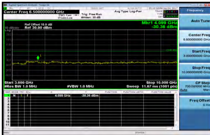
3GHz~10GHz_Band5_10MHz_QPSK_1_0_LowCH20450-829
