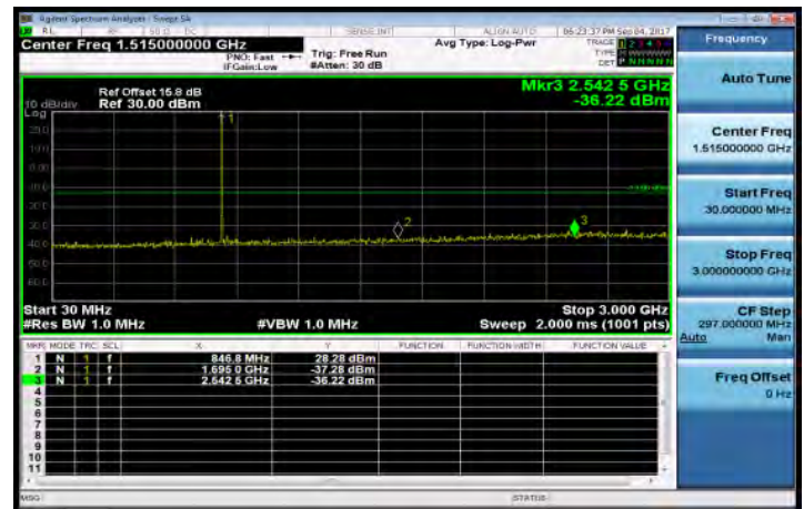
30MHz~3GHz_Band5_3MHz_QPSK_1_0_HighCH20635-847.5
