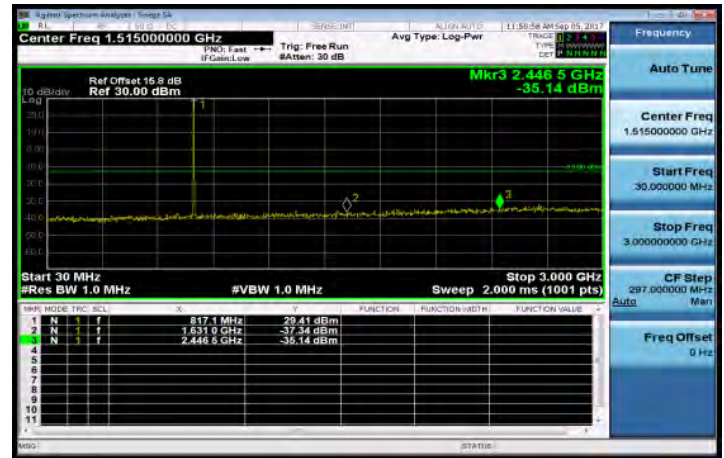
30MHz~3GHz_Band26_3MHz_QPSK_1_0_LowCH26705-815.5
