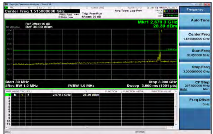
30MHz~3GHz_Band41_20MHz_QPSK_1_0_HighCH41490
