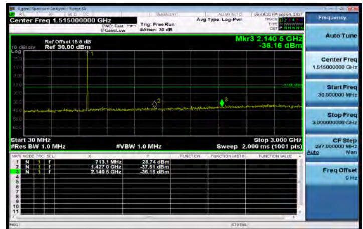
30MHz-3GHz_Band12_5MHz_QPSK_1_0_HighCH23155-713.5
