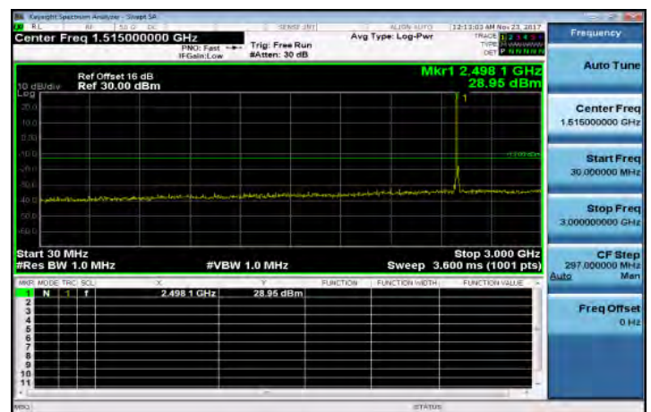
30MHz~3GHz_Band41_15MHz_QPSK_1_0_LowCH39725
