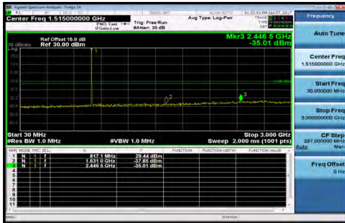
30MHz-3GHz_Band26_3MHz_QPSK_1_0_LowCH26705
