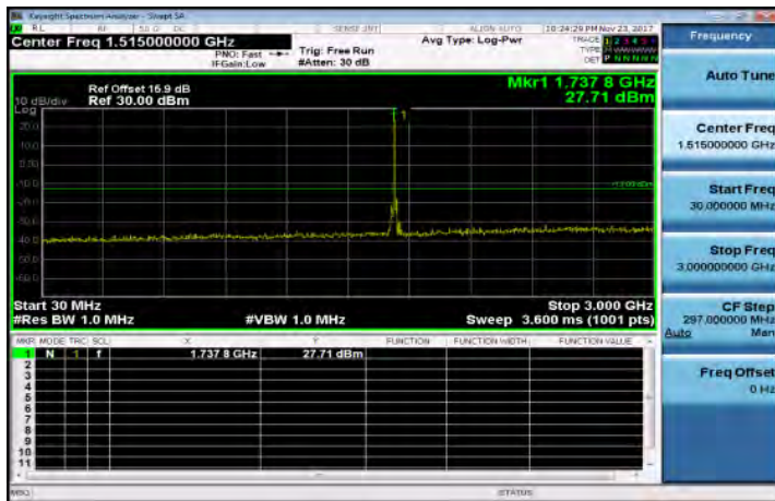
30MHz~3GHz_Band66_15MHz_QPSK_1_0_MidCH132322
