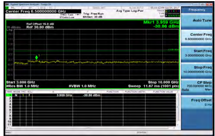
3GHz~10GHz_Band5_10MHz_QPSK_1_0_MidCH20525-836.5
