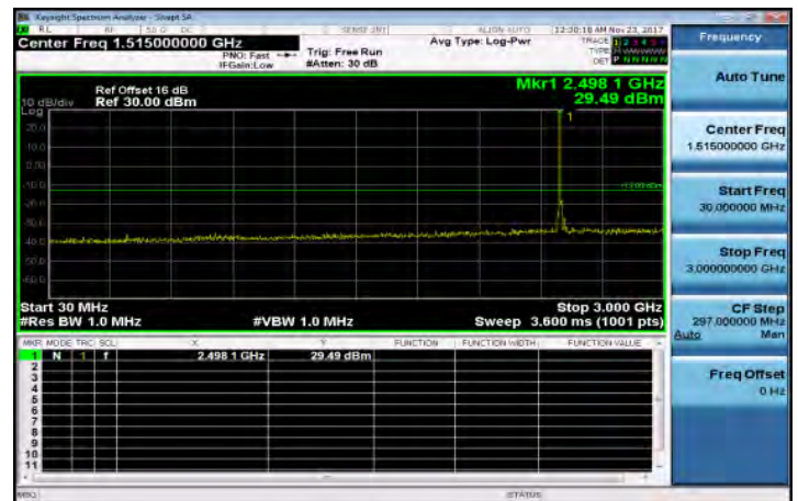
30MHz~3GHz_Band41_10MHz_QPSK_1_0_LowCH39700
