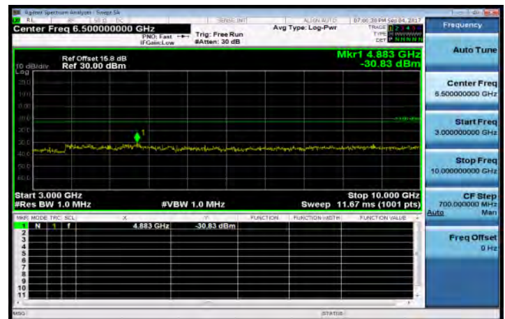
3GHz-10GHz_Band12_3MHz_QPSK_1_0_HighCH23165-714.5
