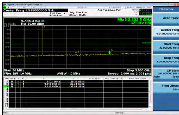
30MHz~3GHz_Band12_1_4MHz_QPSK_1_0_MidCH23095-707.5
