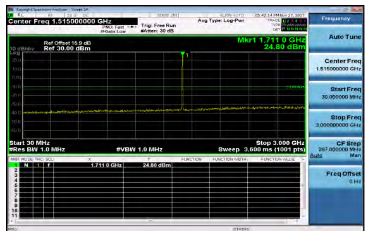
30MHz~3GHz_Band66_1_4MHz_QPSK_1_0_LowCH131979
