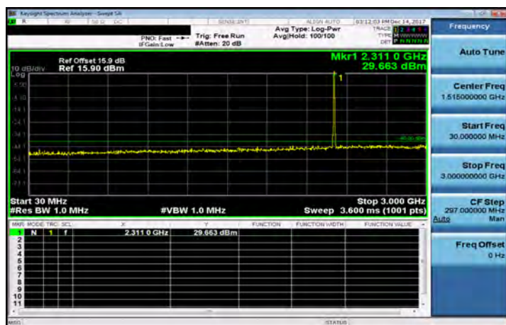
30MHz~3GHz_Band30_5MHz_QPSK_1_0_HighCH27735
