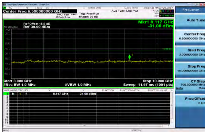
3GHz~10GHz_Band17_10MHz_QPSK_1_0_HighCH23800-711
