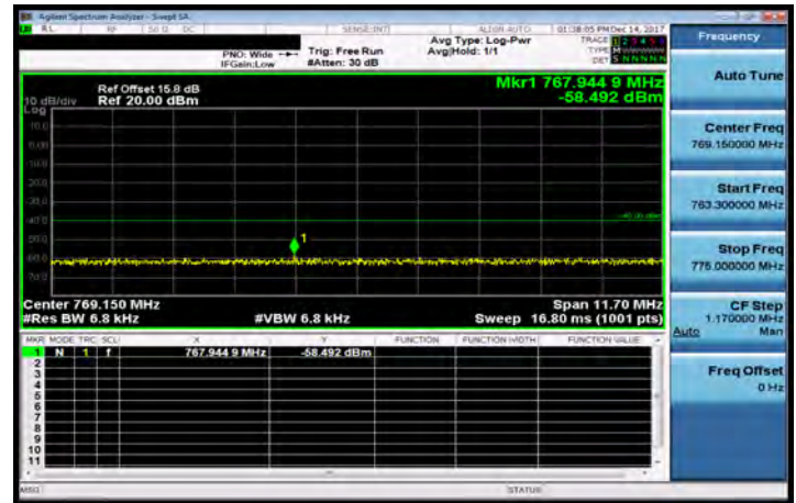
763.3MHz~775MHz_Band13_5MHz_QPSK_1_0_LowCH23205-779.5
