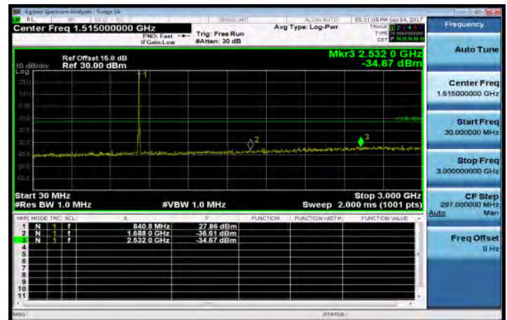
30MHz~3GHz_Band5_10MHz_QPSK_1_0_HighCH20600-844
