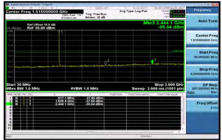
30MHz~3GHz_Band26_1_4MHz_QPSK_1_0_LowCH26697-814.7
