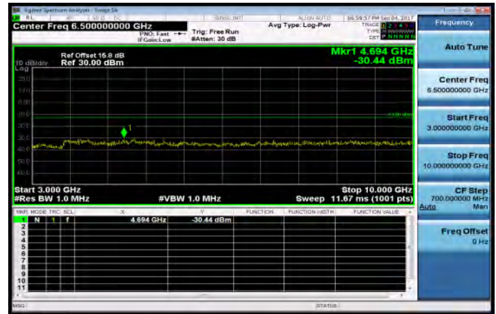
3GHz-10GHz_Band12_3MHz_QPSK_1_0_MidCH23095-707.5
