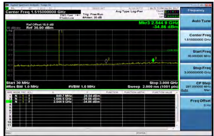
30MHz~3GHz_Band5_1_4MHz_QPSK_1_0_HighCH20643-848.3
