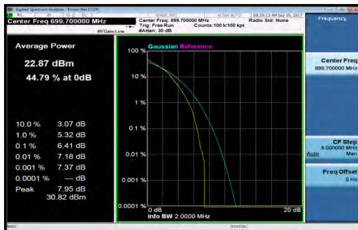
LTE_Band12_1_4MHz_64QAM_6_0_LowCH23017-699.7
