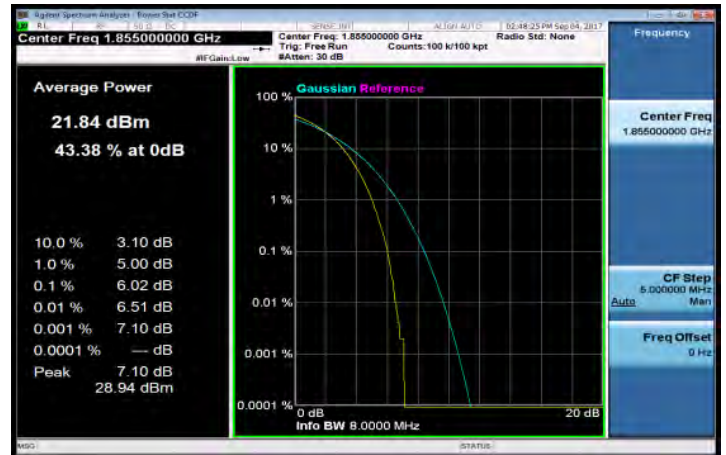
LTE_Band2_10MHz_64QAM_50_0_LowCH18650-1855
