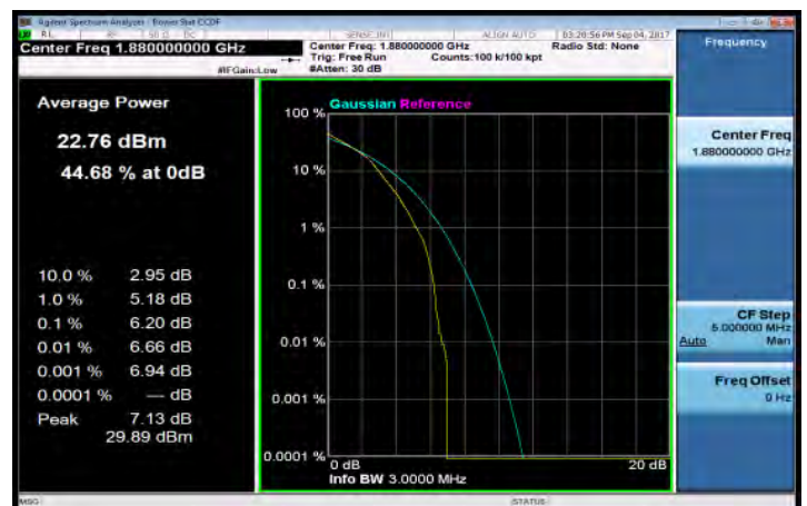
LTE_Band2_3MHz_16QAM_15_0_MidCH18900-1880
