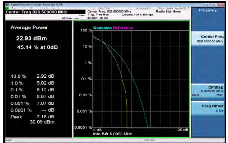
LTE_Band5_5MHz_64QAM_25_0_LowCH20425-826.5
