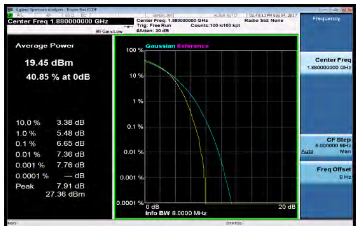
LTE_Band2_15MHz_16QAM_75_0_MidCH18900-1880
