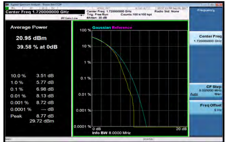
LTE_Band4_20MHz_64QAM_100_0_LowCH20050-1720
