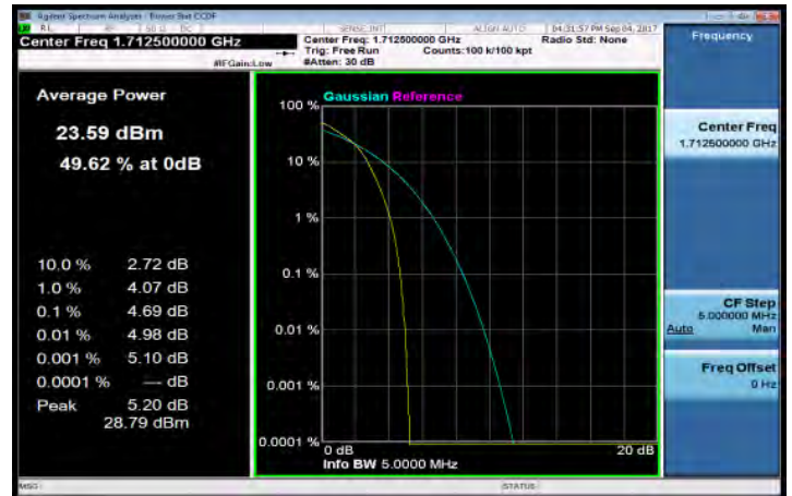
LTE_Band4_5MHz_64QAM_25_0_LowCH19975-1712.5
