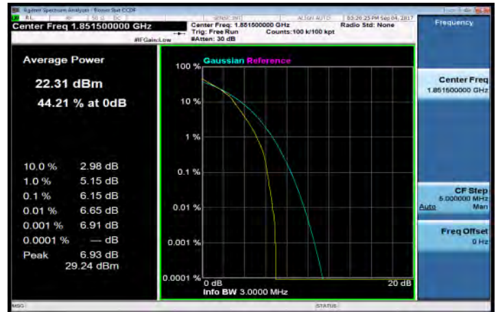
LTE_Band2_3MHz_64QAM_15_0_LowCH18615-1851.5
