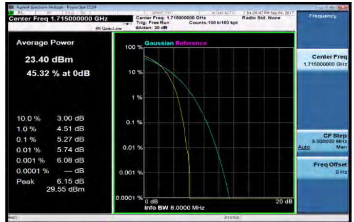
LTE_Band4_10MHz_64QAM_50_0_LowCH20000-1715
