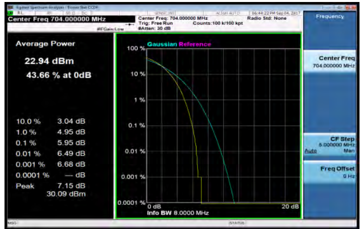
LTE_Band12_10MHz_64QAM_50_0_LowCH23060-704
