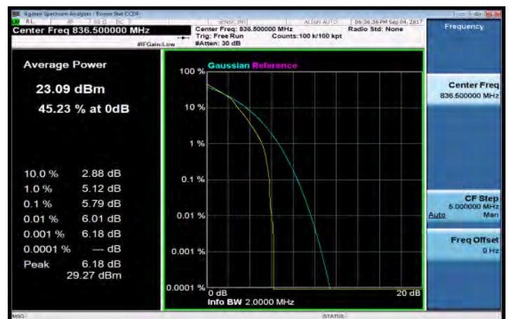
LTE_Band5_1_4MHz_16QAM_6_0_MidCH20525-836.5
