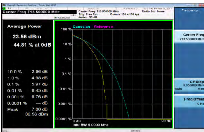
LTE_Band12_5MHz_64QAM_25_0_HighCH23155-713.5
