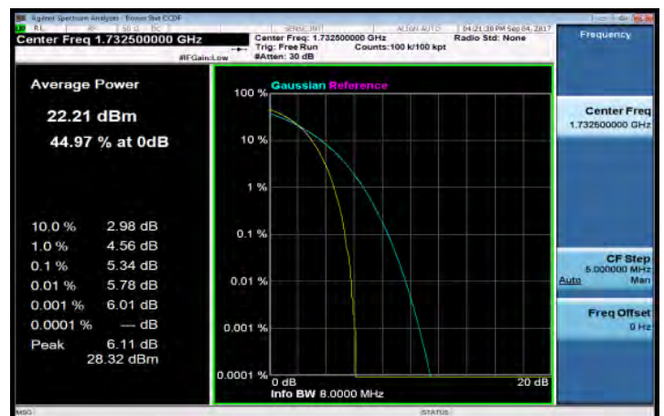
LTE_Band4_10MHz_16QAM_50_0_MidCH20175-1732.5
