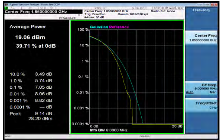
LTE_Band2_20MHz_64QAM_100_0_LowCH18700-1860
