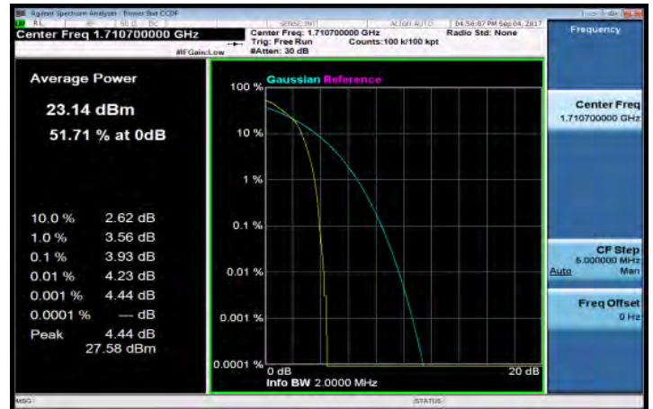
LTE_Band4_1_4MHz_64QAM_6_0_LowCH19957-1710.7
