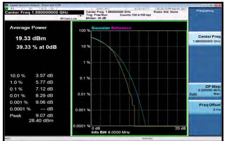
LTE_Band2_20MHz_16QAM_100_0_MidCH18900-1880
