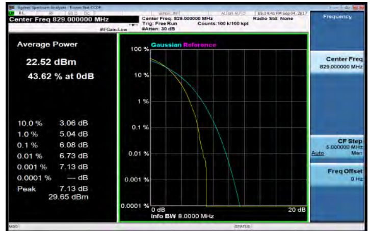
LTE_Band5_10MHz_64QAM_50_0_LowCH20450-829
