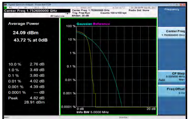
HSUPA_B4_HighCH1513-1752.6
