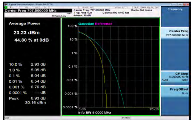
LTE_Band12_5MHz_16QAM_25_0_MidCH23095-707.5
