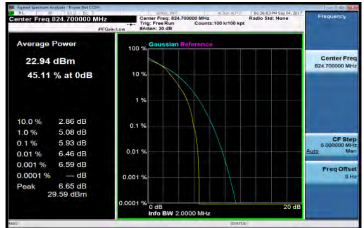
LTE_Band5_1_4MHz_64QAM_6_0_LowCH20407-824.7
