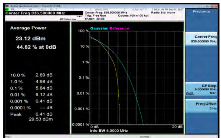
LTE_Band5_5MHz_16QAM_25_0_MidCH20525-836.5
