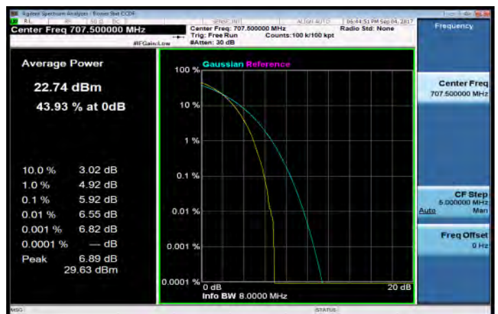
LTE_Band12_10MHz_16QAM_50_0_MidCH23095-707.5
