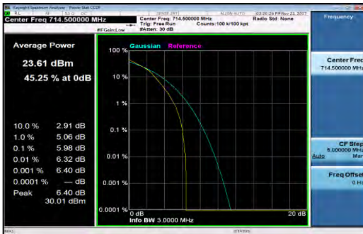
LTE_Band12_3MHz_64QAM_15_0_HighCH23165-714.5
