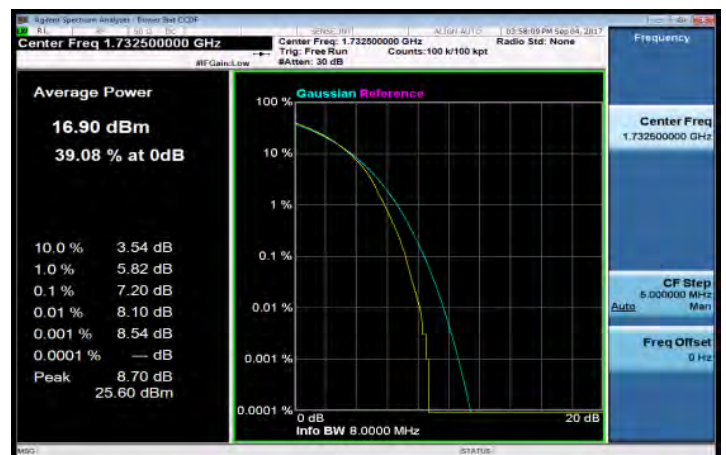
LTE_Band4_20MHz_16QAM_100_0_MidCH20175-1732.5
