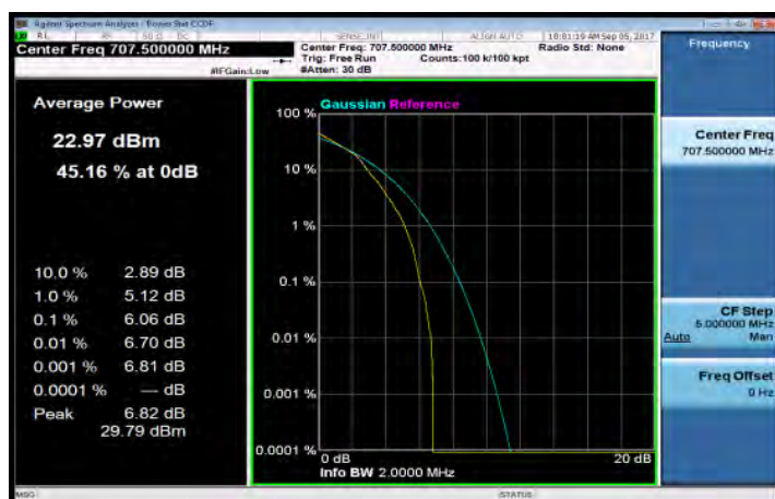
LTE_Band12_1_4MHz_16QAM_6_0_MidCH23095-707.5
