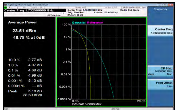
LTE_Band4_5MHz_16QAM_25_0_MidCH20175-1732.5
