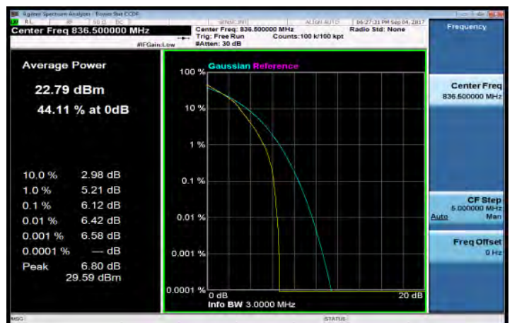
LTE_Band5_3MHz_16QAM_15_0_MidCH20525-836.5
