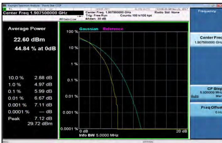
LTE_Band2_5MHz_64QAM_25_0_HighCH19175-1907.5
