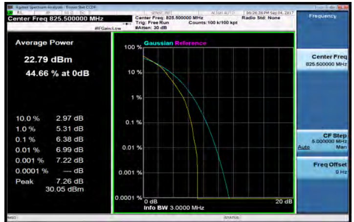
LTE_Band5_3MHz_64QAM_15_0_LowCH20415-825.5
