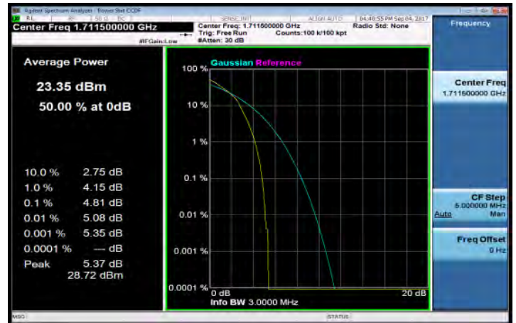
LTE_Band4_3MHz_64QAM_15_0_LowCH19965-1711.5
