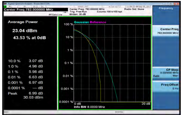
LTE_Band13_10MHz_64QAM_50_0_MidCH23230-782
