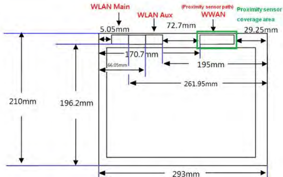
Fig.11 Antenna position of EUT
