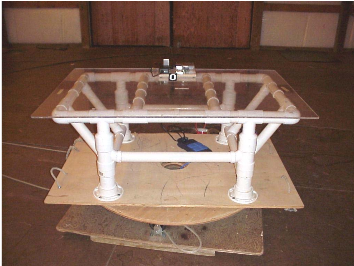
Radiated / Horizontal Setup - Front
