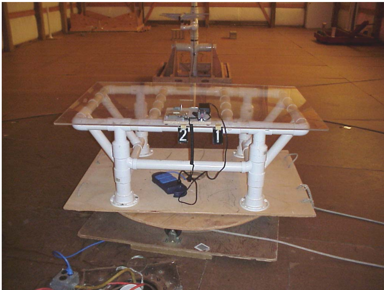
Radiated / Horizontal Setup - Back
