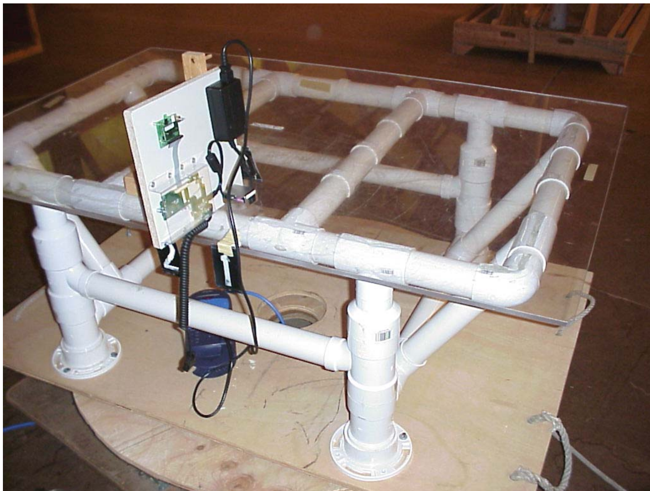
Radiated Setup, 90 degree rotation - Back
