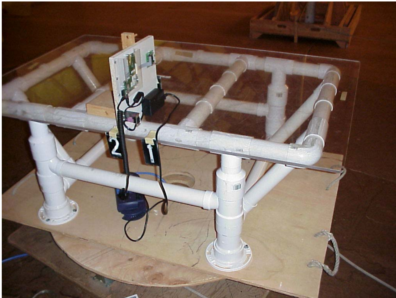
Radiated / Vertical Setup - Back
