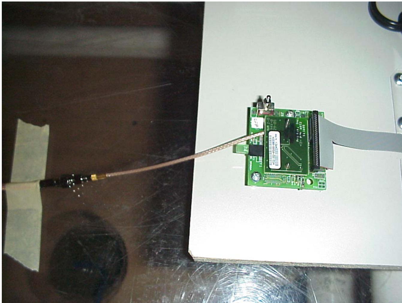
RF Conducted 2
