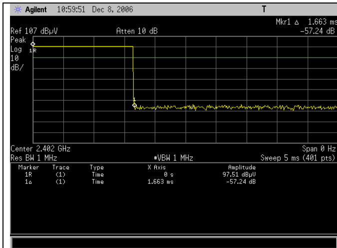
Channel On-Time
