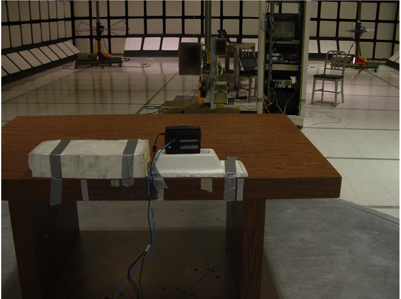
Emissions Y-Axis Setup Photo
