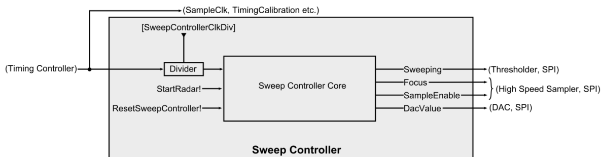
Figure 6. Sweep Controller block diagram.
