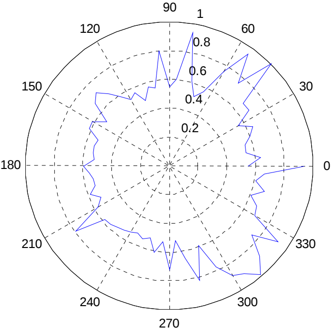
Normalized power pattern (in linear scale) for Pulse ON 200 antenna with corner reflector at 10Gi
