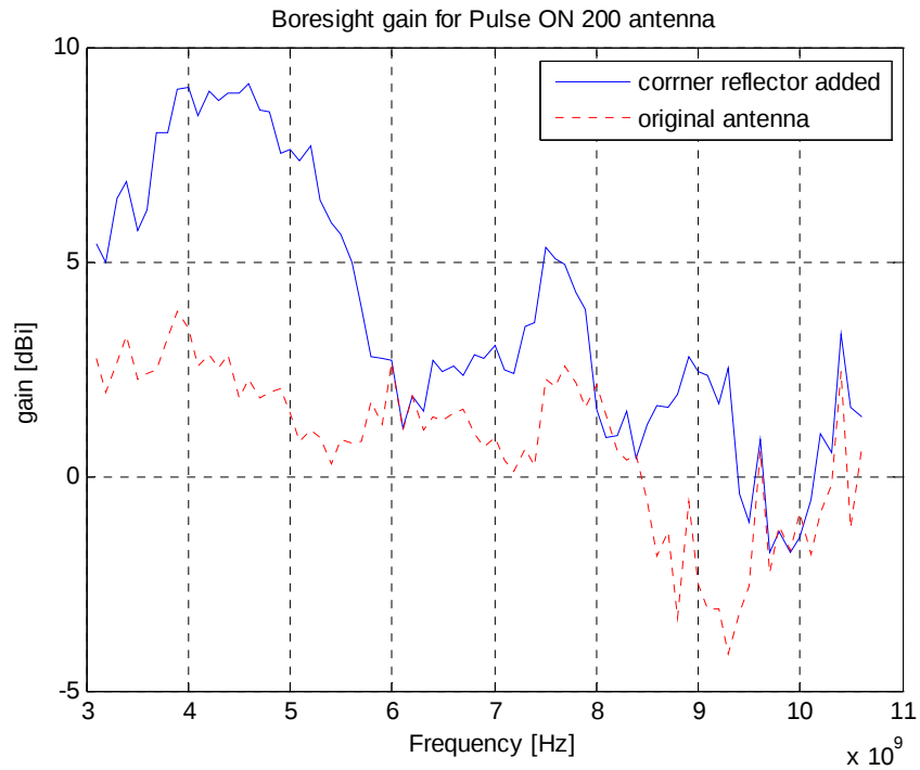
Figure 46. Boresight gain for Pulse ON 200 UWB antenna with corner reflector compared to the original antenna.
