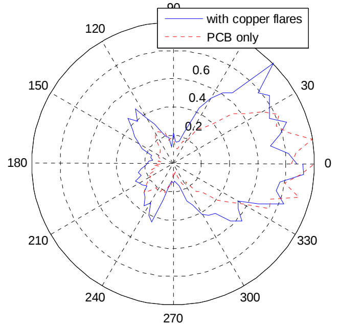
Normalized Power vs. Position at freq=5.5GHz
