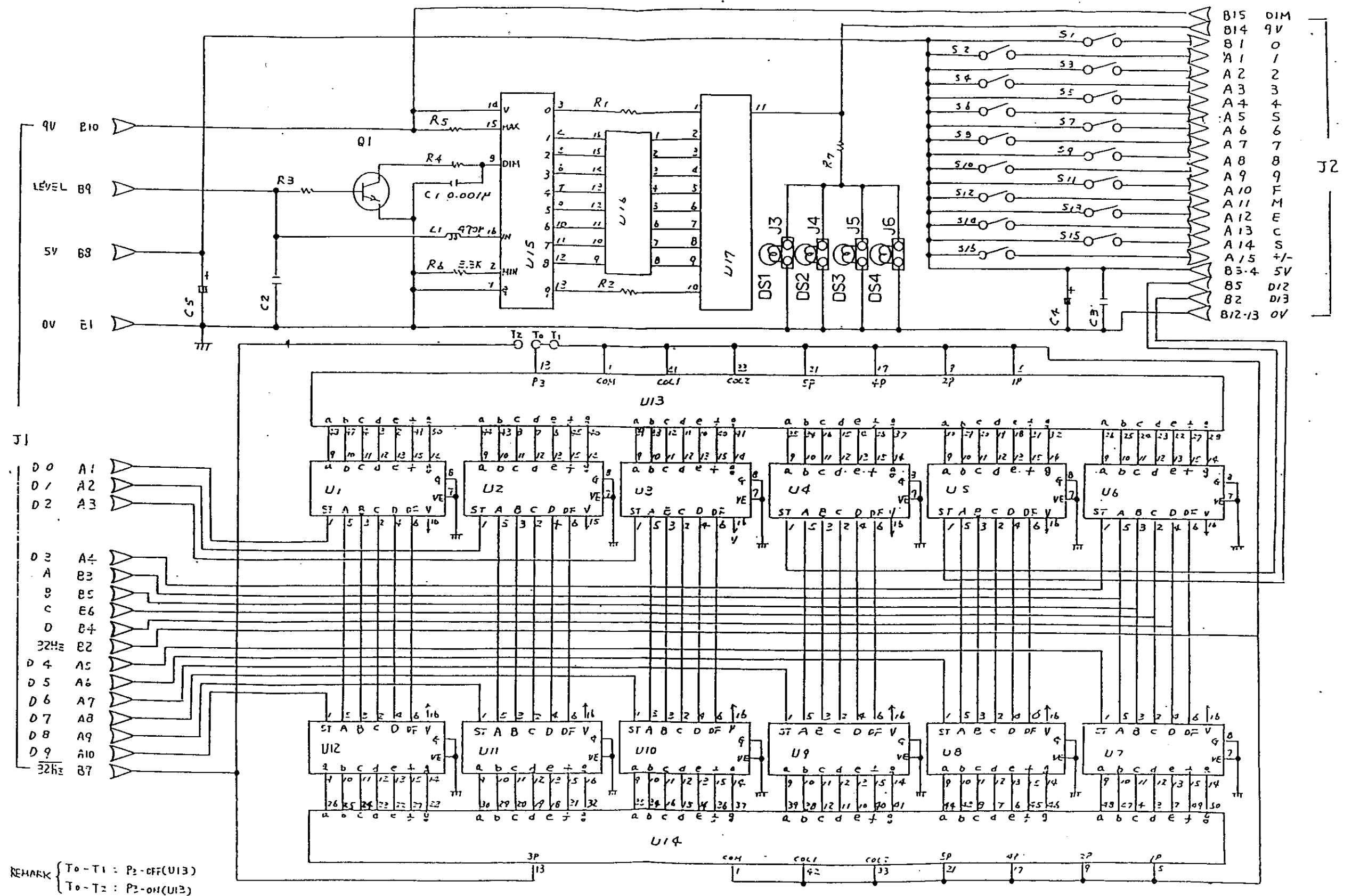
Circuit Diagram of Main Unit PCA LCD Display Drawing No. 332426 TAIYO MUSEN CO., LTD.
