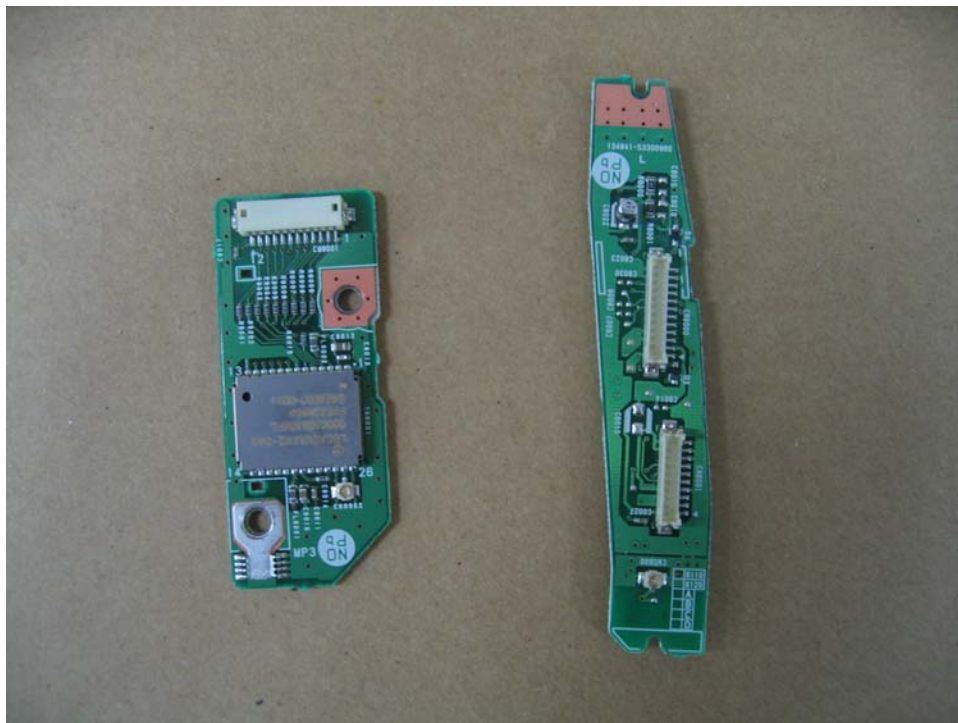
BT module and Antenna Top
