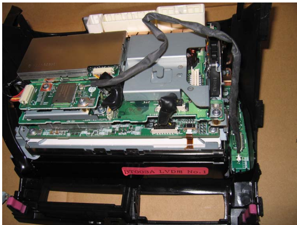
Location of BT module
