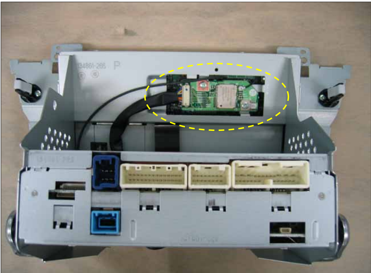
Location of Bluetooth Module
