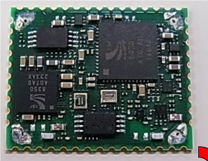
Bluetooth/ WiFi Receiver
