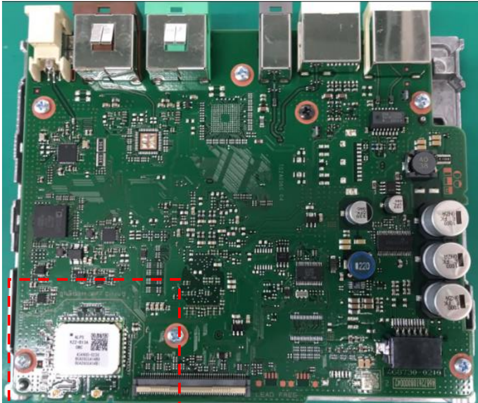
Bluetooth/ WiFi area
