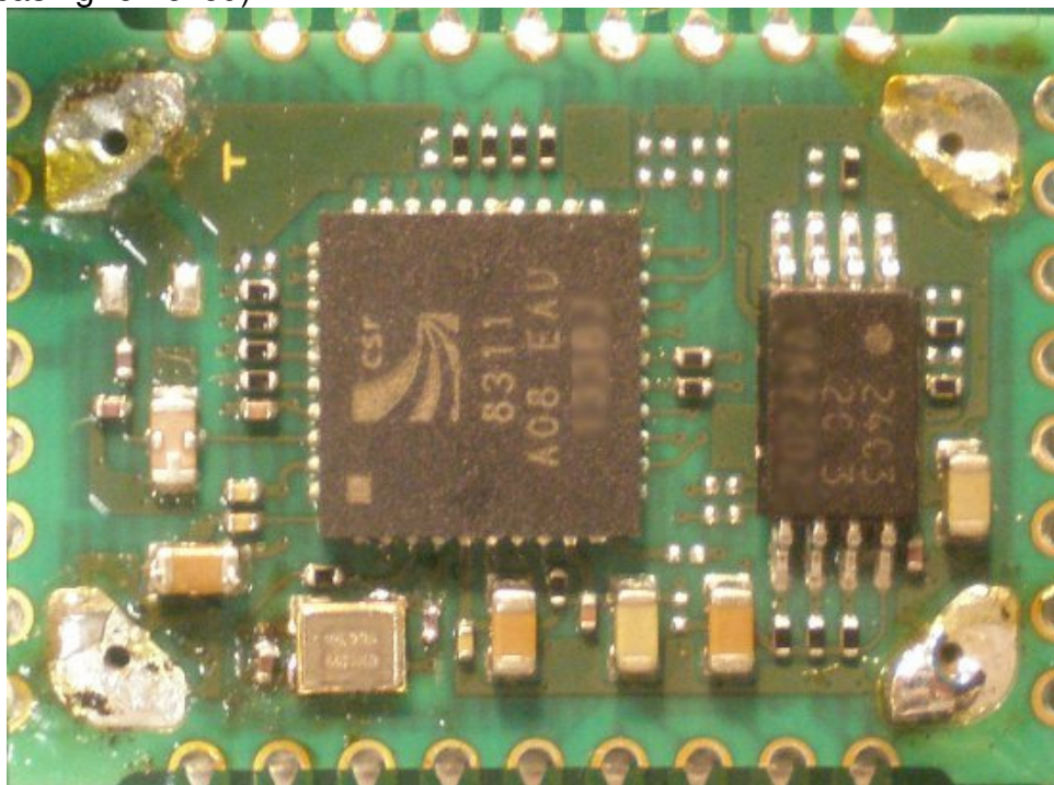
Top View – Internal (Shield casing removed)
