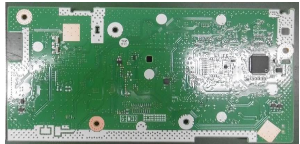
Solder side
