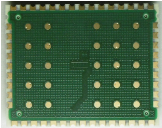
Outside View (BOTTOM)
