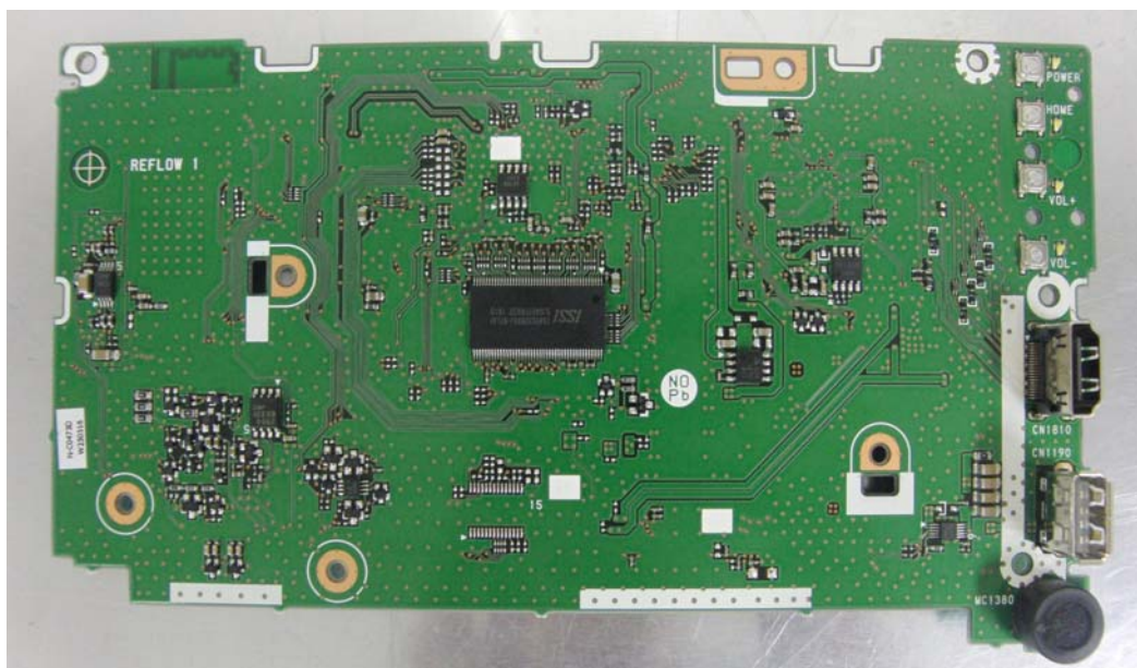
PANEL PCB ASSEMBLY (Part Side)
