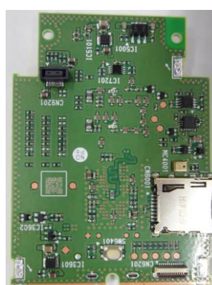
2nd board :backside
