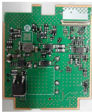
1st board :backside
