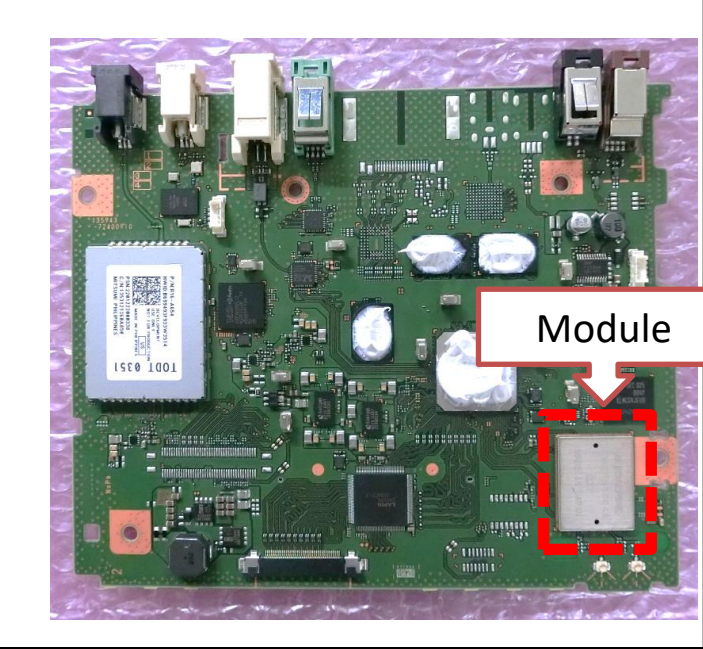
Component side
