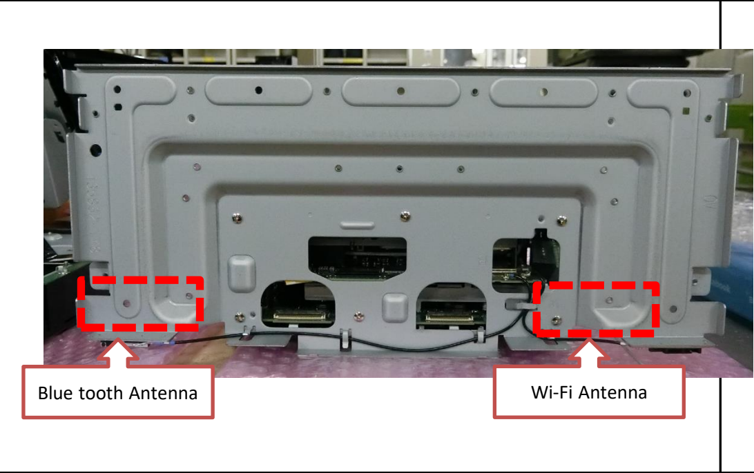
Internal view(side)
