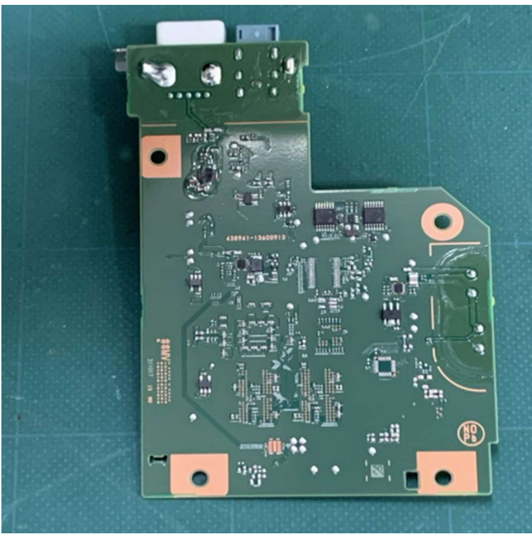
Solder side
