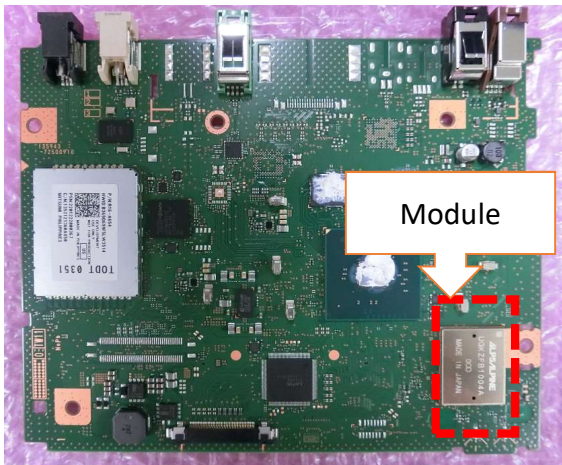
Component side
