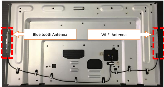
Internal view
