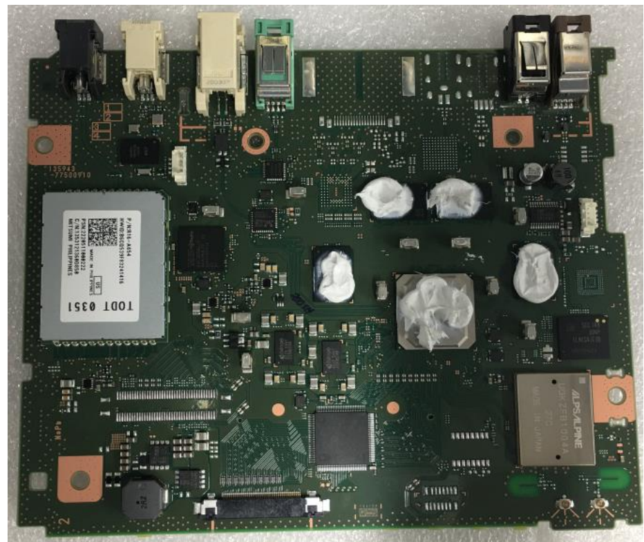
Component side
