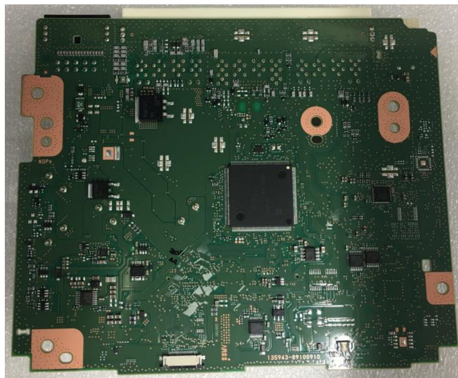
Solder side
