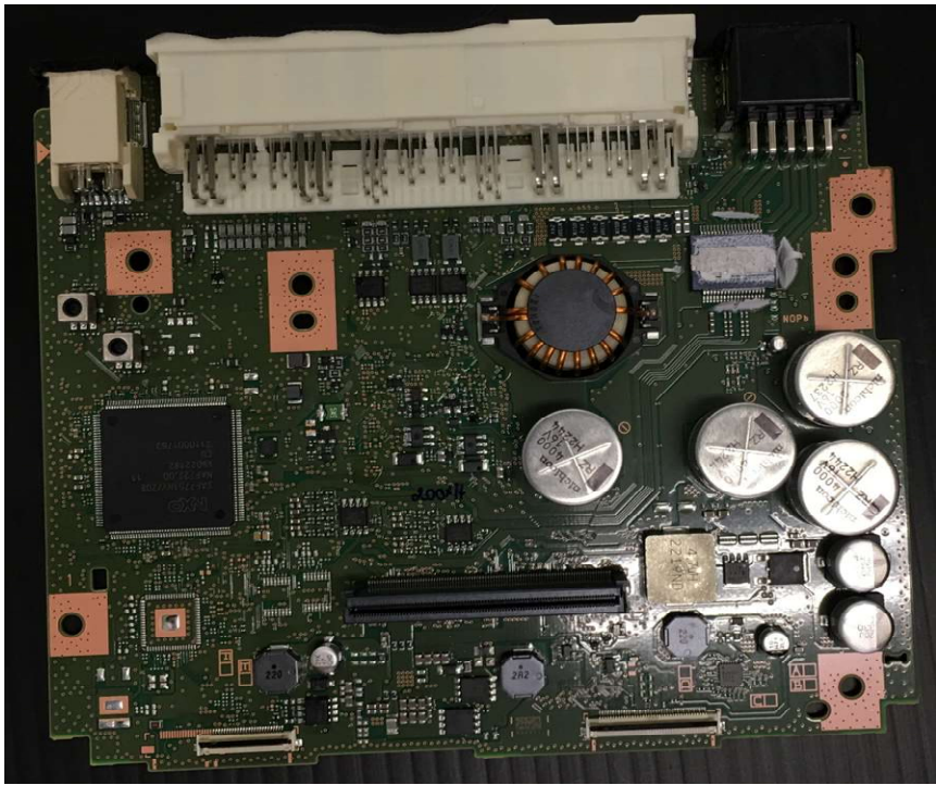
Component side
