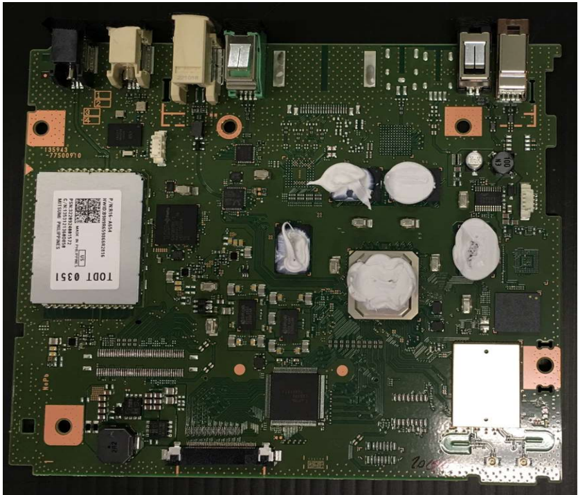
Component side
