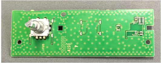
Solder side
