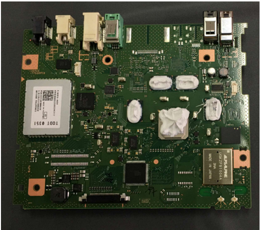
Component side
