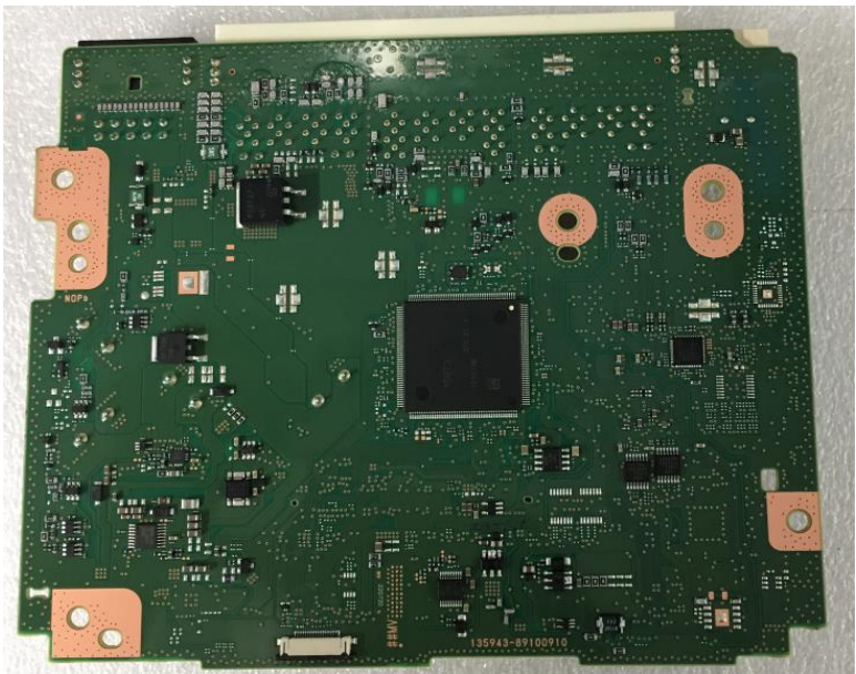
Solder side
