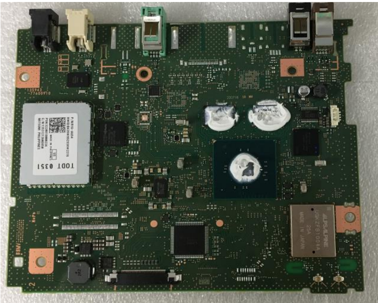
Component side
