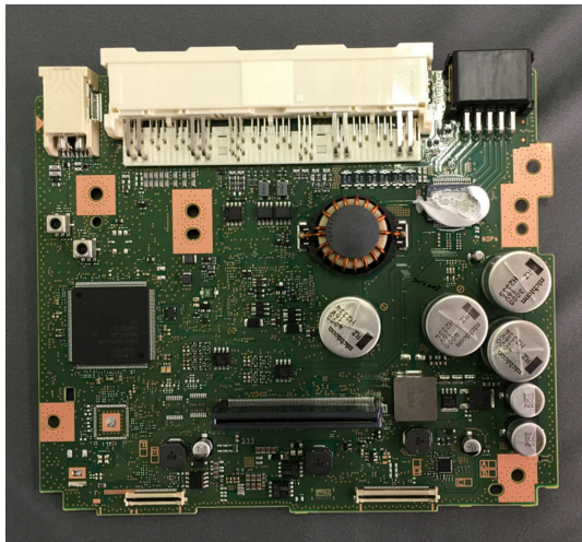
Component side
