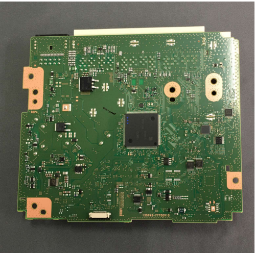
Solder side
