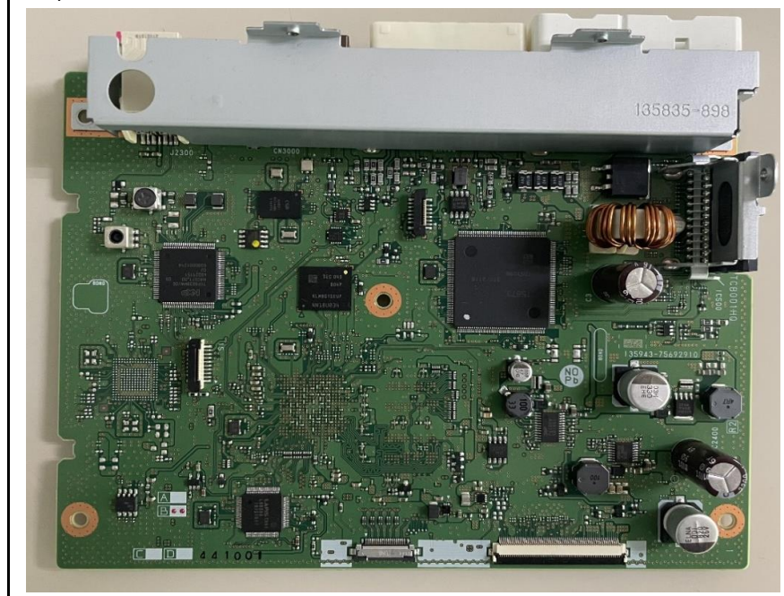
Component side
