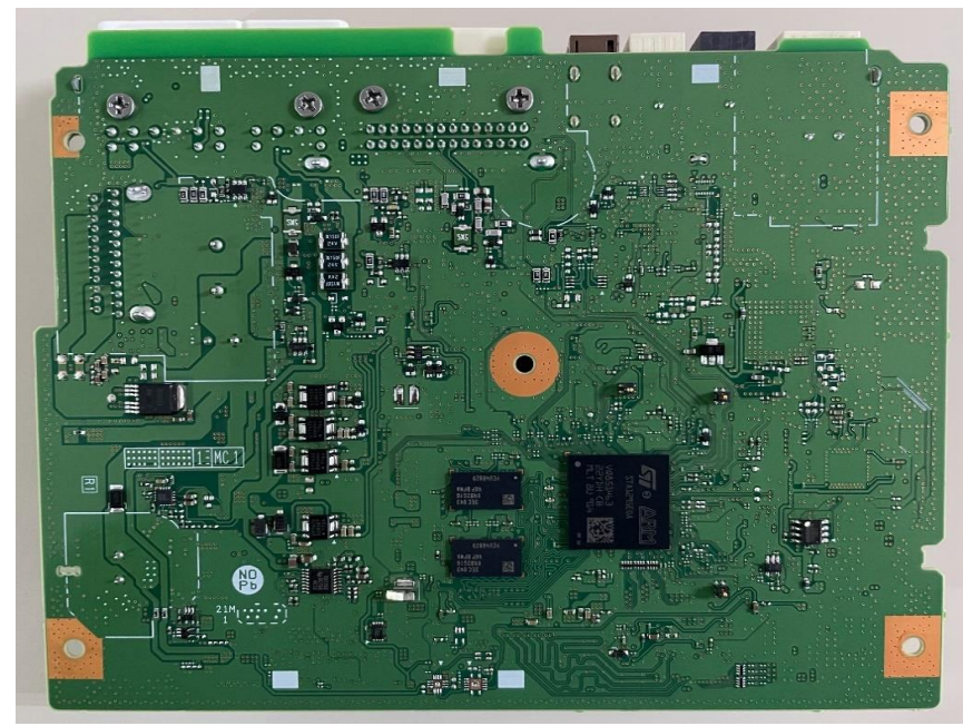
Solder side
