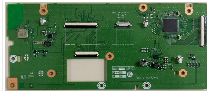
Solder side
