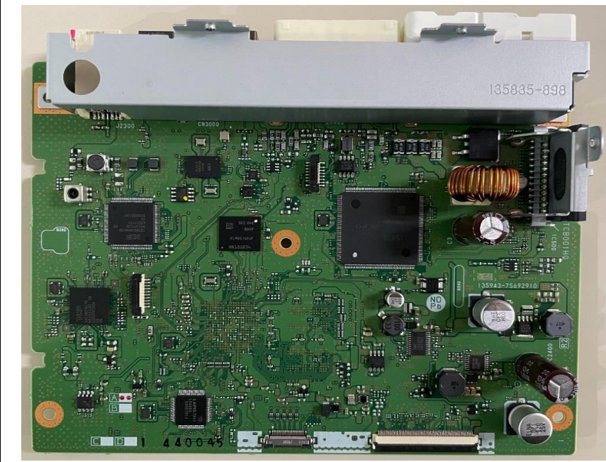
Component side
