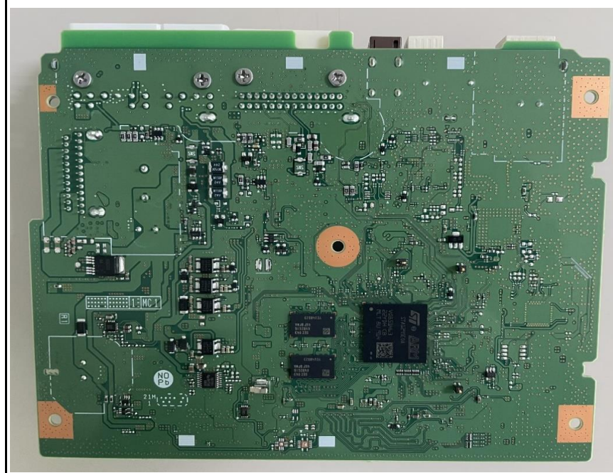
Solder side
