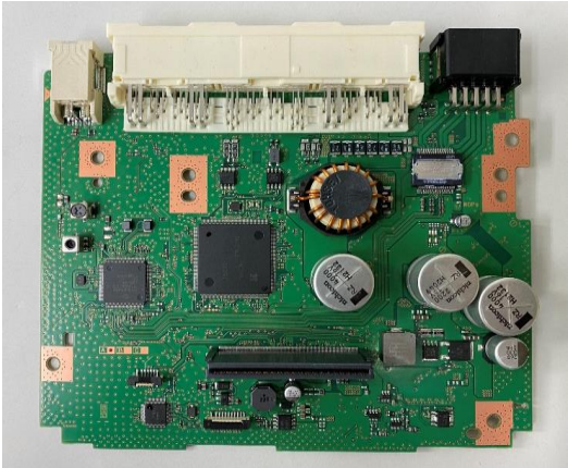
Component side (AUDIO)
