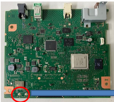
Main (CPU) Assy
