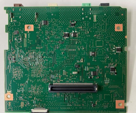
Solder side (AUDIO)
