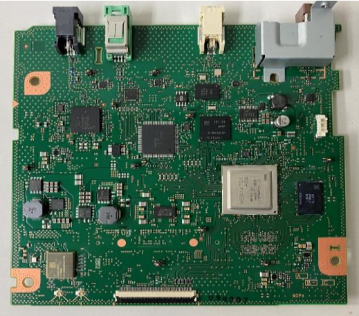
Component side (AUDIO)
