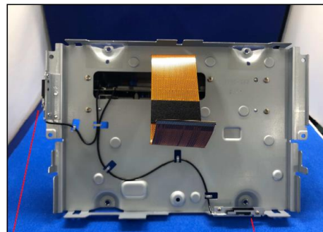
Antenna-Bluetooth
