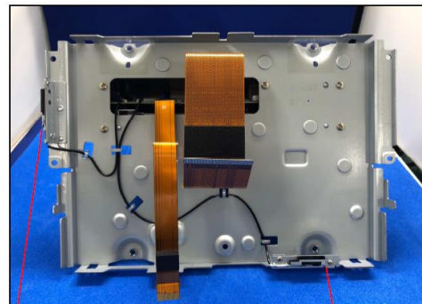
Antenna-Bluetooth
