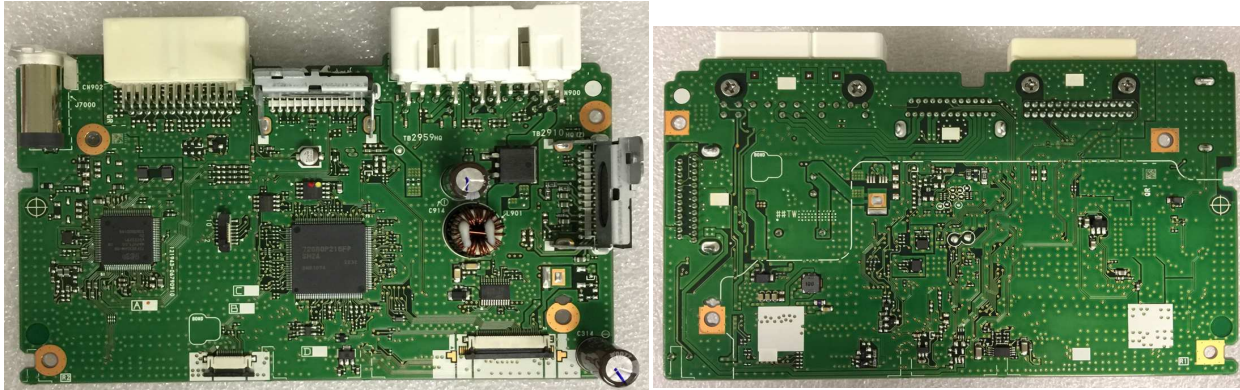
Main PCB
