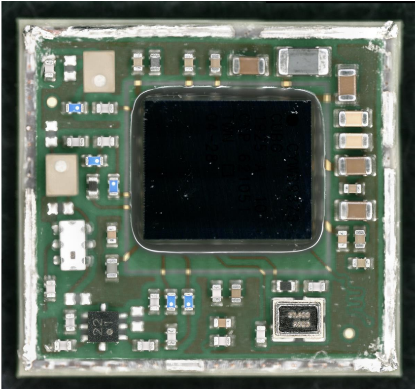
< Top View w/o Metal Case >
