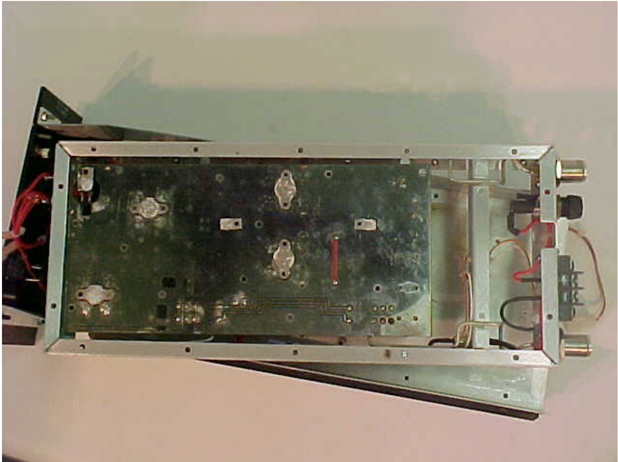
Photo 3 Detail View – Internal – Circuit Side of PCB
