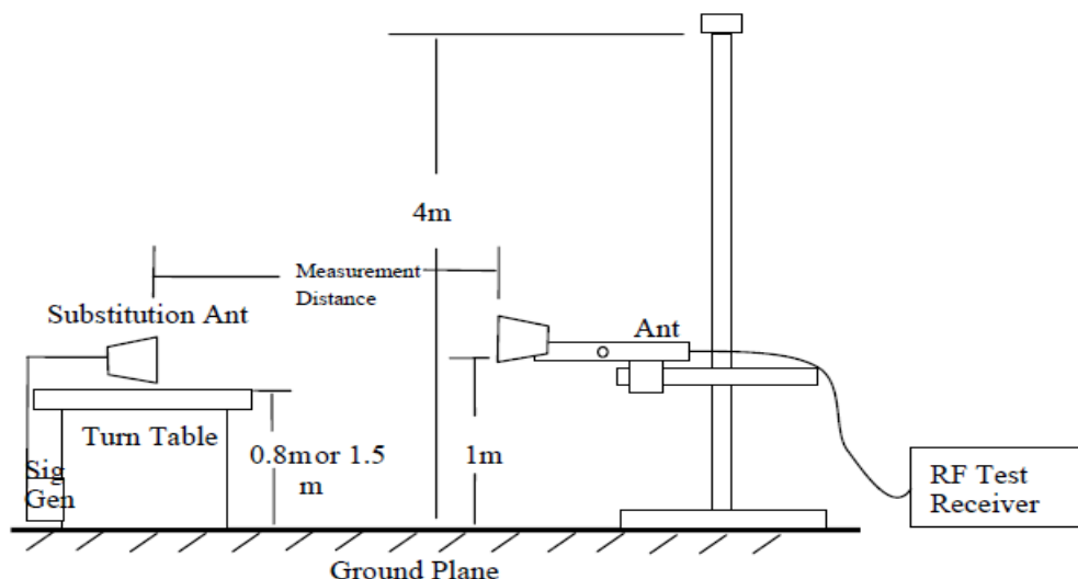
Figure 7—Substitution method set-up for radiated emission
