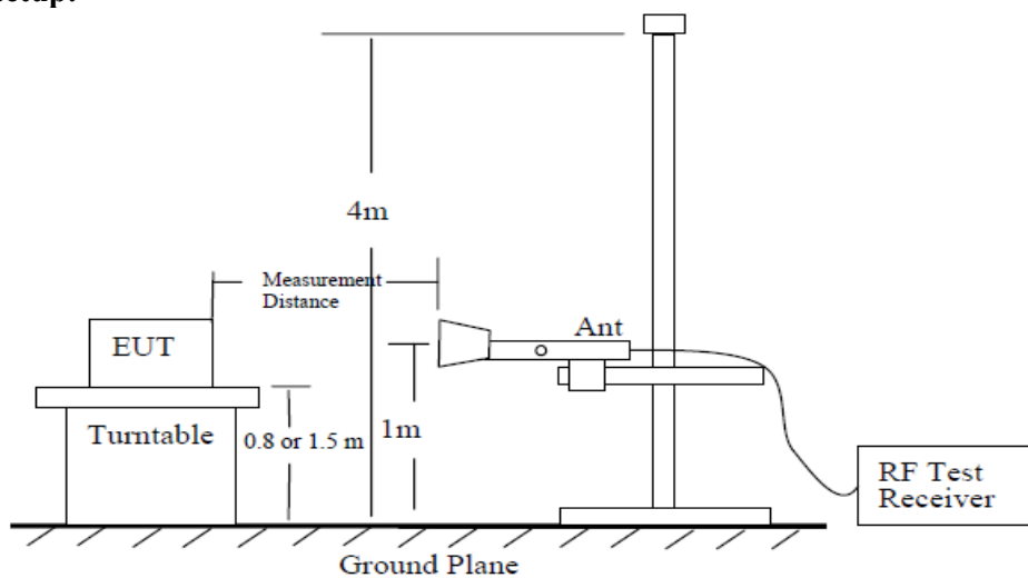
Figure 6—Test site-up for radiated ERP and/or EIRP measurements
