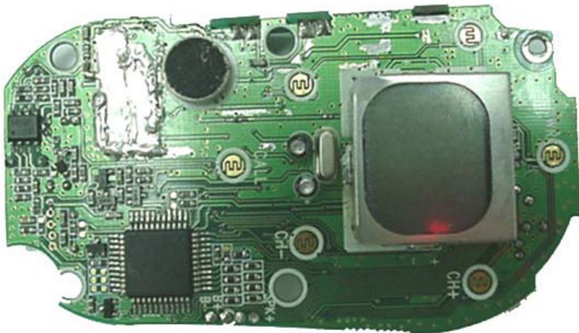
PCB Front w/ Shield
