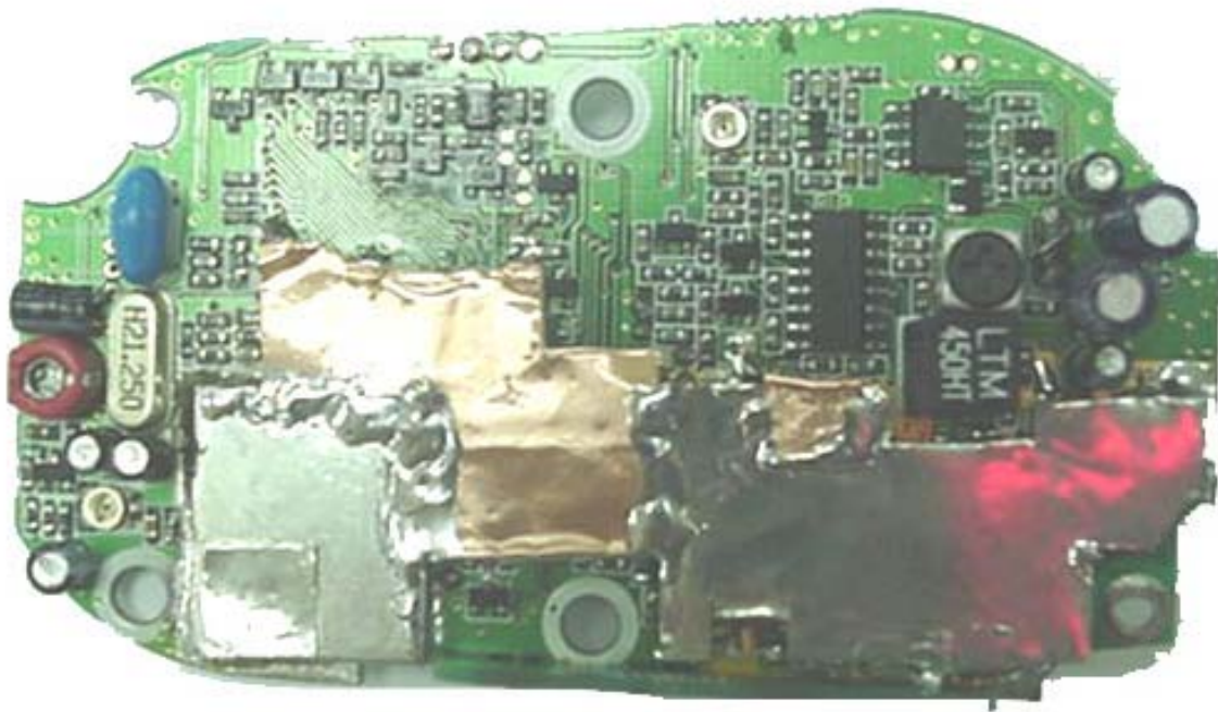
PCB Back w/Shield
