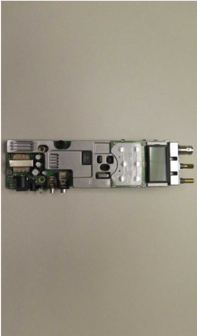
HH50_PCB_Front_With_Shield
