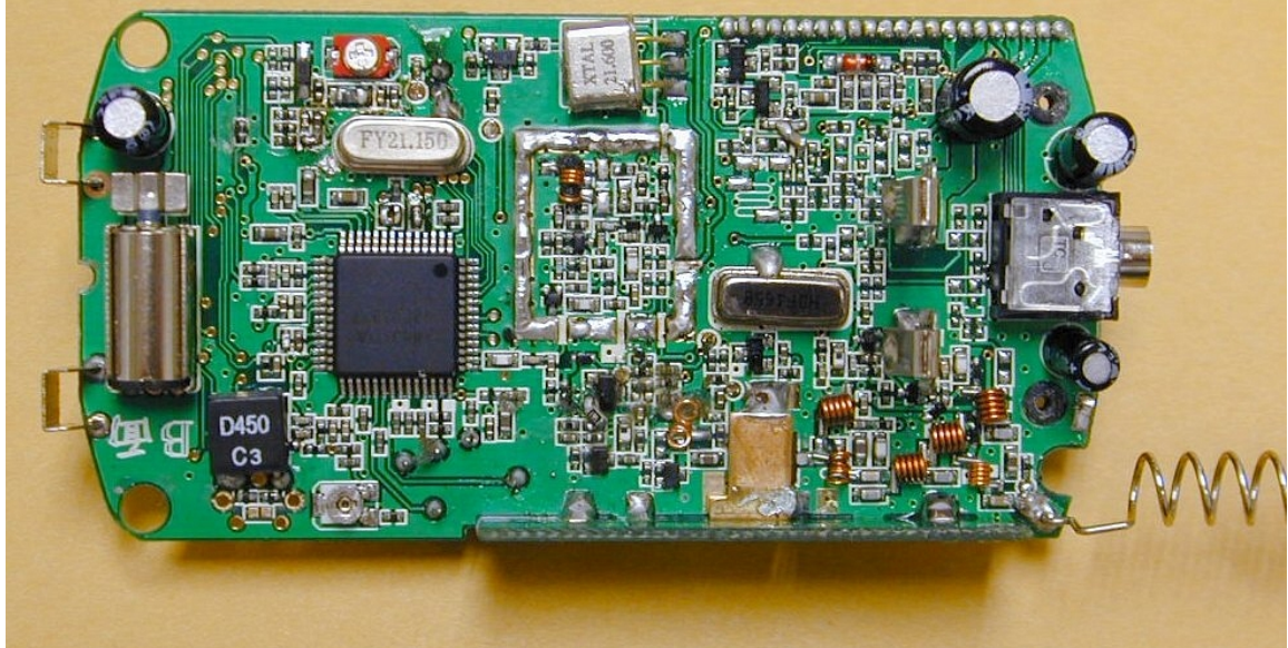
LI3900 Rear View / shield removed BBOLI3900
