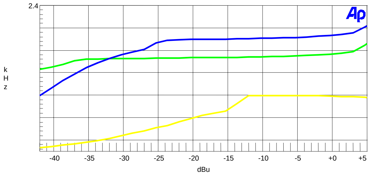
MODULATION LIMITING GRAPH 2.5KHz (Green), 1.0KHz (Blue), and 300Hz (Yellow)
