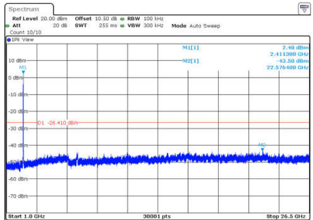
11G-Ant1-2412-1000~26500-PASS
