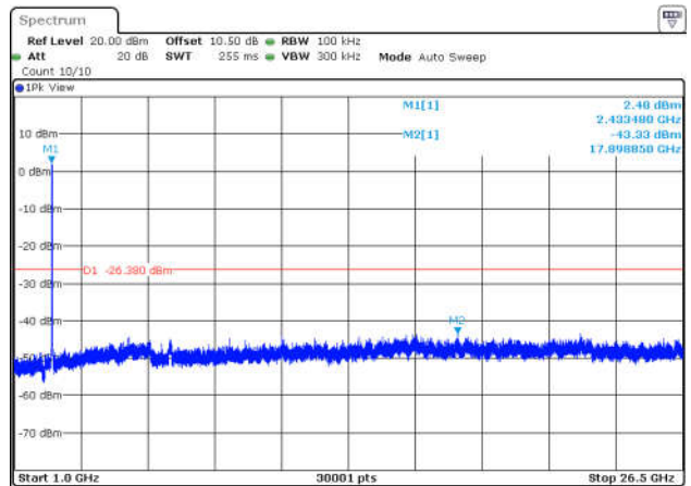
11N20SISO-Ant1-2437-1000~26500-PASS
