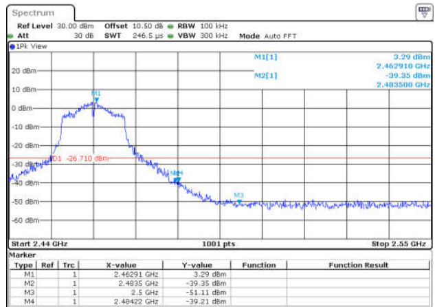
11N20SISO-Ant1-2462-PASS
