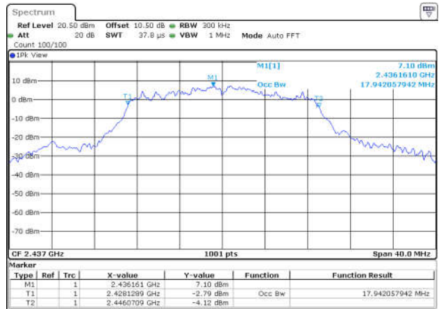
11N20SISO-Ant1-2437
