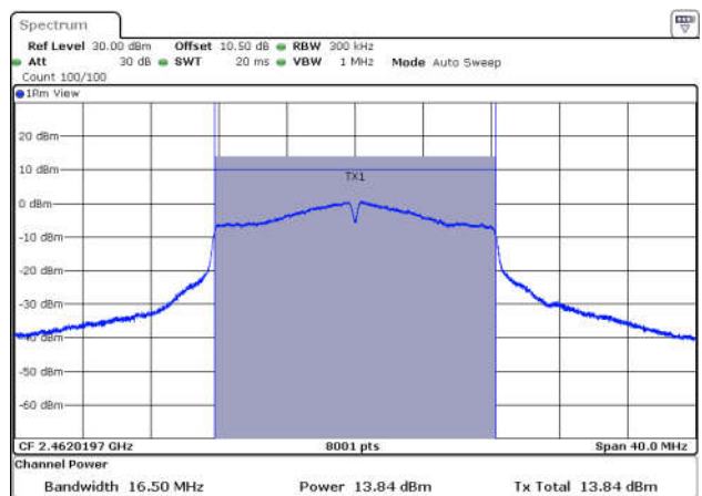
11G-Ant1-2462-PASS
