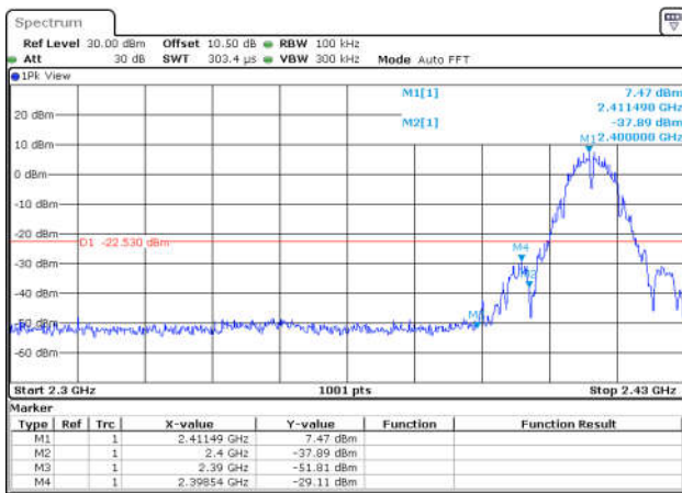
11G-Ant1-2412-PASS
