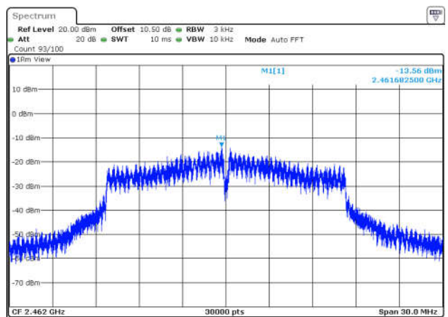
11G-Ant1-2462-PASS
