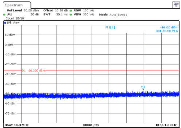
11G-Ant1-2462-0~Reference-PASS
