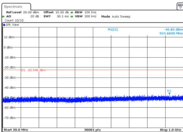
11B-Ant1-2437-30~1000-PASS
