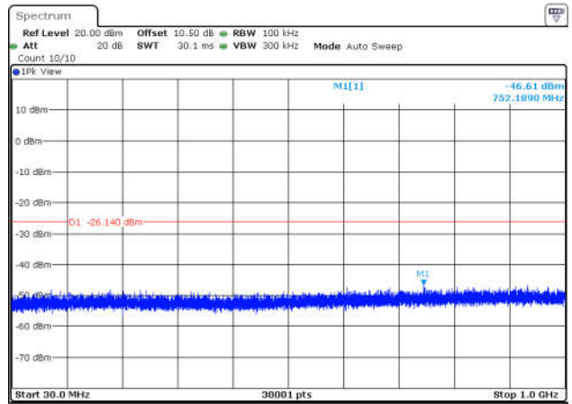
11N20SISO-Ant1-2437-0~Reference-PASS
