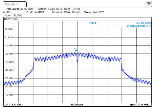
11N20SISO-Ant1-2437-PASS
