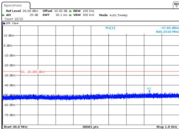
11N20SISO-Ant1-2437-30~1000-PASS
