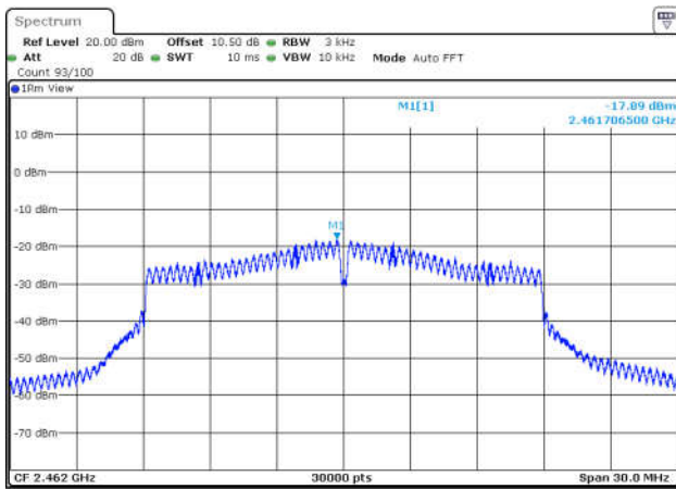
11N20SISO-Ant1-2462-PASS
