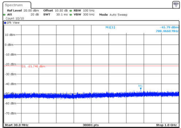
11G-Ant1-2412-0~Reference-PASS
