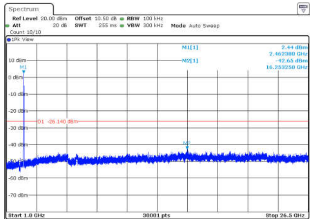
11G-Ant1-2462-1000~26500-PASS
