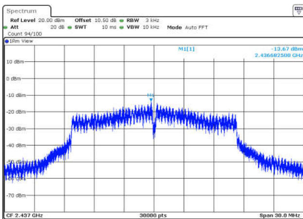
11G-Ant1-2437-PASS
