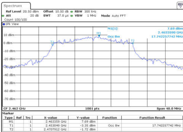
11N20SISO-Ant1-2462
