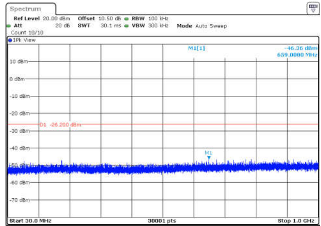
11N20SISO-Ant1-2462-30~1000-PASS
