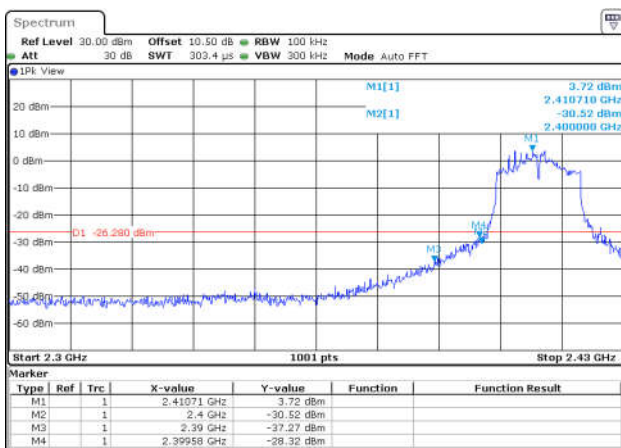
11N20SISO-Ant1-2412-PASS
