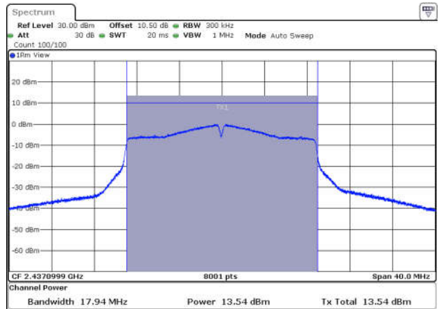
11N20SISO-Ant1-2437-PASS
