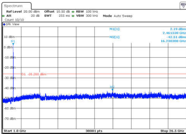
11N20SISO-Ant1-2462-1000~26500-PASS
