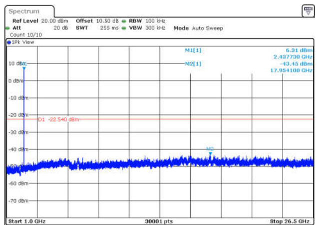
11B-Ant1-2437-1000~26500-PASS
